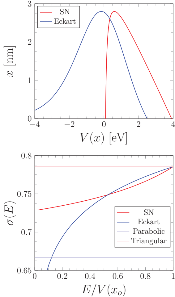
FIG. 4. (top) V(x) for the SN and Eckart barriers for parameters in the text. (bottom) the resulting scale factor \sigma(E) for each, where “Parabolic” and “Triangular” denote \sigma(E) = (2/3, \pi/4) for the inverted parabolic and the triangular FN barriers, respectively, for which both are constant.
