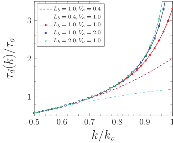
FIG. 2. The rectangular barrier dwell times \tau_d(k) (Eq. (10)) for various barrier widths L and heights V_o : larger values are associated with larger \theta ; smallest two values are dashed lines.
