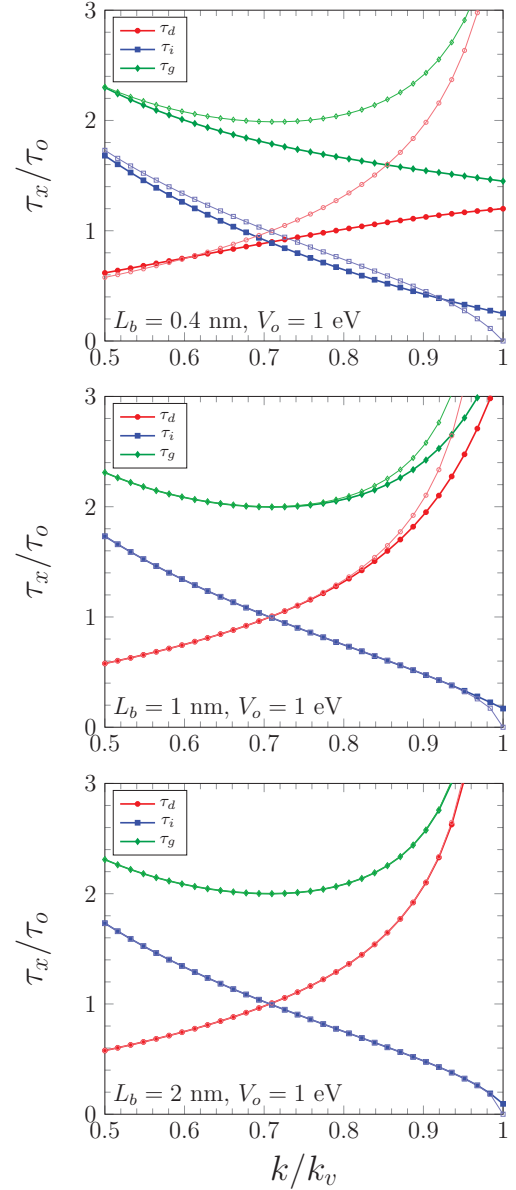
FIG. 1. Comparisons of rectangular barrier dwell time \tau_d (Eq. (8), red \bullet ), self-interference delay \tau_i (Eq. (10), blue \blacksquare ), and group delay \tau_g (Eq. (4), green \blacklozenge ) to the asymptotic large- \theta form (Eq. (11), thin light lines and \circ, \square, \diamond , respectively) for increasing L (top to bottom).
