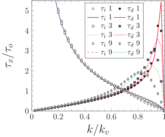
FIG. 3. Comparison of the exact ( \circ, \square, \diamond ) \tau_i(k) (Eq. (18)) and ( \bullet, \blacksquare, \blacklozenge ) \tau_d(k) (Eq. (23)) to the approximations for \tau_i/\tau_d (thick blue line / thick red line = 1, loosely dotted cyan / densely dotted purple = 3 and loosely dashed magenta / densely dashed green = 9) of Eq. (20) and Eq. (24), respectively. Legend is labeled by values of F [0.1 eV/nm]. V_o = 1.25 eV and \tau_o = 0.52657 fs. The subscript “ x ” on the \tau_x axis label denotes either d or i . \tau_g (not shown) would be the sum as per Eq. (4). The curves for \tau_i overlap so closely as to not be easily distinguishable
