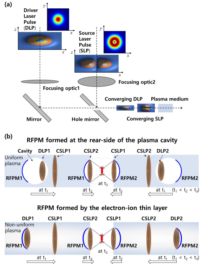
FIG. 4. (a) Schematic diagram for collinear coupling of driver and source laser pulses. (b) Formation of RFPMs and collision in vacuum of two source pulses reflected from respective RFPMs. CSLP: Converging source laser pulse.
