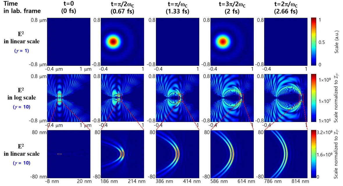
FIG. 3. The squared electric field distribution calculated from Eq. (43). The squared electric field distribution is expressed in the x (vertical)- z (horizontal) plane. In this plane, E''_{f,y} becomes zero since \phi = 0 . The electric field distributions in the first row are calculated under \gamma = 1 , i.e., the mirror is stationary. The field distribution agrees well with the characteristics obtained under the 4\pi -spherical focusing condition. The squared electric field distributions in the second and third rows are calculated under \gamma = 10 . The field distribution travels with a relativistic velocity of c\beta = c\sqrt{(\gamma^2 - 1)/\gamma^2} as shown in the third row, and the peak field strength is enhanced by a factor given by Eq. (46).
