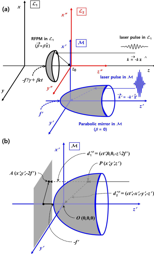
FIG. 2. Relativistic-flying parabolic mirror (RFPM) in the laboratory and the boost frames. As shown in (a), the shape of the parabolic mirror is elongated in the boost frame ( \mathcal{M} ) and the focal length becomes short by a factor of \gamma in the boost frame. The surface equation of the paraboloid in the boost frame can be obtained from the invariant property of event intervals, d'_{1\mu}d'_{1\mu} and d'_{2\mu}d'_{2\mu} , shown in (b).
