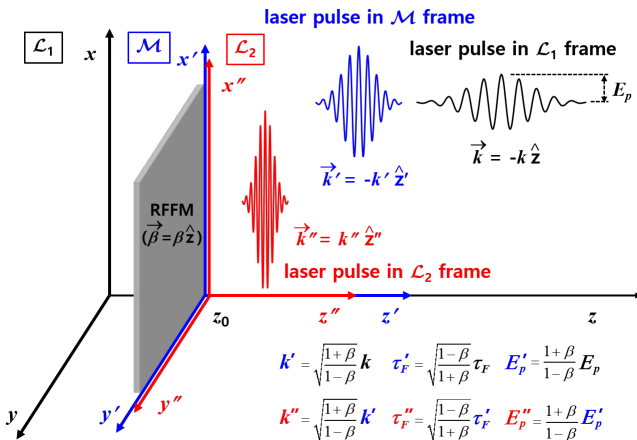
FIG. 1. Laser pulse reflected by a relativistic-flying flat mirror (RFFM). Due to the double Doppler effect, the wavevector, k , and the E-field strength, E_p , in time are enhanced by a total factor of (1+\beta)/(1-\beta) and the pulse duration, \tau_F , is shortened by a total factor of (1-\beta)/(1+\beta) .
