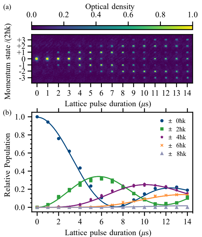
FIG. 3. An example of a Kapitza-Dirac measurement for a lattice of power P \sim 300 \text{ mW} at a wavelength of 881 nm. (a) Absorption images of the different BEC momentum states for varying lattice pulse duration, measured after a 40 ms levitated time-of-flight. (b) The relative atom number of the different diffracted momentum states are extracted from the images and fit using the method described in the text to give a trap depth of 4.96(2) \mu\text{K} .
