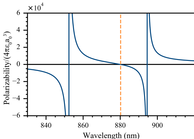
FIG. 1. Calculated scalar polarizability (blue solid line) of ground state Cs in the vicinity of the D_1 , 6S_{1/2} \rightarrow 6P_{1/2} , transition at 894.6 nm, and the D_2 , 6S_{1/2} \rightarrow 6P_{3/2} , transition at 852.3 nm. Between these two transitions the polarizability changes signs and passes through zero at the tune-out wavelength \lambda_0 \approx 880 nm as indicated by the dashed orange line.
