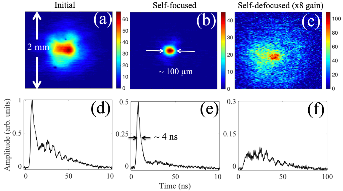
Figure 3: Beam profile measurements of (a) the initial beam, (b) the self-focused, and (c) self-defocused beam that correspond to temporal pulse profile measurements (d), (e), and (f), respectively. The pulse consisted of a 4 ns FWHM spike followed by a \sim 30 ns tail and only the initial spike was subjected to nonlinear focusing. Note that the vertical axes of (d), (e), and (f) are normalized to the peak amplitude of the initial laser pulse and that the absorption was \sim 50\% for (b), (e) and \sim 70\% for (c), (f). These measurements were performed using a peak intensity of 15 \text{ MW/cm}^2 and 100 torr of \text{CO}_2 with the laser wavelength tuned in the vicinity of the 4P(30) line.
