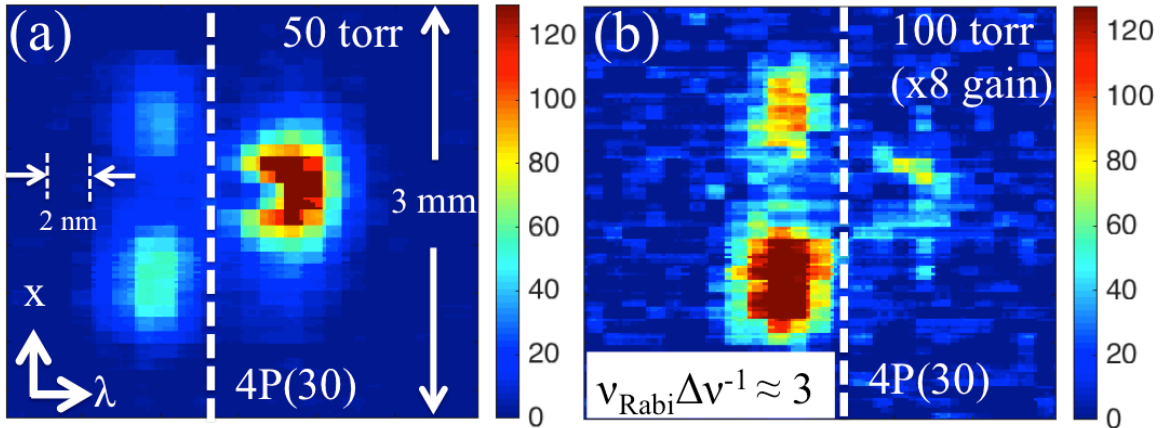
Figure 4: Frequency-resolved measurements of self-focusing and self-defocusing in the vicinity of the 4P(30) line of the 000 – 001 transition of \text{CO}_2 using (a) 50 torr and (b) 100 torr of \text{CO}_2 .
