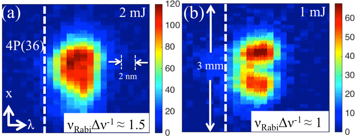
Figure 5: Frequency-resolved measurements of self-focusing and self-defocusing on the red side of the 4P(36) line of the 000 – 001 transition of CO 2 for (a) a 2 mJ pump and a (b) 1 mJ pump, showing an intensity-dependent sign reversal observed in 60 torr of CO 2 . These measurements were performed with approximately twice the cross-sectional area as those presented above to enable peak intensities of ~ 4 – 8 MW/cm 2 . Approximate normalized Rabi frequencies ( \nu_{\text{Rabi}} \Delta\nu^{-1} ) are indicated on each figure.
