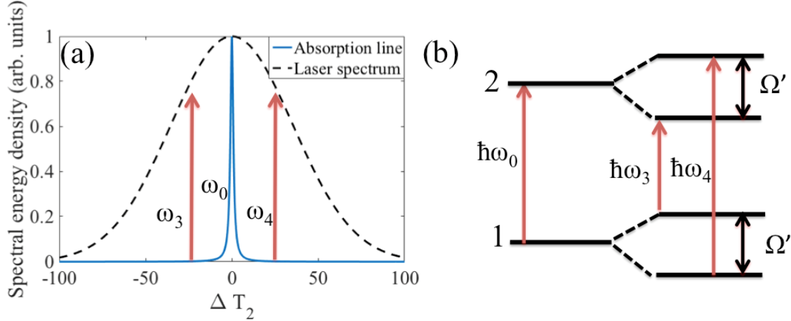
Figure 10: (a) Calculated Lorentzian absorption line of a single rovibrational line broadened to 100 torr with the approximate bandwidth of the Fe:ZnSe laser superimposed. (b) A depiction of the ac-Stark splitting of a two-level system with driven with a strong field, definitions for the frequencies are given in the text.
