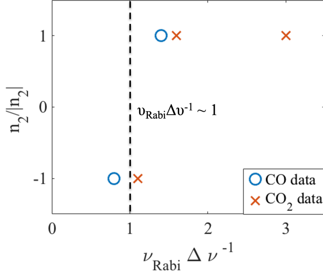
Figure 8: The sign of the nonlinearity inferred from CO and CO 2 data for frequencies below resonance plotted as a function of the estimated ratio between the effective Rabi frequency and the collisional linewidth. The dashed line indicates the point at which the Rabi frequency becomes equal to the collisional linewidth ( \nu_{\text{Rabi}} \Delta \nu^{-1} \sim 1 ).
