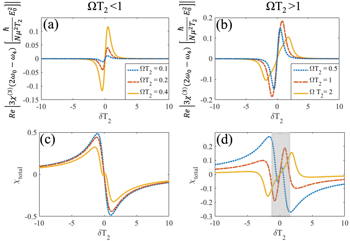
Figure 12: The real part of the third-order electric susceptibility for Rabi frequencies (a) less than the collisional linewidth and (b) greater than the collisional linewidth. The real part of the total electric susceptibility (sum of results presented in (a) and (b) with those presented in Fig. 11c and 11d) for Rabi frequencies (c) less than the collisional linewidth and (d) greater than the collisional linewidth.
