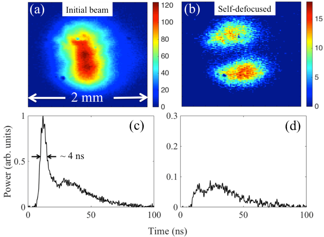
Figure 6: Beam profile measurements of (a) the initial beam and (b) self-defocused beam that correspond to temporal pulse profile measurements (c) and (d), respectively. Note that the pulse consisted of a 4 ns FWHM spike followed by a 30 ns tail and that only the initial spike was subjected to nonlinear focusing. The vertical axes of (c) and (d) are normalized to the peak amplitude of the initial laser pulse. These measurements were performed in the vicinity of the 4P(8) line of the v = 0 to v = 1 transition of CO for which the absorption was \sim 50\% .
