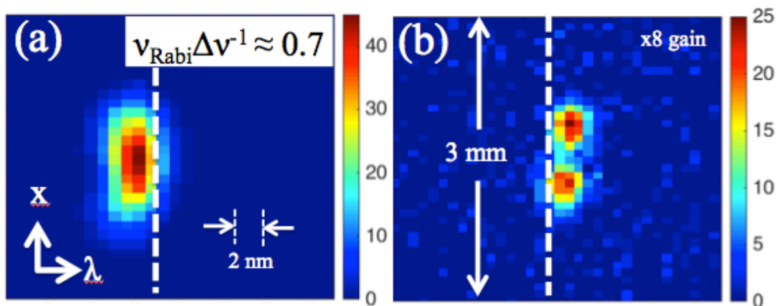
Figure 7: Frequency-resolved measurements in the vicinity of the 4P(8) line of the v = 0 to v = 1 transition of CO. (a) shows the unaffected beam profile and (b) shows strong self-defocusing on the red side of the rovibrational line. These measurements were obtained using 1 atm of 1:9 CO:He mix at a peak intensity of \sim 8 \text{ MW/cm}^2 .
