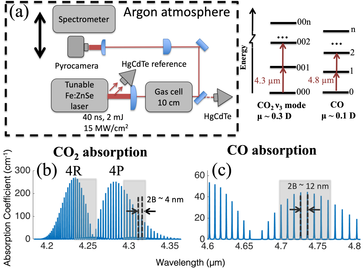
Figure 2: (a) The simplified experimental set-up used for time- and frequency-resolved measurements of resonant nonlinear refraction of 4 – 5 μm light in CO and CO 2 gas. (b) The absorption spectrum of 100 torr of CO 2 gas in the 4 μm wavelength range calculated using HITRAN [25]. (c) The absorption spectrum of 1 atm of CO gas calculated using HITRAN. The inset is a simplified energy level diagram of CO and CO 2 . Regions where spectral measurements were recorded are marked by the shaded rectangles on (b) and (c).
