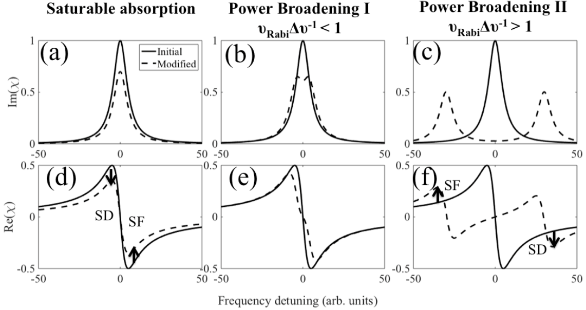
Figure 1: The imaginary (a, b, c) and real (d, e, f) parts of the electric susceptibility depicting saturable absorption (a, d) and power-broadening for cases with the Rabi frequency smaller (b, e) and larger (c, f) than the collisional line width.
