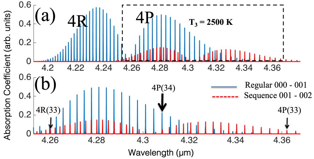
Figure 9: (a) Calculated absorption spectrum of CO 2 in the 4.3 μm wavelength region from HITRAN [25] and showing only the regular band transitions (000 – 001) and sequence band transitions (001 – 002). (b) Zoomed in the area of the black dashed rectangle in (a). The 4P(34) regular band transitions explicitly shares an energy level with the 4R(33) and 4P(33) sequence band transitions and are marked.
