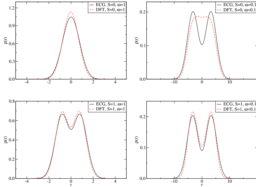
FIG. 1: Electron density of the two electron system. Top S=0 , bottom S=1 , left \omega = 1 , right \omega = 0.1 a.u. The solid curve is calculated by ECG; the dashed line is by DFT. The distance r is in a.u.
