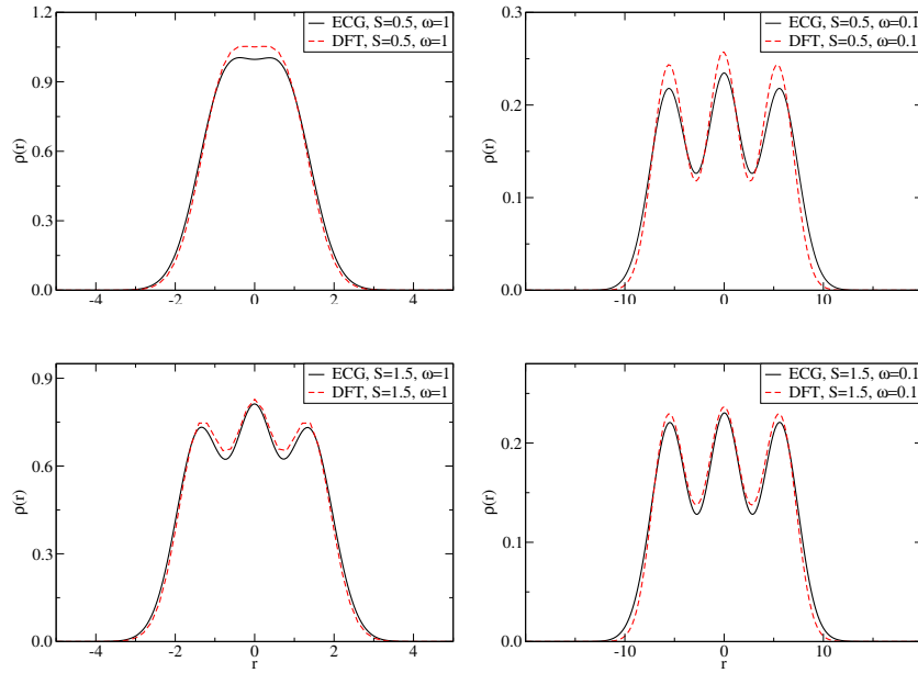
FIG. 2: Electron density of the three electron system. Top S=1/2 , bottom S=3/2 , left \omega = 1 a.u., right \omega = 0.1 a.u. The distance r is in a.u.
