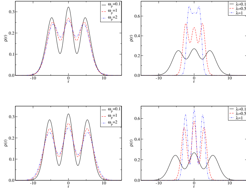
FIG. 8: Electron density of the three electron system coupled to light. Top S = 1/2 , bottom S = 3/2 ; left \lambda = 0.1 a.u., right \omega_n = 1 a.u. The distance r is in a.u.
