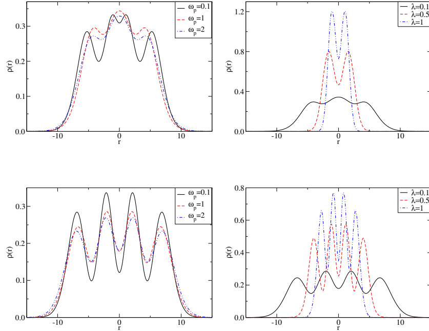
FIG. 9: Electron density of the four electron system coupled to light. Top S = 0 , bottom S = 2 ; left \lambda = 0.1 a.u., right \omega_p = 1 a.u. The distance r is in a.u.
