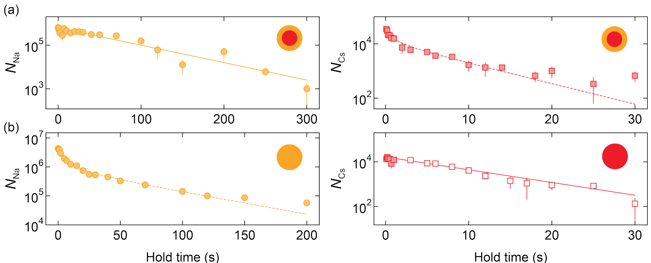
FIG. 7. Lifetimes of Na and Cs BECs at 23 G. (a) Decay of overlapping Na and Cs condensates. Orange circles (red squares) represent Na (Cs). (b) Decay of standalone Na and Cs condensates. Filled (empty) data points indicate the presence of a BEC (thermal cloud). Dashed lines represent fits that take into account one- and three-body decay, solid lines represent pure one-body decay.
