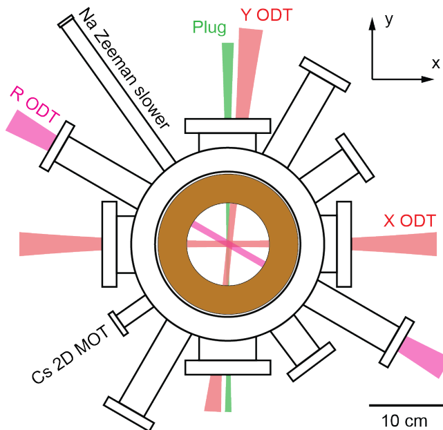
FIG. 2. Schematic of the experiment chamber, as viewed from top. Cold beams of Na (Cs) atoms enter the chamber from a Zeeman slower (2D MOT). Additional laser beams for absorption imaging (not shown) enter the chamber on the x -axis and the y -axis. The brown ring represents the magnetic field coils that can be switched between Helmholtz and anti-Helmholtz configurations.
