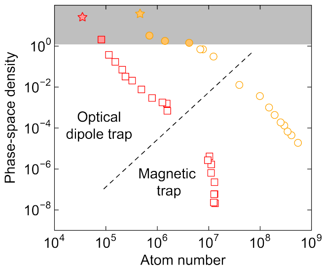
FIG. 5. Phase-space density versus atom number for Na (orange circles) and Cs (red squares) during the cooling process, measured for the working point at 23 G. Empty points indicate a thermal gas, filled points indicate that a condensate is present, and stars indicate the final atom number of the BEC for each species. Error bars are smaller than the size of the data points. The grey shaded region indicates phase-space densities for which condensation is expected.
