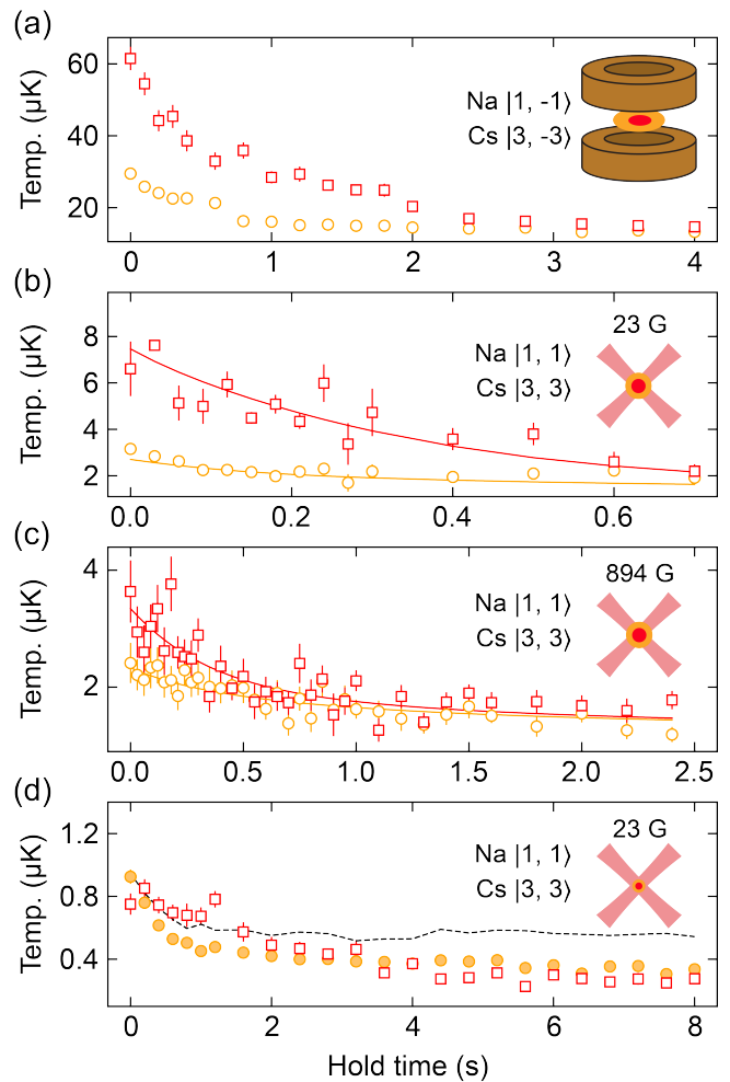
FIG. 6. Thermalization of Na and Cs. Na (Cs) data is shown as orange circles (red squares). Filled (empty) data points indicate the presence of a condensate (thermal cloud), error bars indicate the standard error of the mean of three experimental runs. Solid lines show the fit of the classical kinetic model. (a) Thermalization in the magnetic trap. (b) Thermalization between Na and Cs thermal clouds in the ODT at 23 G. (c) Thermalization between Na and Cs thermal clouds in the ODT at 894 G. (d) Thermalization between a Na BEC and a Cs thermal cloud. The dashed line indicates the critical temperature for a Na BEC, calculated from the atom numbers and trap parameters. During hold time, the Cs thermal cloud cools to about half of the Na critical temperature.
