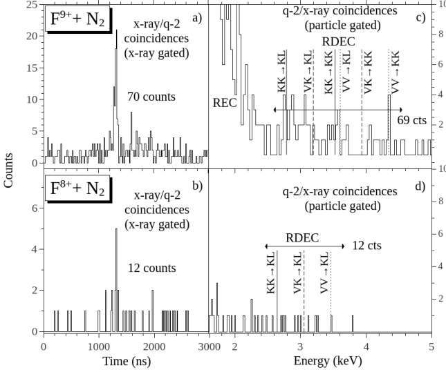
FIG. 5. Spectra obtained for 2.11 MeV/u (40 MeV) F^{9+} and F^{8+} + N_2 : Panels (a) and (b) are the x-ray-gated particle spectra for the doubly-charge changed projectiles sorted using the region labeled RDEC in Fig. 3a, while panels (c) and (d) are the particle-gated x-ray spectra corresponding to panels (a) and (b), respectively, i.e., the doubly-charge changed, q-2, outgoing state. The numbers shown on each graph are the totals for each spectrum after background subtraction, showing that the left and right panels agree with each other. The total number of incident particles was \sim 1.0 \times 10^{12} .
