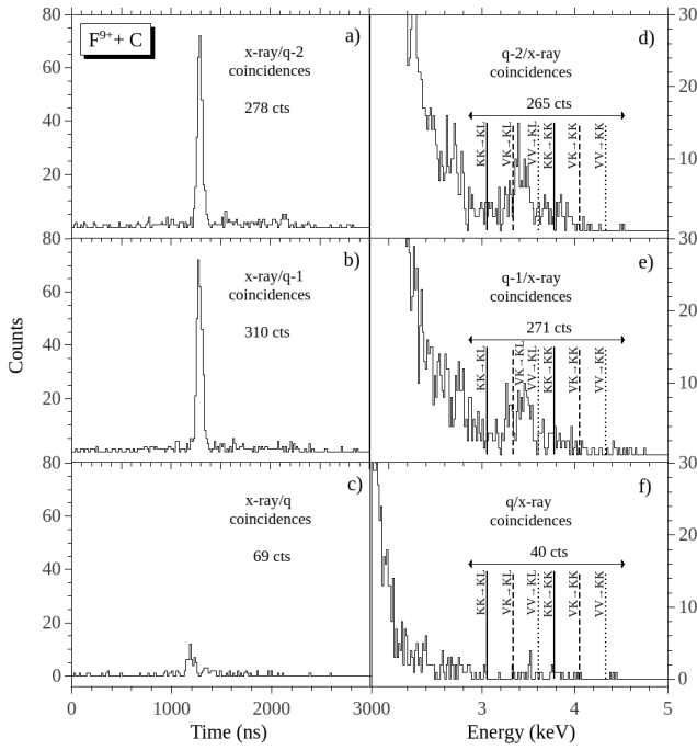
FIG. 7. Spectra obtained for 2.11 MeV/u (40 MeV) F^{9+} + C : Panels (a), (b), and (c) are the x-ray-gated particle spectra for the doubly-, singly-, and no charge changed projectiles sorted using the region labeled RDEC in Fig. 4a. Panels (d), (e), and (f) are the particle-gated x-ray spectra corresponding to panels (a), (b), and (c), respectively, i.e., doubly-, singly-, and no charge-changed outgoing states. The numbers on each graph are the totals for each spectrum after background subtraction, showing that the left and right panels agree with each other. The total number of incident particles was \sim 7.13 \times 10^9 .
