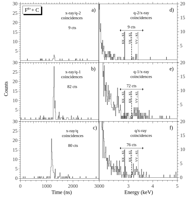
FIG. 8. Spectra obtained for 2.11 MeV/u (40 MeV) F^{8+} + C : Panels (a), (b), and (c) are the x-ray-gated particle spectra for the doubly-, singly-, and no charge changed projectiles sorted using a region similar to that labeled RDEC in Fig. 4a. Panels (d), (e), and (f) are the particle-gated x-ray spectra corresponding to panels (a), (b), and (c), respectively, i.e., doubly-, singly-, and no charge-changed outgoing states. The numbers shown on each graph are the totals for each spectrum after background subtraction, showing that the left and right panels agree with each other. The total number of incident particles was \sim 2.48 \times 10^9 .
