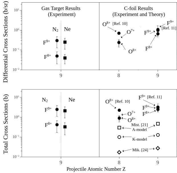
FIG. 12. Present results for F^{9+} and F^{8+} projectiles incident on gas targets ( N_2 and Ne), and for these same projectiles in addition to O^{8+} and O^{7+} incident on thin-foil C targets. The present gas results are in the left-most panels and the thin-foil results in the right-most panels. Theoretical calculations of Ref. [21] and Ref. [24] are also shown, which were only done for the foil targets.
