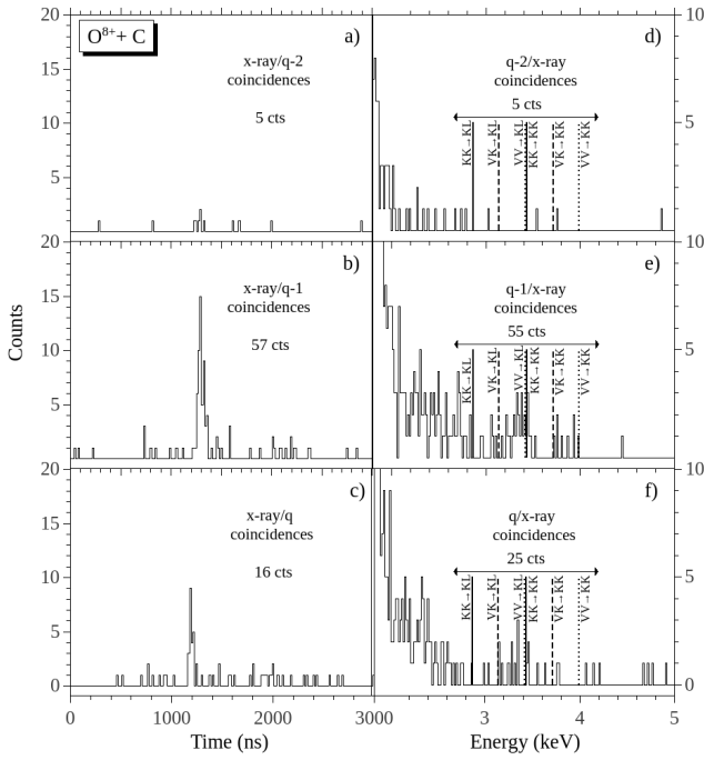
FIG. 9. Spectra obtained for 2.19 MeV/u (35 MeV) O^{8+} + C : Panels (a), (b), and (c) are the x-ray-gated particle spectra for the doubly-, singly-, and no charge changed projectiles sorted using a region similar to that labeled RDEC in Fig. 4a. Panels (d), (e), and (f) are the particle-gated x-ray spectra corresponding to panels (a), (b), and (c), respectively, i.e., doubly-, singly-, and no charge-changed outgoing states. The numbers shown on each graph are the totals for each spectrum after background subtraction, showing that the left and right panels agree with each other. The total number of incident particles was \sim 3.74 \times 10^9 .
