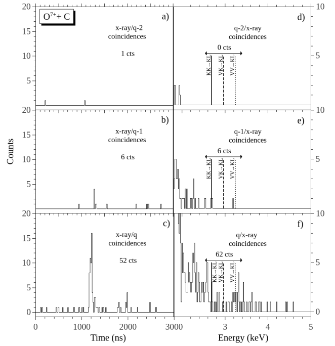
FIG. 10. Spectra obtained for 2.19 MeV/u (35 MeV) O^{7+} + C : Panels (a), (b), and (c) are the x-ray-gated particle spectra for the doubly-, singly-, and no charge changed projectiles sorted using a region similar to that labeled RDEC in Fig. 4a. Panels (d), (e), and (f) are the particle-gated x-ray spectra corresponding to panels (a), (b), and (c), respectively, i.e., doubly-, singly-, and no charge-changed outgoing states. The numbers shown on each graph are the totals for each spectrum after background subtraction, showing that the left and right panels agree with each other. The total number of incident particles was \sim 2.11 \times 10^9 .
