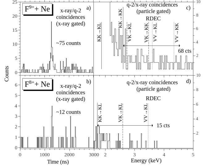
FIG. 6. Spectra obtained for 2.11 MeV/u (40 MeV) F^{9+} and F^{8+} + Ne . See Fig. 5 for the rest of the caption. Please note these spectra were obtained for an RDEC region similar to that indicated in Fig. 5, which was taken from the Ne spectrum corresponding to Fig. 3a.
