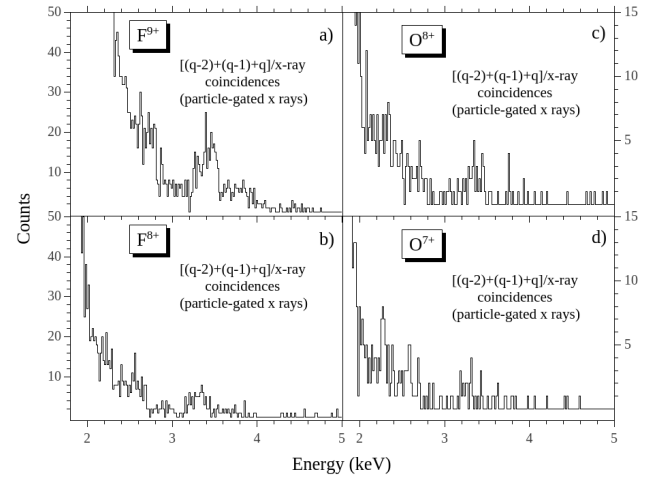
FIG. 11. Particle-gated x-ray spectra for the sum of q-2, q-1, and q outgoing charge states of incident 2.11 MeV/u (40 MeV) F^{9,8+} and 2.19 MeV/u (35 MeV) O^{8,7+} projectiles on C: Panels (a) and (b) are for F^{9+} and F^{8+} , respectively, and panels (c) and (d) for O^{8+} and O^{7+} , respectively. The total number of incident particles is given by the numbers in Figs. 7–10.
