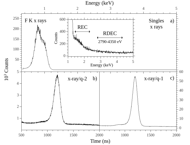
FIG. 3. Typical raw spectra obtained for the gas targets. Shown are the sums of collected (a) x-ray singles events, (b) x-ray/doubly charge-changed, q-2, and (c) x-ray/singly charged, q-1, coincidence events. The data are for 2.11 MeV/u (40 MeV) F^{9+} + N_2 . The RDEC range in eV is shown in the insert to panel (a).
