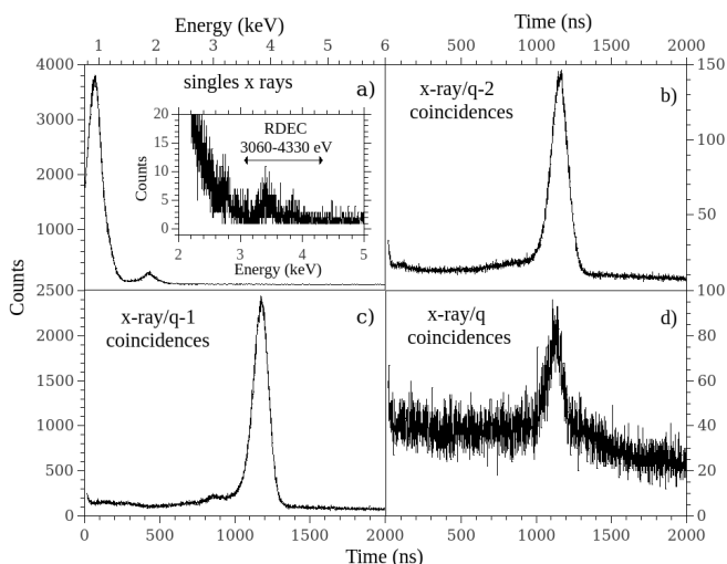
FIG. 4. Typical raw spectra obtained for the thin-foil C targets. Shown are the sums of collected (a) x-ray singles events, (b) x-ray/doubly charge-changed, q-2, (c) x-ray/singly charged, q-1, and (d) x-ray/no charge changed, q, coincidence events. The data are for 2.11 MeV/u (40 MeV) F^{9+} + C . The RDEC range in eV is shown in the insert to part (a).
