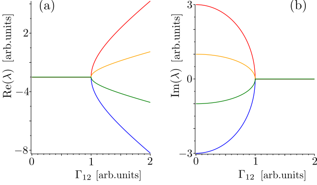
FIG. 3. (a) Real and (b) imaginary parts of the eigenvalues \lambda , according to Eq. (31), of the effective evolution matrix \hat{M}_C^{\text{eff}} , given in Eq. (30), for the third-order field moments. Its four eigenvalues coalesce at the EP in Eq. (22), thus indicating that the EP is of the fourth order. System parameters are set as \Gamma = 1 [arb. units] and \Delta = 1 [arb. units].
