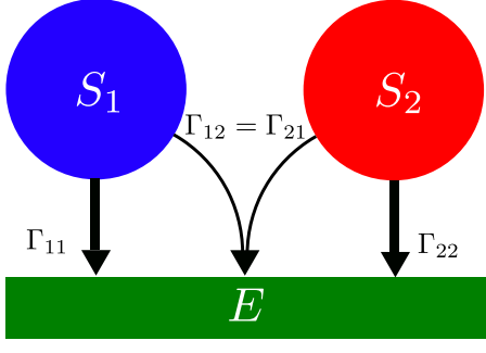
FIG. 2. Schematic representation of the model described by the Liouvillian superoperator \mathcal{L} in Eq. (17). S_1 and S_2 are two system modes, which dissipate to the environment E with rates \Gamma_{11} and \Gamma_{22} , respectively. The modes are also dissipatively coupled to the environment with the incoherent coupling strength \Gamma_{12} = \Gamma_{21} .
