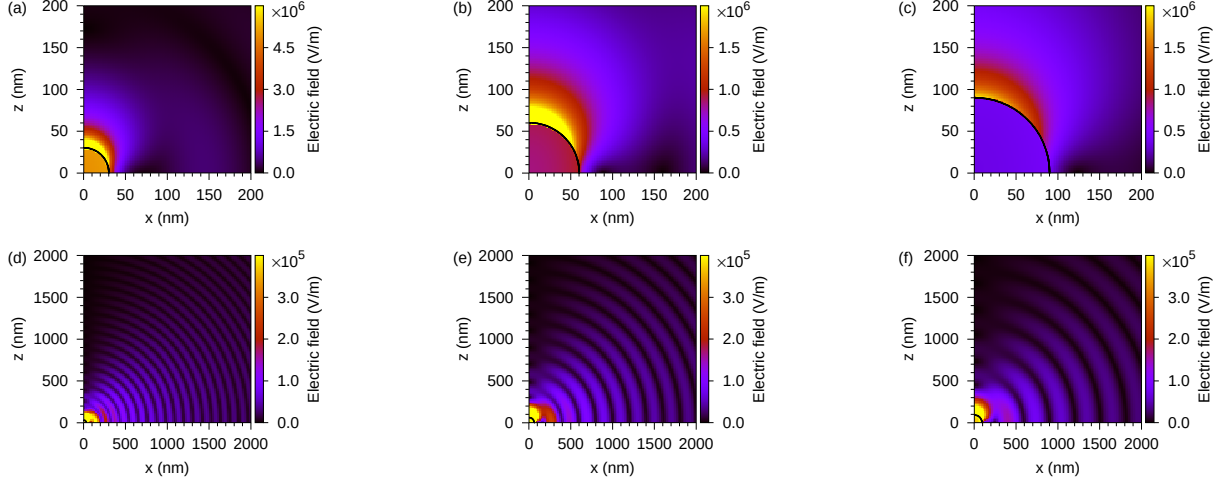
FIG. 5. Spatial distribution of electric field \mathbf{E}_\omega^{(slm)}(\mathbf{r}) per plasmon for Al nanosphere with the radius R for (a,d) 30 nm, (b,e) 60 nm, and (c,f) 90 nm. Absolute values of the electric fields are plotted. The angular frequency \omega is set at the resonance excitation energy of (a,d) 5.67 eV, (b,e) 3.08 eV, and (c,f) 2.04 eV. The permittivity of Al is taken from Ref. 54.
