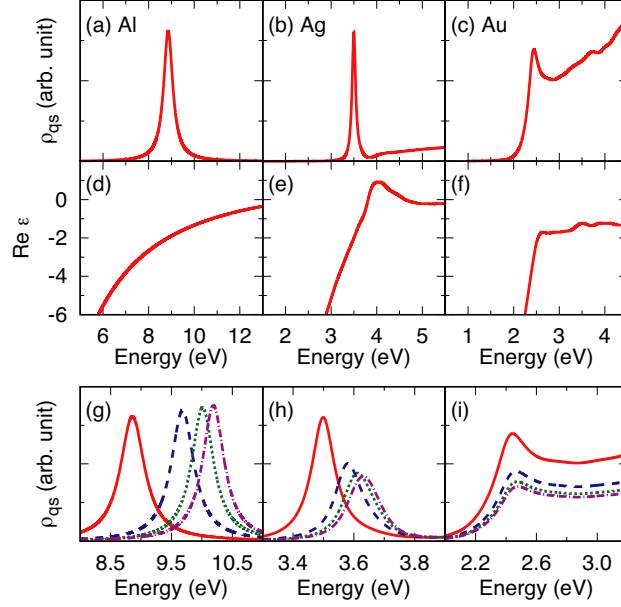
FIG. 1. Spectral function \rho_{\text{qs}}(\omega) for dipolar mode ( l = 1 ) for (a) Al, (b) Ag, and (c) Au nanosphere. Real part of permittivity of (d) Al taken from the experimental data reported in Ref. [54] and (e) Ag and (f) Au in Ref. [55] are displayed. Spectral function \rho_{\text{qs}}(\omega) for multipolar modes in (g) Al, (h) Ag, and (i) Au nanosphere are plotted. Red solid, blue dashed, green dotted, and purple dashed-dotted lines indicate l = 1, 2, 3, 4 modes, respectively.
