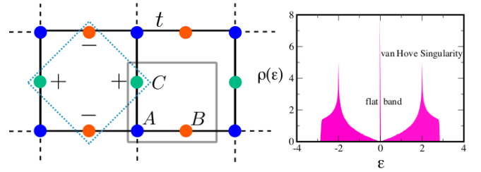
FIG. 1. (a) 2D Lieb lattice: The convention for the unit cell (grey square box) and the labelling of the three sublattices ( \alpha = A, B, C ) are shown. The links represent hoppings with magnitude t . A localized state of the flat band is the linear superposition of the four sites of the B and C sublattices inside the dashed square box. (b) The density of states \rho(\epsilon) of the noninteracting model.
