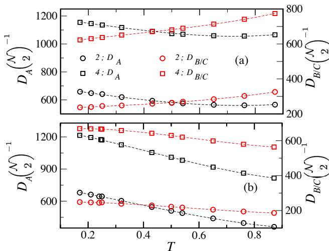
FIG. 6. a) : Sublattice-resolved and spatially-averaged double occupancy D_\alpha = \sum_i \langle \hat{n}_{i\alpha} \rangle vs. temperature T for U = 2 and \mathcal{N} = 2, 4 , in the presence of harmonic trapping. The chemical potential is fixed at \mu = 0 ( n = 3 at the trap center for \mathcal{N} = 2 , and n = 6 for \mathcal{N} = 4 ). b) : Same as in Fig. 4, with the only difference that the total particle number N is kept fixed, specifically N = 1.2 \times 10^4 ( 2.4 \times 10^4 ) for \mathcal{N} = 2 ( 4 ) components.
