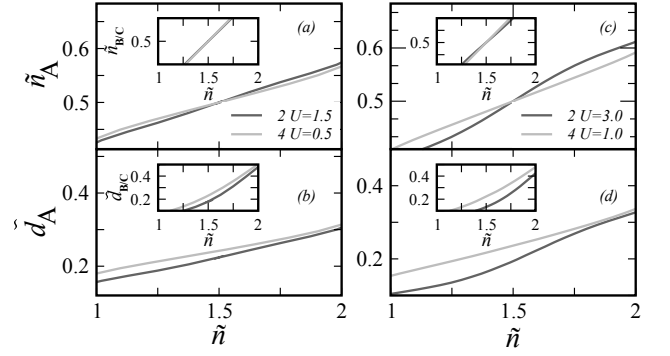
FIG. 5. Comparison of DMFT results between pairs of values (U, \mathcal{N}) satisfying the scaling relation (2). On the left (right) column the black lines are results for the sublattice-resolved occupation number \tilde{n}_{\alpha} = n_{\alpha}/\mathcal{N} and double occupancy \tilde{d}_{\alpha} = d_{\alpha}/\binom{\mathcal{N}}{2} for U = 1.5 ( U = 3 ) and \mathcal{N} = 2 , while the grey lines are results for U' = 0.5 ( U' = 1 ) and \mathcal{N}' = 4 . The occupation number and the double occupancy are normalized in such a way that the curves for different number of components would coincide if the mean-field approximation were exact.
