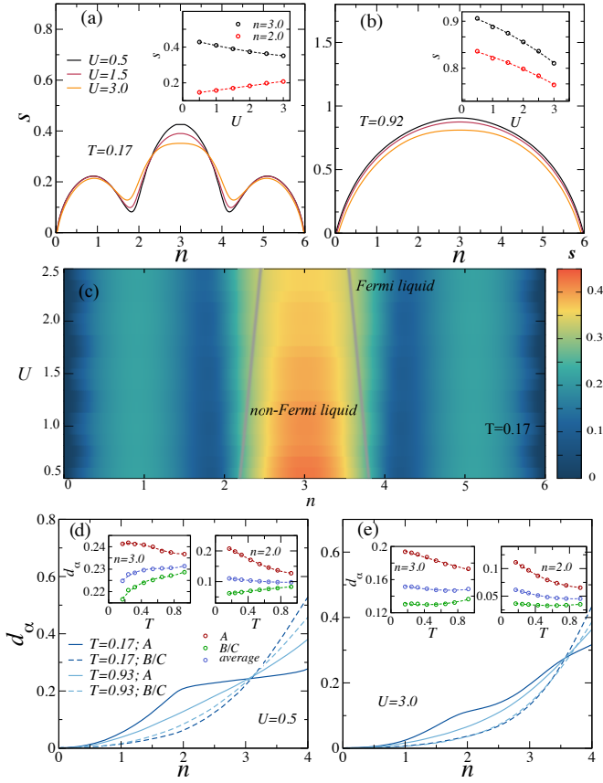
FIG. 2. a) Entropy per lattice site s as a function of total filling n = \sum_{\alpha} n_{\alpha} for \mathcal{N} = 2 component fermions at T = 0.17 and for three different values of the interaction strength. In the inset the entropy as a function of interaction strength is shown for filling n = 3 (half filling) and n = 2 (fully filled lowest band). b) Same as panel a , but at the different temperature T = 0.92 . c) Color map of the entropy in the n - U plane at the fixed temperature T = 0.17 . In the region between the grey lines, the entropy is a decreasing function of the interaction strength ( \partial U s < 0 ), a manifestation of the flat band-induced non-Fermi liquid behavior. d) Sublattice resolved double occupancy d_{\alpha} vs. filling n at U = 0.5 and for the same two values of temperature of panels a and b . In the insets the double occupancy (both sublattice-resolved and averaged) vs. temperature at fixed fillings n = 2, 3 is shown. e) Same as panel d , but for the different value of the interaction strength U = 3 .
