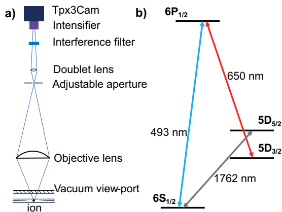
FIG. 1. Optical setup (a) and energy level diagram of ^{138}\text{Ba}^+ (b). Fluorescence from ions passing through the vacuum view-port is collected by the objective lens, through the adjustable aperture and further magnified by the doublet lens. An 493 nm interference filter is used to reduce the background. Finally, the 493 nm fluorescence is imaged onto the intensifier, which is connected to the Tpx3Cam camera. 493 nm and 650 nm lasers drive 6S_{1/2} - 6P_{1/2} and 5D_{3/2} - 6P_{1/2} cooling and repumping transitions, respectively. A 1762 nm laser couples the 5D_{5/2} and the 6S_{1/2} qubit states.
