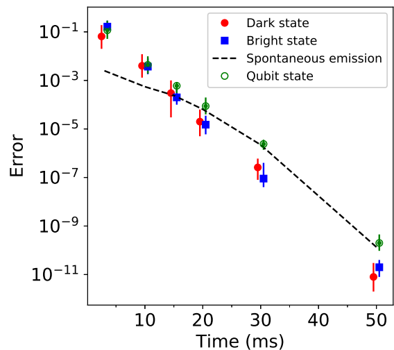
FIG. 5. Detection errors as a function of integration time. Solid squares (circles) represent the data for the bright (dark) state discrimination errors. The optimal threshold value n_{tr} is set by calculating where two Poisson curves corresponding to dark/bright ion states cross by extrapolating the curves, and rounding this value to an integer. The error bars are calculated by setting the threshold to n_{tr} \pm 1 . Horizontal offset of \pm 0.5 ms between dark and bright detection errors was introduced for clarity. The dashed line is the error due to the 5D_{5/2} spontaneous decay, calculated using Eq. 1. The combined error, shown in open circles, is the qubit state detection error that takes into account the bright/dark state discrimination error and the error due to spontaneous emission.
