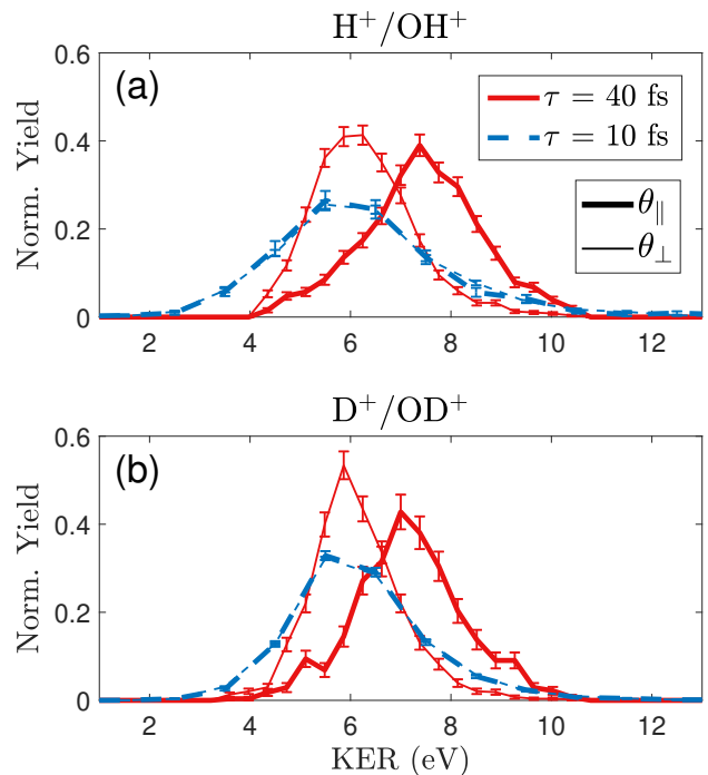
FIG. 5. The KER distribution for the two-body decay pathway of doubly-ionized water H_2O^{2+} \rightarrow H^+/OH^+ (a), and deuterated water, D_2O^{2+} \rightarrow D^+/OD^+ (b). In each case, the 40-fs data is plotted in solid red lines, and the 10-fs data is plotted in dashed blue lines. Both long and short-pulse data are further subdivided between dissociation aligned along the laser polarization axis: \theta_{\parallel} = 0^\circ \pm 30^\circ (thick lines) and dissociation aligned perpendicular to the laser polarization axis: \theta_{\perp} = 90^\circ \pm 30^\circ (thin lines). All distributions are independently normalized to integrate to one.
