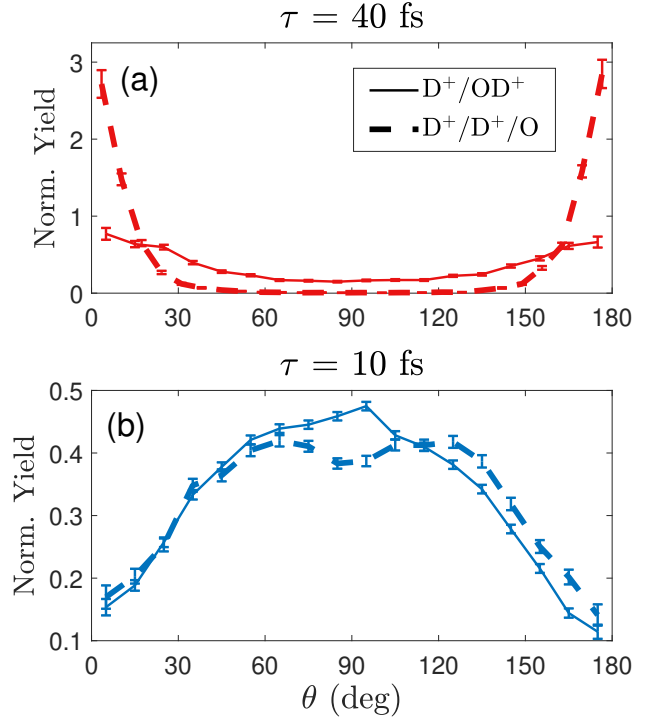
FIG. 4. The angular distribution of both two-body and three-body decay channels, as measured by the angle between the assumed \hat{y}_m molecular axis and the laser polarization, \hat{e}_{\text{laser}} . For both (a) the long-pulse data (in red) and (b) the short-pulse data (in blue), the two-body dissociation channel ( D^+/OD^+ ) is plotted as a thin solid line and the three-body dissociation channel ( D^+/D^+/O ) is plotted as a thick dashed line. For the two-body channel, \theta represents the angle between the dissociation axis and the laser polarization. For the three-body channel, \theta = \arccos(\hat{e}_{\text{laser}} \cdot \hat{y}_m) .
