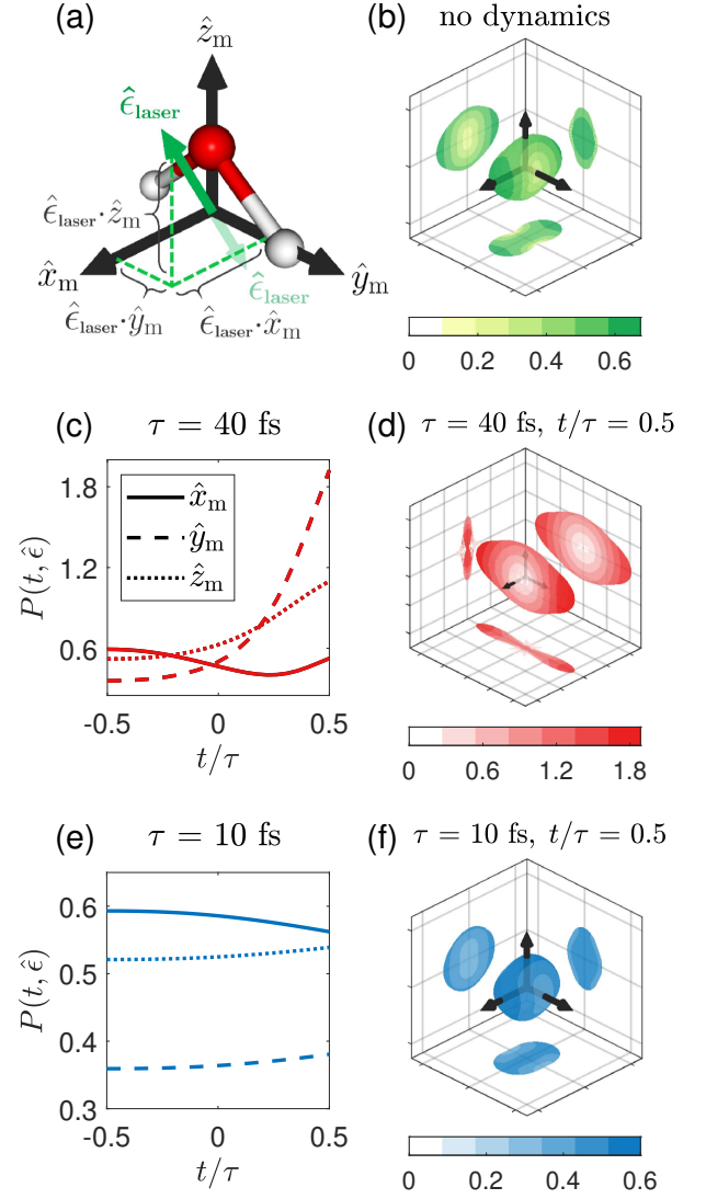
FIG. 3. (a) A schematic drawing of a definite laser polarization ( \hat{\epsilon}_{\text{laser}} ) plotted in the molecular frame with each of its projections along the molecular axes ( \hat{x}_m/\hat{y}_m/\hat{z}_m ) labeled. (b) The angle-dependent ionization yield for \text{D}_2\text{O}^+ (calculated via TD-RIS) represented as a 3D probability distribution of the laser polarization in the molecular frame as seen in (a). (c) The time-resolved alignment distribution of \text{D}_2\text{O}^+ as characterized by the value of the probability distribution, P(t, \hat{\epsilon}) , along each molecular axis: \hat{\epsilon} = \hat{x}_m (solid line), \hat{\epsilon} = \hat{y}_m (dashed line), and \hat{\epsilon} = \hat{z}_m (dotted line). Here, P(t, \hat{\epsilon}) was initiated with the distribution displayed in (b) at t/\tau = -0.5 where t/\tau = 0 is the time at which the molecule experiences peak field intensity, I_0 = 600 \text{ TW}/\text{cm}^2 , and \tau = 40 \text{ fs} is the ionizing pulse duration (FWHM). (d) The 3D alignment distribution of \text{D}_2\text{O}^+ after evolving in a strong field from t/\tau = -0.5 to t/\tau = 0.5 . As in (b), this distribution is represented by the 3D probability distribution of the laser polarization in the molecular frame as seen in (a). Note: the limits of all three axes are double those of (b) in order to capture the whole distribution. (e) The same as in (c) but for \tau = 10 \text{ fs} and I_0 = 400 \text{ TW}/\text{cm}^2 . (f) The same as in (d) but for \tau = 10 \text{ fs} and I_0 = 400 \text{ TW}/\text{cm}^2 . Note: the limits of all three axes are identical to those of (b).
