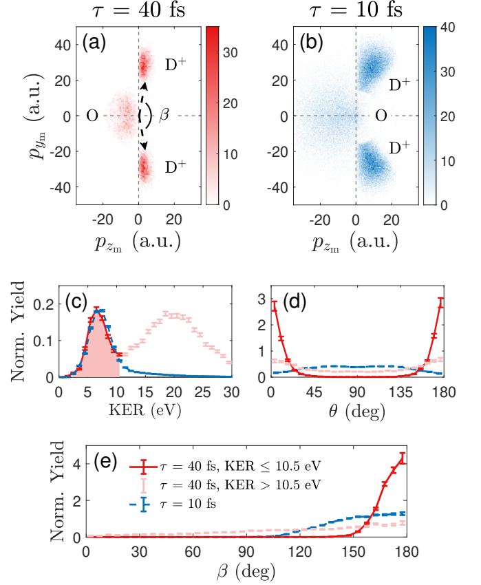
FIG. 2. (a) 2D momentum distributions of the fragments in the three-body breakup channel of the heavy water dication, \text{D}^+/\text{D}^+/\text{O} , following ionization by the 40-fs pulse. Here, the bisector between the vector momenta of the two \text{D}^+ ions is fixed to be along the horizontal such that the vector momentum of each ion can be decomposed into a component parallel to the bisector, p_{z_m} , and a component orthogonal to the bisector, p_{y_m} . (b) The same as in (a) but following ionization with the 10-fs pulse. (c) The KER distribution for the case of 40 fs (solid red line) and 10 fs (dashed blue line). Light red shading indicates the KER filter used to discriminate between the \text{D}^+/\text{D}^+/\text{O} dication channel (solid red line, shaded) and contamination from the higher-KER \text{D}^+/\text{D}^+/\text{O}^+ trication channel (light red markers, unshaded). Here, the 40-fs data has been resized to match the peak height of the 10-fs data. (d) The distribution in angle \theta = \arccos(\hat{e}_{\text{laser}} \cdot \hat{y}_m) , measured between the laser polarization axis ( \hat{e}_{\text{laser}} ) and the \hat{y}_m molecular axis. (e) The distribution in angle \beta = \arccos(\hat{p}_{\text{D}^+}^{(1)} \cdot \hat{p}_{\text{D}^+}^{(2)}) , measured between the two \text{D}^+ vector momenta ( \hat{p}_{\text{D}^+}^{(1)} and \hat{p}_{\text{D}^+}^{(2)} ), as drawn in panel (a).
