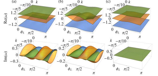
FIG. 4: (a) Band structure for 2\mathbb{Z} Chern insulator phase shown in Fig. 1(b). The band Chern numbers are -2, 4 and -2 from bottom to top. (b) Real gap closing at \delta\phi_L = 0.16\pi . (c) Band structure for \mathbb{Z} Chern insulator phase shown in Fig. 1(c). The band Chern numbers are -1, 2 and -1 from bottom to top.
