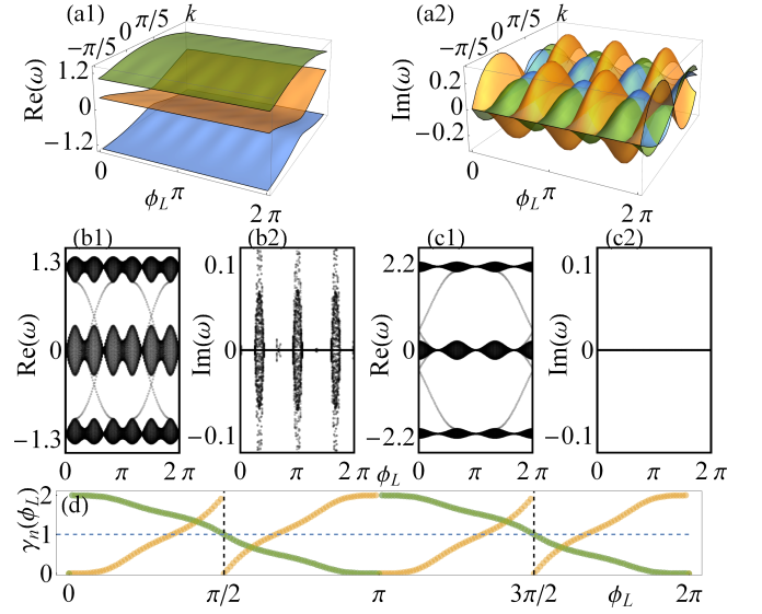
FIG. 1: 2\mathbb{Z} Chern insulator phase when \alpha = 1/3 . (a) 2D band structure in momentum-parameter space when \lambda = 1 . The Chern numbers for each band are -2 , 4 and -2 (from bottom to top). (b) Open-boundary spectra with respect to \phi_L for \lambda = 1 and N_L = 120 . (c) Similar to (b) but plotted with \delta\phi_L = \pi , which leads to a \mathbb{Z} Chern insulator with odd Chern number. (d) Normalized Berry phase \gamma_n(\phi_L) for bulk bands in (b). The dashed vertical lines indicate inversion-symmetric points.
