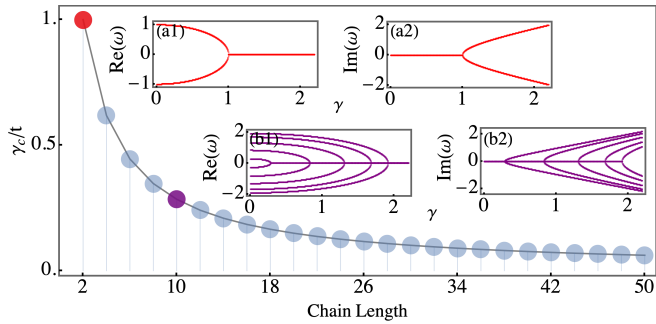
FIG. 6: Critical gain/loss rate for \mathcal{PT} breaking versus the length of the total chain in real space. The insets show how the spectrum changes for varying \gamma at given chain length 2 or 10.
