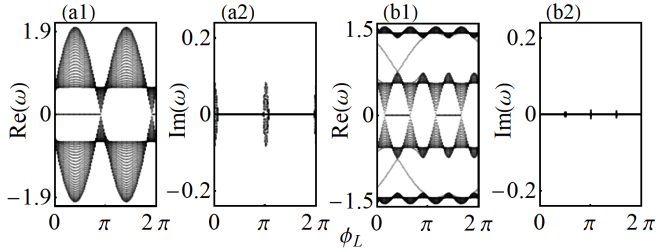
FIG. 5: (a) Open-boundary spectrum for varying \phi_L with \alpha = 1/2 , \lambda = 1 and \delta\phi_L = 0.2\pi . (b) Similar as panel (a) but plotted with \alpha = 1/4 .
