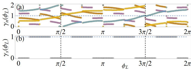
FIG. 7: (a) Berry phase \gamma_n(\phi_L) for the coexisting phase shown in Fig. 3(e). The dashed vertical lines indicate inversion-symmetric points and the numeric errors are more significant near gap closing points. (b) The \mathbb{Z}_2 invariant computed from panel (a).
