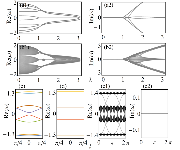
FIG. 3: (a) Open-boundary spectrum with respect to \lambda for \alpha = 1/5 , \phi_L = 0 and N_L = 10 . (b) Similar to (a) except N_L = 120 . (c) Bulk bands when \alpha = 1/8 , \lambda = 1 and \phi_L = 0.1\pi . (d) Flat bands at high-symmetry points \phi_L = \pi/4 . Other parameters are the same as panel (c). (e) Coexistence of chiral surface wave and zero modes at \alpha = 1/8 and \lambda = 1 .
