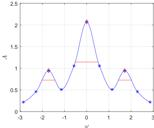
Figure 7. An example of how the linewidths are extracted. The blue stars correspond to experimental data. The blue line consists of a polynomial fit. The red diamonds mark the peaks and the red horizontal lines mark the widths of the peaks.
