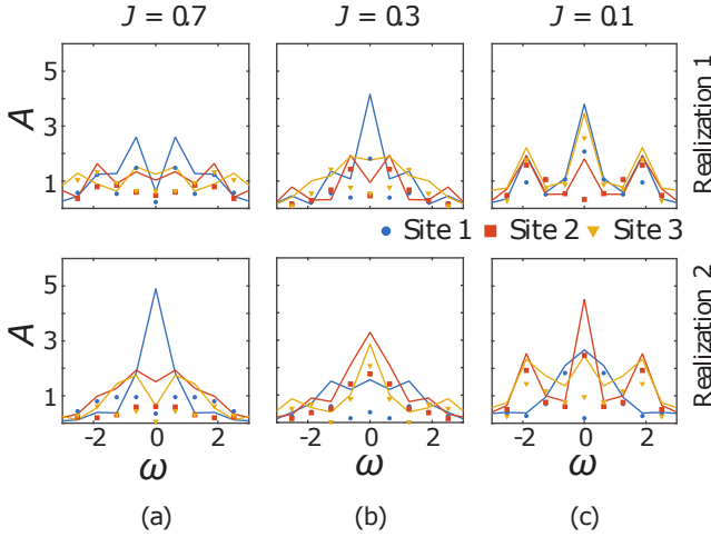
Figure 2. The spectrum of \hat{\sigma}_i^z at different values of J (with w = 1 ) for a 3 site system for two sample disorder realizations (top and bottom). Each panel show both simulation (curves) and experimental (symbols) results. The different colors are for the different sites. The lack of distinguishing characteristics between the spectra at different values of J for individual samples shows the necessity of averaging over several disorder realizations. With 2400 repetitions, the statistical error bars are smaller than the plot markers.
