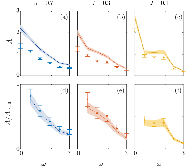
Figure 3. (a)-(c) The spectral function of \hat{\sigma}_i^z averaged over position and 24 disorder realizations for different values of J (with w = 1 ) for a 3-site system. Lines show simulation results and circles show experimental results. (d)-(f) The spectral function normalized by its value at \omega = 0 . At J = 0.7 , the spectral response increases as \omega decreases while at J = 0.1 , the spectrum is damped at low frequencies. The bands on the simulation curves and error bars on the experimental data signify the uncertainty after averaging over different disorder realizations. The points at \omega = 0 in the top row are discontinuous with the rest of the curves since they arise from the diagonal elements of the observable in the eigenstate basis which have qualitatively different behavior than the off-diagonal ones.
