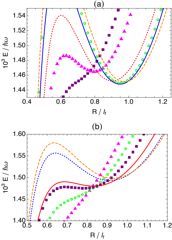
FIG. 5. (Color online) Adiabatic potentials with Q(R) included for a_s = -4.577 \times 10^{-4} l_t ; all are single-orbital results. (a) Results for N = 1220 . Orange dashed, blue solid, and red dotted curves are from \phi_{N_0, a_s} with N_0 = 1112.41, 1220 , and 1257.1 . Purple squares, magenta triangles, and green circles are from \phi_l^s with l = 0.38, 0.43 , and 0.64 . (b) Results for N = 1300 . Orange dashed, blue dotted, and red solid curves are from \phi_{N_0, a_s} with N_0 = 1149.27, 1203.19 , and 1257.12 . Magenta triangles, green circles, and purple squares are from \phi_l^s with l = 0.38, 0.43 , and 0.48 .
