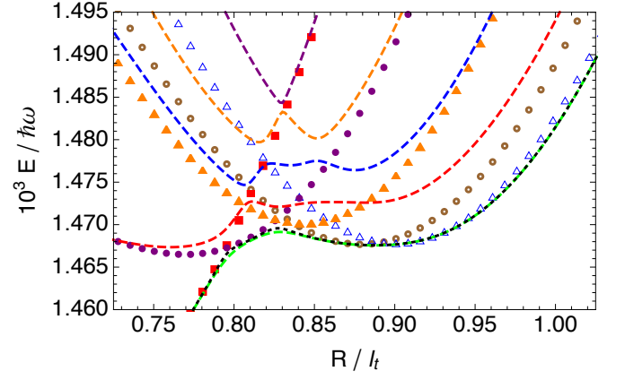
FIG. 6. (Color online) Adiabatic potentials for 1257 bosons with a_s = -4.577 \times 10^{-4} l_t . Open brown circles and open blue triangles are U with Q included from single \phi_{N_0, a_s} , with N_0 = 1257 and 1251.51 . Red squares, purple filled circles, and orange filled triangles are U with Q included from single \phi_l^s with l = 0.39, 0.44 , and 0.49 . The 5 dashed curves are the primitive generalized eigenvalues U , without Q , from coupling the above 5 orbitals; no eigenstate of Q is removed. The colors green, red, blue, orange, and purple denote the 5 eigenvalues in increasing order. The dotted black curve includes Q for the lowest eigenvalue.
