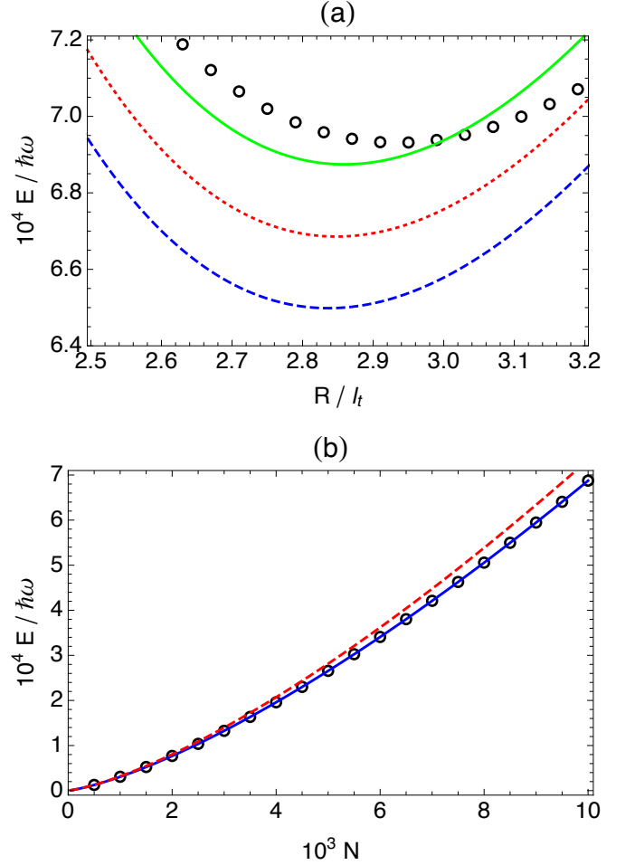
FIG. 1. (Color online) (a) Adiabatic potentials with Q included, U(R) - \frac{Q(R)}{2N} , for a_s = 0.01 l_t and various N . The blue dashed, red dotted, and green solid curves come from single \phi^{GP} for N = 9600, 9800 , and 10000 , respectively. The black circles are the K-Harmonic U for N = 9600 . (b) Here a_s = 0.01 l_t with varying N . The black circles are the mean-field energy E_0(N) . The blue solid and red dashed curves are the minima of U - \frac{Q}{2N} from \phi^{GP} and from the K-Harmonic approximation, respectively.
