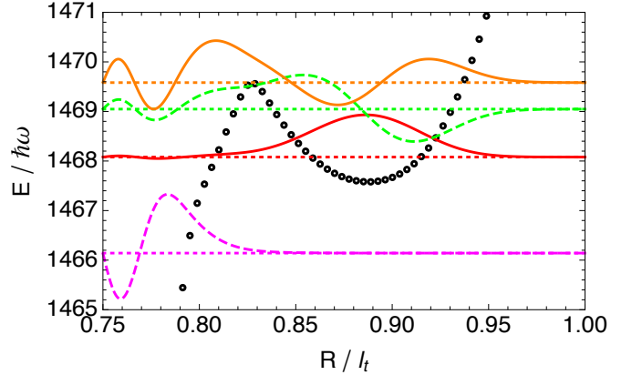
FIG. 7. (Color online) Hyperradial eigenstates F(R) for N = 1257 and a_s = -4.577 \times 10^{-4} l_t . The potential, represented by black circles here, is the dotted black curve of Fig. 6. Boundary condition F(R_c) = 0 at R_c = 0.75 l_t is chosen. Dotted lines denote the eigenenergies; solid and dashed curves are the corresponding wavefunctions F(R) (scaled arbitrarily). Magenta denotes a collapsed state outside the minimum well; red denotes a metastable state, while green and orange denote rapidly decaying states.
