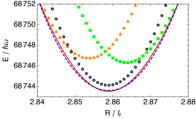
FIG. 4. (Color online) Adiabatic potentials with Q(R) included for 10^4 bosons with a_s = 10^{-2} l_t . The orange triangles, black circles, and green squares are single \phi_{N_0, a_s} results with N_0 = 9600.04, 10^4 , and 10399.96 . The red solid curve is the lowest primitive eigenvalue from coupling 3 orbitals with N_0 = 9800.02, 10^4 , and 10199.98 , with no eigenstate of \underline{Q} removed. The blue dashed curve is the lowest reduced eigenvalue from coupling 5 orbitals with N_0 = 9600.04, 9800.02, \dots, 10399.96 , with 1 eigenstate of \underline{Q} removed.
