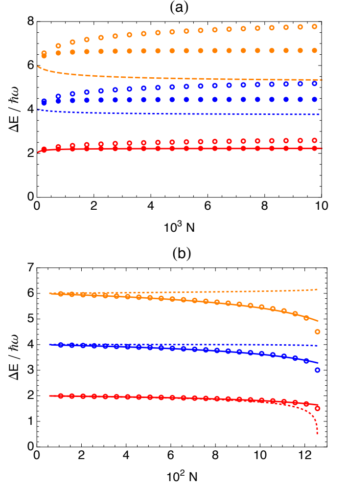
FIG. 3. (Color online) The first 3 excitation energies E_i - E_0 with varying N . Red, blue, and orange denote the 1st, 2nd, and 3rd excited states. (a) Results for a_s = 0.01 l_t . Solid, dotted, and dashed curves are the Bogoliubov mode frequencies, while solid circles are from the K-Harmonic potentials. Open circles are the results of single- \phi^{GP} calculations. (b) Results for a_s = -4.577 \times 10^{-4} l_t . Dotted curves are the Bogoliubov predictions, while solid curves are from the K-Harmonic U . Circles are from single- \phi^{GP} calculations.
