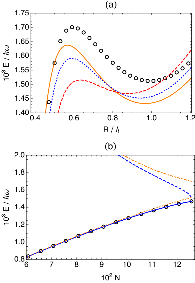
FIG. 2. (Color online) (a) Adiabatic potential with Q included for a_s = -4.577 \times 10^{-4} l_t and various N . The orange solid, blue dotted, and red dashed curves come from single \phi^{GP} for N = 1197, 1227 , and 1257 , respectively. The black circles are the K-Harmonic potential U for N = 1257 . (b) Here a_s = -4.577 \times 10^{-4} l_t with varying N . The black circles are the mean-field E_0(N) . The blue solid and dashed curves are the minima and maxima, respectively, of U - \frac{Q}{2N} from \phi^{GP} . The orange dotted and dash-dotted curves are the minima and maxima, respectively, of the K-Harmonic U .
