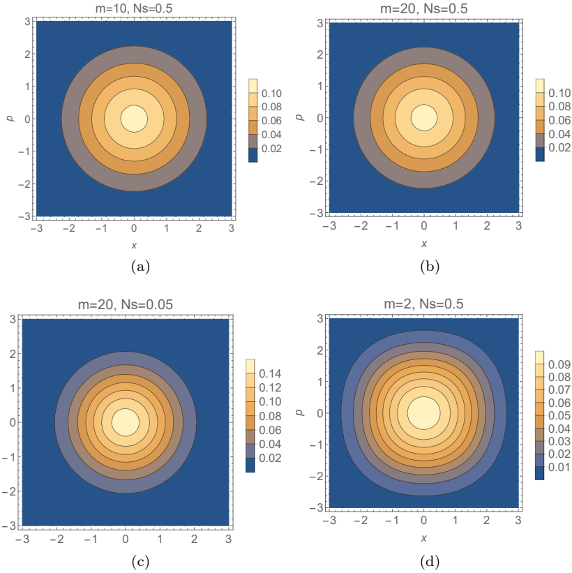
FIG. 1. (a) M = 10, N_s = 0.5 (b) M = 20, N_s = 0.5 (c) M = 20, N_s = 0.05 (d) M = 2, N_s = 0.5
