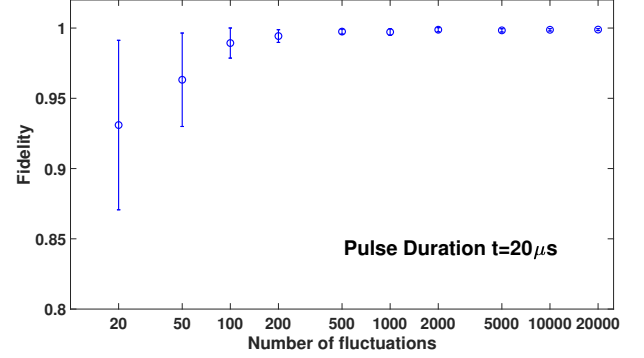
FIG. 5. Fidelity of the geometric gauge transformation versus number of fluctuations. Each point is calculated by averaging five runs with the same number of fluctuations for 26 different initial states, the errorbars is the standard deviation of all the fidelities calculated from the 130 runs for the same number of fluctuations. The ideal SU(2) transformation operator is U_c^{ideal} = (\mathbb{1} - i\sigma_y)/\sqrt{2} . The standard deviation of random Gaussian noises for bias magnetic field and laser powers are 5% of their amplitudes. For relative phase, the standard deviation of the Gaussian noise is 0.01\pi . All fluctuations are distributed evenly during the pulse duration.
