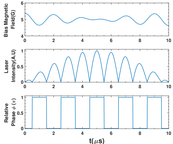
FIG. 2. From top to bottom: (a) driving signal of the magnetic field, (b) laser intensity, and (c) relative phase between lasers. The driving parameters are \Omega = 2\pi \times 50\text{kHz} , \omega = 2\pi \times 500\text{kHz} . Here we only show the driving signals for the first 10\mu\text{s} .
