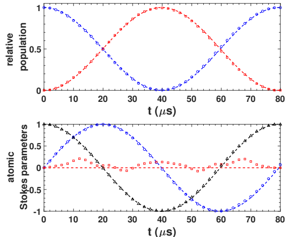
FIG. 3. Simulation results of an SU(2) transformation, where circles and squares and triangles are simulation results from solving the TDSE in the rotating frame, and dashed lines are analytical curves calculated in the Floquet basis under adiabatic approximation. Upper plot: population transfer, blue and red represent |1\rangle and |2\rangle , respectively. Lower plot: evolution of the atomic Stokes parameters, where blue, red and black represent S_1 , S_2 , and S_3 , respectively. Here we use the parameters: maximum laser powers P_a = P_b = 271.7\mu W , beam waist w = 300\mu m , magnitude of the time-varying part of the bias magnetic field \Delta B = 0.368G , bias magnetic field average B_0 = 5G , which results in \Omega_0 = 2\pi \times 258.3\text{kHz} . The driving frequencies are \Omega = 2\pi \times 50\text{kHz} and \omega = 2\pi \times 500\text{kHz} . With the above parameters, the geometric phase result in a Rabi-like oscillation with a period T_{geo} \approx 80\mu s .
