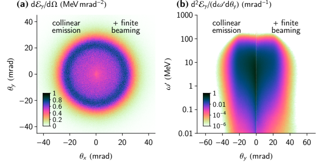
FIG. 4. The effect of the radiation beaming on the angularly resolved photon spectrum is much weaker when the laser is circularly polarized: density maps (colour scale, normalized to respective maxima) of (a) the energy radiated per unit solid angle and (b) the energy radiated per unit frequency and angle in the collision of a 500-MeV electron beam and a circularly polarized laser pulse with peak intensity 2 \times 10^{21} \text{ Wcm}^{-2} .
