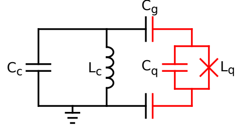
FIG. 6. (Color online) Circuit model for a 3D transmon circuit (red/gray) coupled to a linear cavity (black).
