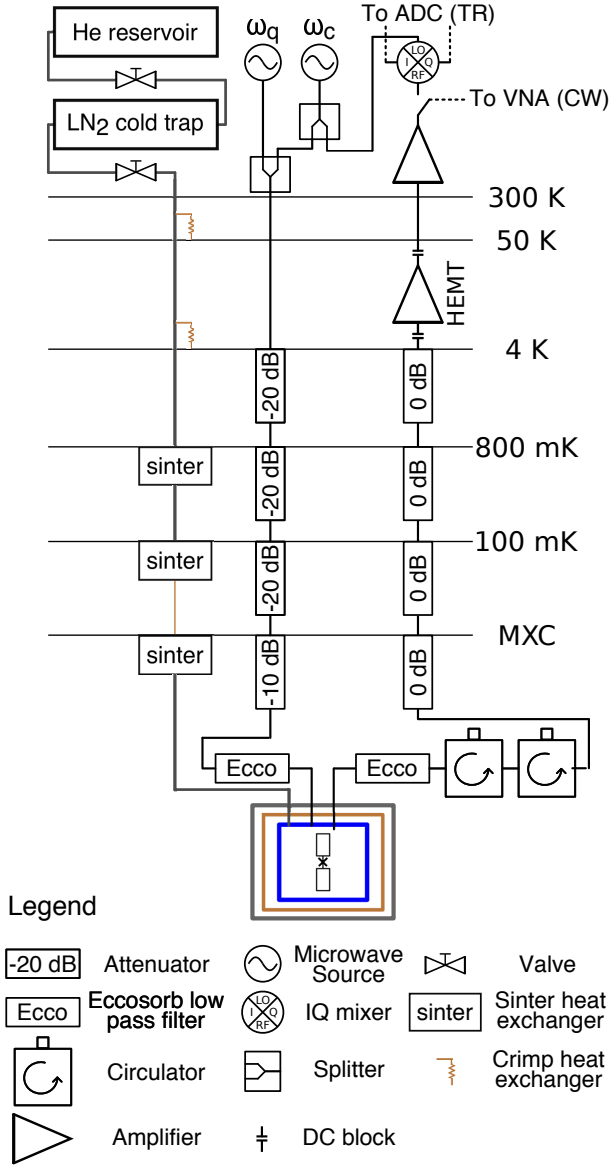
FIG. 5. (Color online) Schematic diagram of the experimental setup
