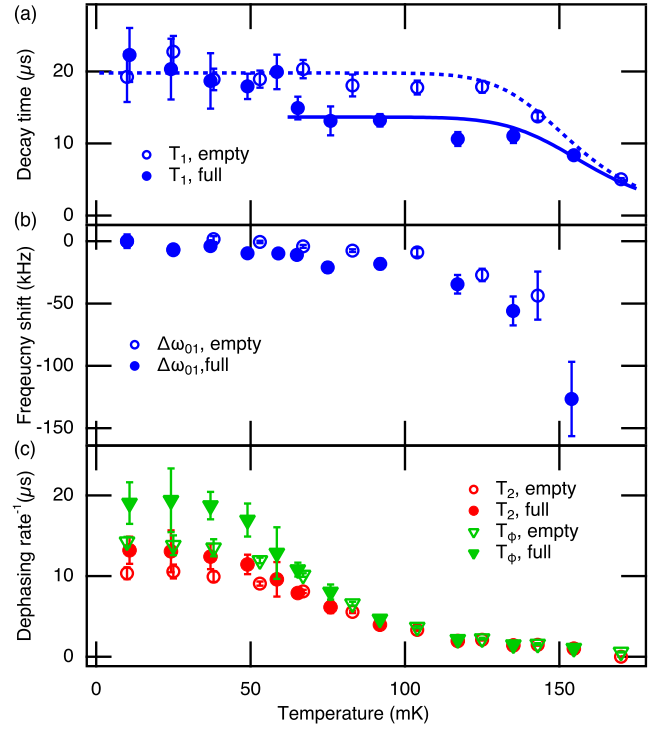
FIG. 3. (Color online) (a) Qubit energy relaxation time T_1 , as a function of temperature, for both the empty cavity and the cavity filled with superfluid helium. We fit the data to theory (see Ref. [19]) for quasiparticle limited T_1 , using only the superconducting gap of aluminum and the nonequilibrium quasiparticle density x_{qp} (solid and dashed curves) to extract the change in quasiparticle density above \sim 60 mK when the cavity is filled with superfluid (see main text for discussion.) (b) Qubit frequency shift relative to its base temperature value, (c) dephasing ( T_2 ) and pure dephasing ( T_\phi ) times of the qubit as a function of temperature, for both the empty and full cavity configurations.
