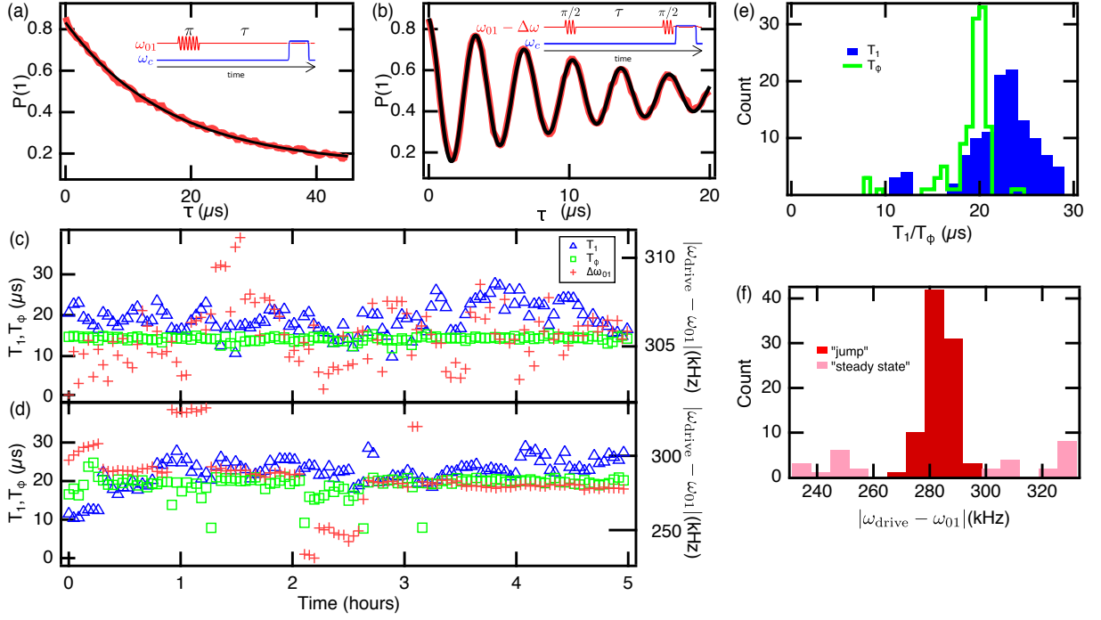
FIG. 7. (Color online) (a) Representative measurement of the qubit energy relaxation time T_1 inset with a schematic of the corresponding pulse sequence. We measure the probability P(1) of finding the qubit in the excited state |1\rangle after a variable delay time \tau after exciting it and fit the data to an exponential function to extract the decay time T_1 . (b) A representative free induction decay measurement, which is fit to a sinusoid superimposed on a decaying exponential function. From this fit we extract the dephasing time T_2 and the drive/qubit detuning |\omega_{\text{drive}} - \omega_{01}| . We interleave a single run of each measurement described in (a) and (b), and then repeat this for \sim 150 s to get a single data set to fit to. We repeat this process for 5 hours to gather statistics on long timescale fluctuations: (c) is a representative measurement of T_1 , T_\phi = (1/T_2 - 1/2T_1)^{-1} , and |\omega_{\text{drive}} - \omega_{01}| for the empty cavity at T \simeq 10 mK. (d) Is a similar measurement run at the same temperature but for the cavity filled with helium. Note the difference in scale between right axes of (c) and (d). (e) A histogram of the values of T_1 and T_\phi plotted in (d): The average and standard deviations of these datasets are what is reported in Fig (3) of the main text. (f) A histogram of the values of \Delta\omega_{01} recorded in (d): to measure the frequency shift as a function of temperature, we reject data measured during a discrete “jump” (light) and average over only data in “steady state” values of \omega_{01} (dark).
