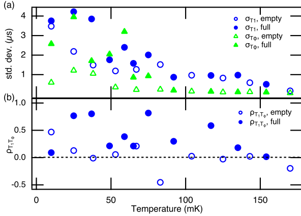
FIG. 8. (Color online) (a) Standard deviation of the measured datasets of T_1 and T_\phi for both empty and full cavities. (b) Normalized covariance of the sets of measured T_1 and T_\phi .
