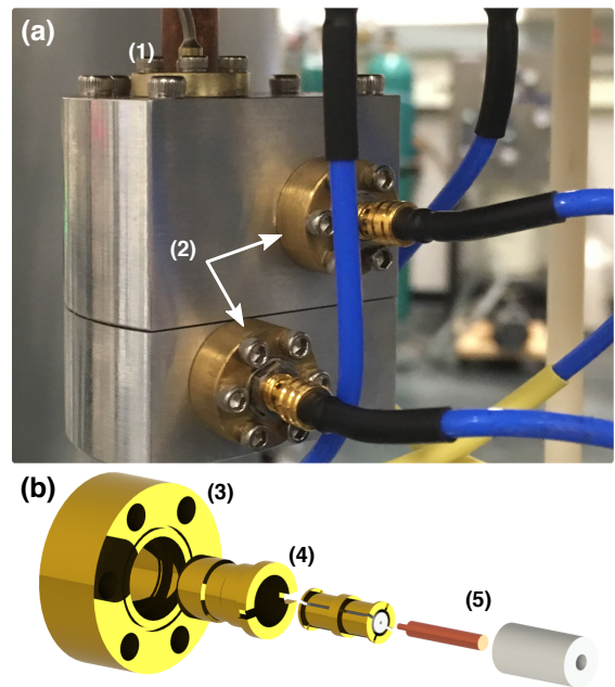
FIG. 1. (Color online) (a) Picture of the hermetically sealed 3D superconducting microwave cavity. Visible are (1) the helium fill capillary and flange and (2) the two microwave coupling ports. (b) Exploded rendering of the custom microwave coupling assembly. The hermetic GPO feedthrough (4) sits in a brass flange (3), and is sealed with an indium o-ring in between both the feedthrough and the flange, and the flange and the wall of the 3D cavity. A 50\ \Omega impedance matched copper pin (5) is soldered into a GPO “bullet” connector and extends to the inner wall of the cavity and provides coupling to the TE 101 fundamental mode of the cavity.
