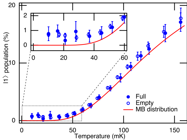
FIG. 4. (Color online) Residual population of the qubit excited state |1\rangle as a function of temperature for both the empty and superfluid filled cavity configurations. Also plotted is the theoretical Maxwell-Boltzmann (MB) distribution, calculated using the energy levels obtained from spectroscopy. The presence of helium in the cavity has no significant effect on the |1\rangle population, and the data fit the expected population well with no adjustable parameters. Inset: expanded view of boxed region. The |1\rangle population for the qubit saturates at roughly the same value both when the cavity is full of superfluid and when it is empty.
