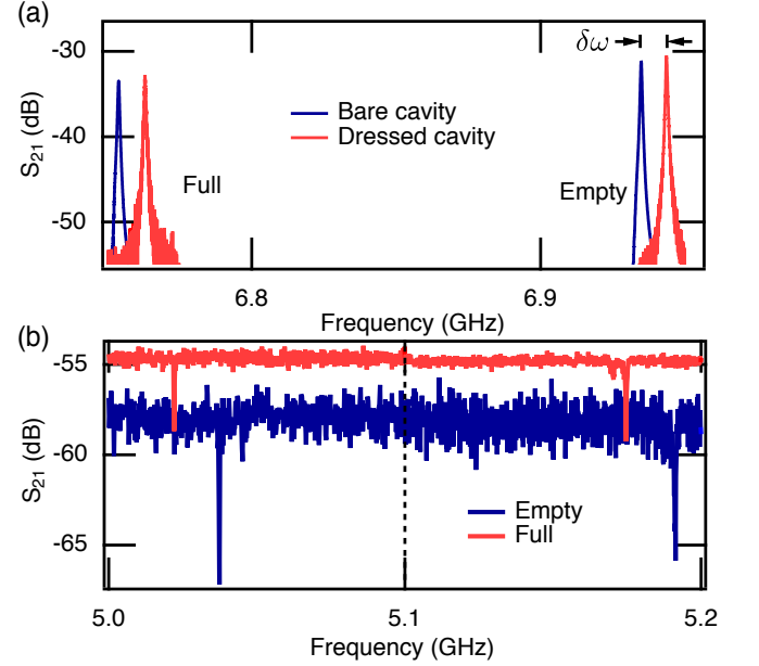
FIG. 2. (Color online) (a) Measured cavity transmission S_{21} as a function of frequency when the cavity is empty (right) and full of superfluid helium (left). Depending on the level of the applied microwave power we can measure both the cavity resonance dressed by the qubit in its ground state (red/light gray, P \approx -120 dBm) or the bare cavity resonance (blue/dark gray, P \approx -80 dBm.) (b) Two-tone spectroscopy of the qubit immersed in liquid helium (red/light gray) and in vacuum (blue/dark gray), offset vertically for clarity. Right of the dotted line, a low power tone is applied to excite the qubit ( P_q \approx -120 dBm) from its ground state |0\rangle to its first excited state |1\rangle , while to the left of the line a high power ( P_q \approx -90 dBm) tone is applied to induce a two photon transition from |0\rangle to |2\rangle . The dips in the transmission correspond to qubit excitation frequencies \omega_{01} (right) and (\omega_{01} + \omega_{12})/2 (left).
