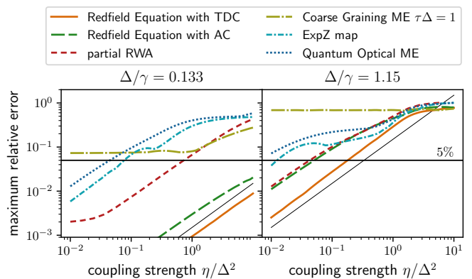
Figure 7. The scaling of the maximum relative error with the coupling strength \eta/\Delta^2 is shown for different correlation times. For all methods, except the Coarse-Grained Master Equation and the partial RWA , the scaling of the error in the limit of small coupling seems to be linear with the coupling strength (thin solid line). For the Coarse-Grained Master Equation and the partial RWA the few examples hint at a finite limiting error. Note, the non-monotonic behavior shown by the Redfield Equation is due to numerical integration errors.
