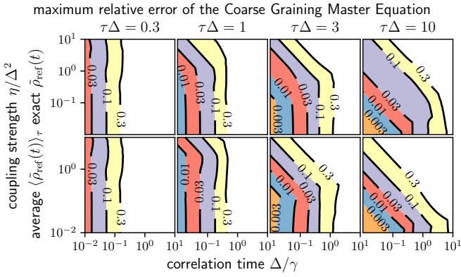
Figure 8. For the detuned case ( \Delta_A = \Delta , \Delta_B = 0.95\Delta ) the maximum relative error of the Coarse-Grained Master Equation when compared to the exact reduced state (upper row) and to its time average with coarse graining time \tau (lower row) is shown, without revealing significant differences. The columns refer to different coarse-graining times \tau . The kinks in the lines of equal error indicate that the condition \tau_{\text{env}} = 1/\gamma \ll \tau imposes an error which depends solely on the correlation time \Delta/\gamma and not on the coupling strength \eta/\Delta^2 . Further, the plot most left reveals that for short correlation times and a suitable coarse-graining time the Coarse-Grained Master Equation can deal with stronger couplings as compared to the Quantum Optical Master Equation (approximately shown in the most right panel).
