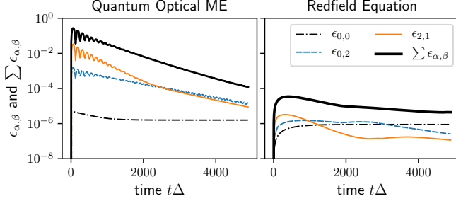
Figure 2. A selection of the partial deviations (thin lines) and the sum over all partial deviations (thick line) is shown for two detuned qubits ( \omega_A = \Delta and \omega_B = 0.95\Delta ) and a Lorentzian environment with \omega_c = \Delta , \gamma = 11.54\Delta and \eta = 0.02371\Delta^2 . In particular, the initial state independent error bound (dashed dotted line) reveal that the Redfield Equation with time dependent coefficients is significantly more accurate than the Quantum Optical Master Equation .
