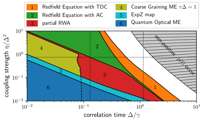
Figure 5. For each method, the plot shows the parameter region where the maximum relative error is smaller than 5% (detuned case \omega_A = \Delta and \omega_B = 0.95\Delta , initial condition \psi_0 = |\uparrow\uparrow\rangle and \omega_0 = \Delta ). Additionally, parameters which yield positivity violation for the reduced state obtained from the Redfield Equation with time dependent coefficients are marked by the line-filled area. Note, due to numerical errors the non-positivity condition was relaxed to \rho < -10^{-8} . The dotted lines correspond to the cuts shown in Fig. 6 and Fig. 7.
