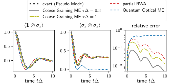
Figure 11. The dynamics of a local (left panel) vs. non-local (middle panel) expectation value is shown for two detuned qubits \omega_A = \Delta, \omega_B = 0.95\Delta . In the chosen regime (short correlation time \Delta/\gamma = 0.005 and strong coupling \eta/\Delta^2 = 150 ) considerable differences between the partial RWA and Coarse-Grained Master Equation become not only visible in the relative error of the reduces dynamics (right panel) but also in the non-local expectation value.
