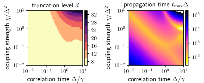
Figure 1. The truncation level of the pseudo-mode (left) and the propagation time t_{\text{max}} (right) required for the detuned qubits to approach the steady state up to 1% relative Hilbert-Schmidt distance.
