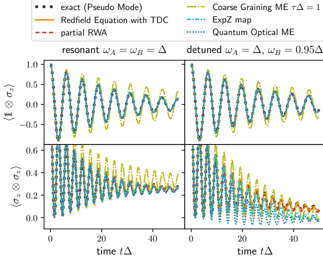
Figure 9. The time dependent expectation value of the local \mathbb{1}^A \otimes \sigma_z^B and non-local \sigma_z^A \otimes \sigma_z^B operator is shown for \eta/\Delta^2 = 0.149 and \Delta/\gamma = 0.673 . Only the Redfield Equation with time dependent coefficients reproduces the non-local quantity for detuned qubits correctly.
