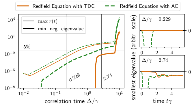
Figure 6. For fixed coupling strength \eta/\Delta^2 = 0.75 and varying correlation time \Delta/\gamma the shown maximum relative difference (thin lines) reveals a minor advantage in accuracy of the Redfield Equation with time dependent coefficients over its asymptotic variant Redfield Equation with asymptotic coefficients . However, concerning positivity, the minimum negative eigenvalue of the density matrix (thick line) indicates a significant difference between the two methods. That difference is due to the short time dynamics (right panels) where the Redfield Equation with asymptotic coefficients results in positivity violation on the timescale of the correlation time (see also Ref. [14, 47, 51, 55–57]). Only in a regime where the used approximation breaks down, long lasting positivity problems occur for both variants of the Redfield Equation .
