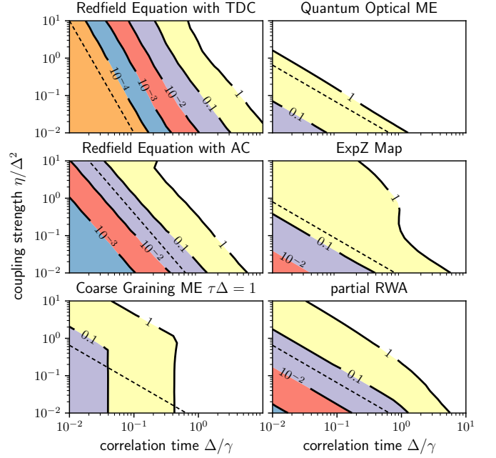
Figure 3. The absolute error bound based on the maximum value of the time dependent deviation \epsilon(t) is shown for different methods; detuned case \omega_A = \Delta and \omega_B = 0.95\Delta , Lorentzian environment with fixed central frequency \omega_0 = \Delta but varying coupling strength \eta and correlation time 1/\gamma . Dashed lines indicate a power law behavior for the lines of constant error ( Redfield Equation with time dependent coefficients (TDC): exponent -3 , Redfield Equation with asymptotic coefficients (AC): exponent -2 , others: -1 , see text). (Error bounds below 10^{-4} are prone to numerical error due to them being calculated from a difference in combination with the long propagation time of the particular parameter region.)
