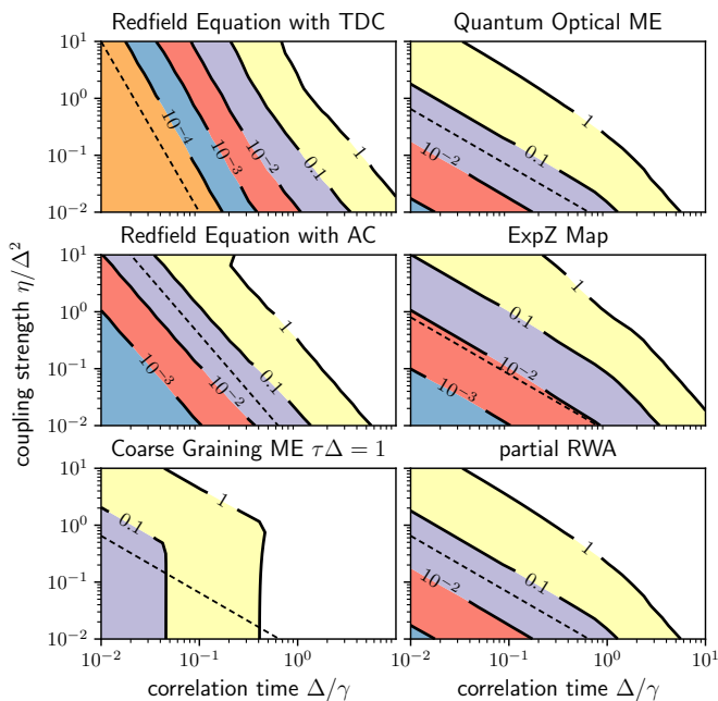
Figure 4. As in Fig. 3 the absolute error bound is shown for different methods but now for the resonant case \omega_A = \omega_B = \Delta .
