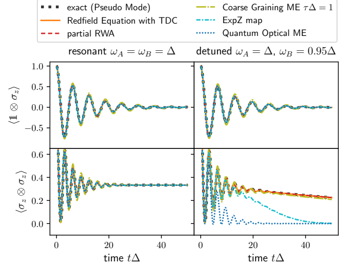
Figure 10. The same quantities as in Fig. 9 are shown for \eta/\Delta^2 = 1.29 and \Delta/\gamma = 0.165 . Notably, for detuned qubits the accuracy of the Coarse-Grained Master Equation has increased, whereas the Quantum Optical Master Equation and the related ExpZ Map have lost accuracy. Nevertheless, the local expectation value is well reproduced by all methods.
