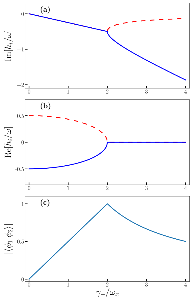
Figure 2. Spectral properties of the NHH in Eq. (42), showing an HEP. (a) Imaginary and (b) real parts of the eigenvalues in Eq. (43) as a function of \gamma_-/\omega_x : the ratio between the spin-flip rate and the drive. (c) Scalar product between |\phi_1\rangle and |\phi_2\rangle , given in Eq. (44), as a function of \gamma_-/\omega_x .
