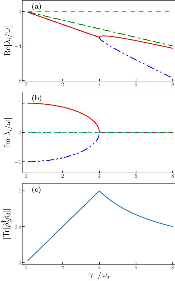
Figure 3. Spectral properties of the Liouvillian in Eq. (41), exhibiting a LEP, but for the same parameters as the NHH studied in Fig. 2. (a) Real part and (b) imaginary parts of the Liouvillian eigenvalues in Eq. (45) as a function of \gamma_-/\omega_x . Note that, according to Eq. (5), one should compare \text{Re}[\lambda_i] with \text{Im}[h_i] in Fig. 2(a), and \text{Im}[\lambda_i] with \text{Re}[h_i] in Fig. 2(b). (c) Scalar product between the two eigenmatrices \hat{\rho}_2 and \hat{\rho}_3 , given in Eq. (46), as a function of \gamma_-/\omega_x .
