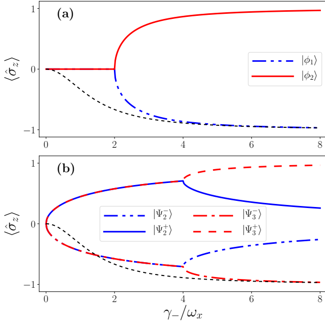
Figure 4. Expectation value of \langle \hat{\sigma}_z \rangle as a function of \gamma_-/\omega_x . In both panels the dashed black curves represent the mean value of photons in the steady state. (a) NHH eigenvectors [Eq. (44)]. (b) Eigenvectors obtained via the spectral decomposition of \hat{\rho}_{3,4} [cf. Eq. (48)].
