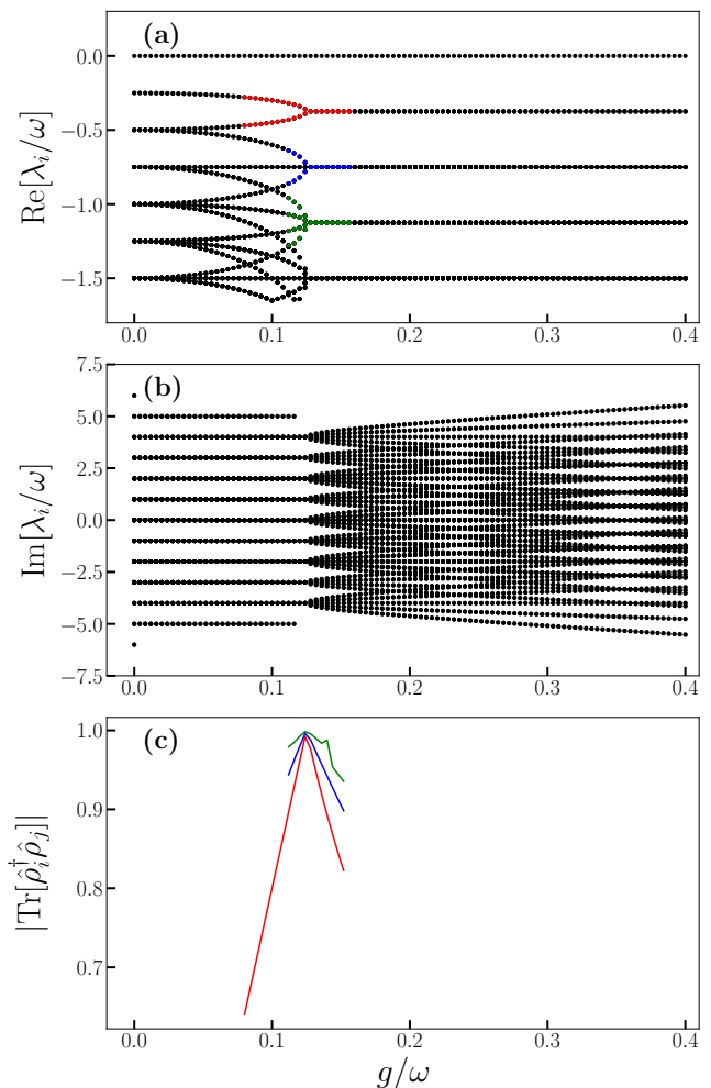
Figure 6. (Colors online) Spectral properties of the full Liouvillian in Eq. (50). (a) Real and (b) imaginary parts of the eigenvalues as a function of g/\omega . Note that, according to Eq. (5), one should compare \text{Re}[\lambda_i] with \text{Im}[h_i] in Fig. 5(a), \text{Im}[\lambda_i] with \text{Re}[h_i] in Fig. 5(b). (c) Scalar product between the eigenvectors associated with the EP, as a function of g/\omega . We were not able to extract this quantity for all the values of g/\omega due to numerical problems in correctly sorting the eigenvectors. Indeed, the eigenmatrices of \mathcal{L} do not obey anymore the total-excitation conservation law valid for the NHH. Here, the parameters used are: \gamma_a = \omega , \gamma_b = \omega/2 .
