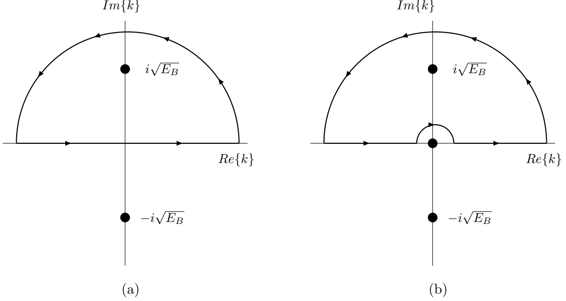
FIG. 1: (a) Contour for doing integration in Eq. (17). The poles are at k = \pm i\sqrt{E_B} but there is no pole at k = 0 . (b) Integration contour required for in Eq. (18). The poles are at k = \pm i\sqrt{E_B} and at k = 0 . The small detour around k = 0 contributes the extra -1/2 term.
