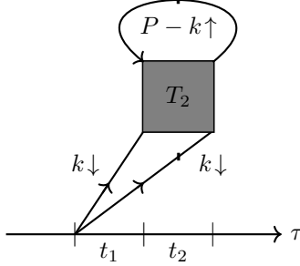
FIG. 2: Diagram corresponding to the calculation of \delta b_2 . The tree-level contact coupling is replaced by the full 1PI 2-body T-matrix T_2 , where T_2 is a function only of the center of mass momentum P flowing through the s-channel. The tick marks represent G^{(0,1)} propagators.
