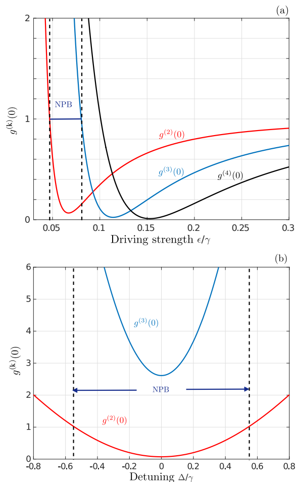
FIG. 6. Squeezed-reservoir model: Correlation functions g^{(k)}(0) versus: (a) the driving strength \epsilon for fixed \Delta = 0 and (b) the detuning \Delta for the maximally squeezed reservoir for n = 3 \times 10^{-4} , which corresponds to M = 0.017 , for fixed \epsilon = 0.07\gamma . All the parameters are scaled in \gamma units. The regions between the broken lines correspond to nonstandard single-photon blockade (type 2).
