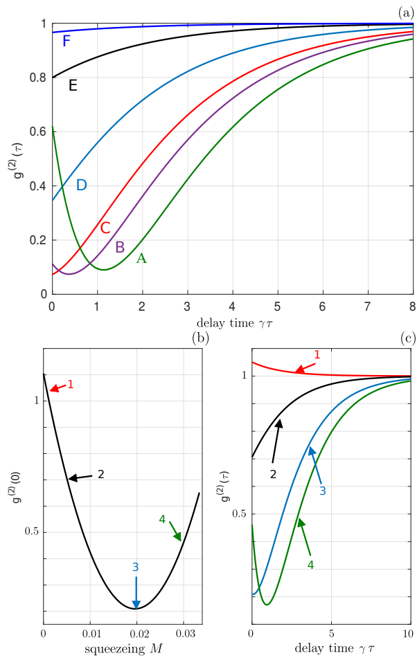
FIG. 2. Squeezed-reservoir model: Steady-state second-order correlation function g^{(2)}(\tau) versus: (a,c) the (rescaled) delay time \gamma\tau between the measurements of subsequent photons and (b) the reservoir squeezing parameter M for various values of the external field strength \varepsilon at the resonance, \Delta = 0 , between the cavity and external fields, with the damping rate \gamma = 1 . Moreover, in (a) we set \varepsilon/\gamma = 0.05 (curve A), 0.06 (B), 0.07 (C), 0.1 (D), 0.2 (E), and 0.5 (F), and assume that the reservoir is maximally squeezed with the reservoir mean photon number n = 0.003 , which corresponds to M = 0.017 . The \tau -dependences for the four specific points in (b) are shown in panel (c). In (b) and (c) we set \varepsilon/\gamma = 0.07 and n = 0.001 . It is evident that the curves 2 and 3 (1 and 4) show two-time photon antibunching (bunching) in panel (c). This implies that only the points 2 and 3 in panel (b) can correspond to “true” single-photon blockade states.
