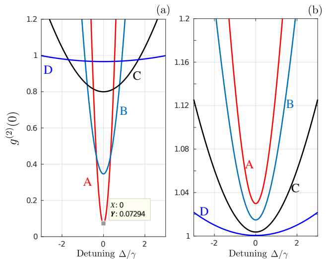
FIG. 7. Squeezed-reservoir model: Single-photon blockade in a driven harmonic resonator coupled to a squeezed reservoir. Specifically, the steady-state second-order correlation function g^{(2)}(0) versus the detuning \Delta between the cavity and driving frequencies for various values of the external field strength \varepsilon , assuming: (a) the squeezed-vacuum reservoir (see Appendix B) with M = \sqrt{n(n+1)} and (b) no squeezing ( M = 0 ) of the reservoir. We set the reservoir mean photon number as n = 3 \times 10^{-4} , and \varepsilon/\gamma = 0.07 (curve A), 0.1 (B), 0.2 (C), and 0.5 (D). All the parameters are scaled in \gamma = 1 units. Panel (a) shows strong single-time photon antibunching, especially for \varepsilon = 0.07\gamma and \Delta = 0 , which characterizes single-photon blockade. Panel (b) shows single-time photon bunching, which confirms that the single-photon blockade in panel (a) results from the squeezed reservoir.
