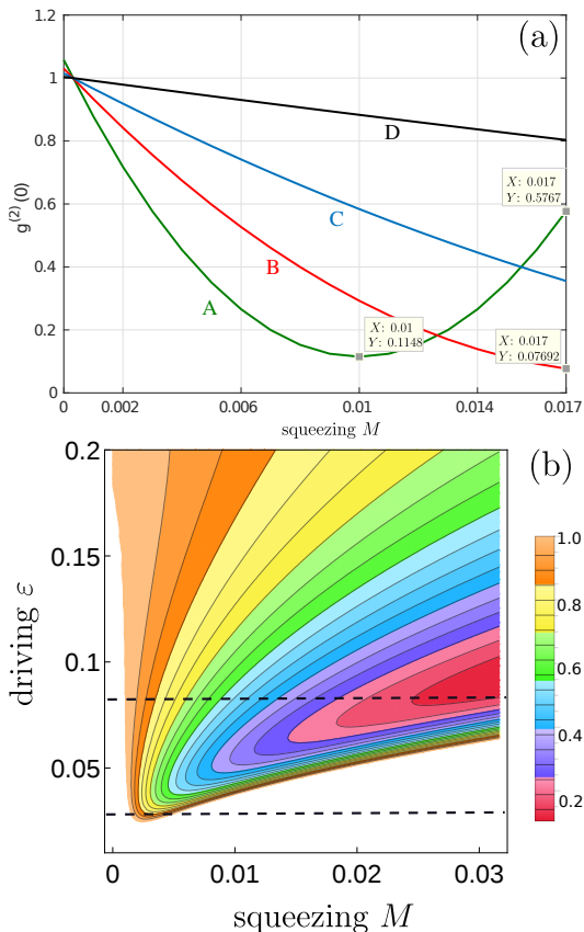
FIG. 8. Squeezed-reservoir model: Steady-state correlation function g^{(2)}(0) versus the reservoir squeezing parameter M and the driving strength \varepsilon in a driven harmonic resonator coupled to a squeezed reservoir. We set \varepsilon/\gamma = 0.05 (curve A), 0.07 (B), 0.1 (C) and 0.2 (D). Moreover, we assume resonance between the cavity and external fields, \Delta = 0 , and the mean photon number of the squeezed reservoir is n = 3 \times 10^{-4} . All the parameters are scaled in \gamma units. It is seen that, usually, a larger reservoir squeezing parameter M implies stronger single-time PAB, reaching the smallest value of g^{(2)}(0) for the squeezed-vacuum reservoir with M = \sqrt{n(n+1)} (see Appendix B). However, this is not the case for, e.g., \varepsilon = 0.05\gamma in panel (a), when there is an optimal value of M \ll \sqrt{n(n+1)} , which results in the strongest single-time PAB. The same surprising result is shown in panel (b) in the area between the dashed lines indicating the range of the external field strength \varepsilon for which g^{(2)}(0) has a minimum for M < \sqrt{n(n+1)} .
