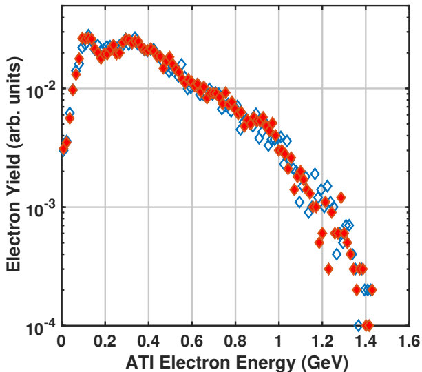
FIG. 5. ATI electron energy spectra for electrons produced by ionization of \text{Kr}^{35+} integrated over the focal volume. Electron initial conditions are calculated by simulation of immobile (closed diamonds, red) or mobile (open diamonds, blue) krypton ions in the focus. The peak laser intensity is 3 \times 10^{23} \text{ W/cm}^2 and focal spot 1/e^2 diameter is 3 \mu\text{m} .
