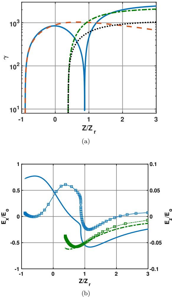
FIG. 7. a) Test electron \gamma as it travels through focus for representative initial conditions for RA (solid blue, negative z origin) and DIA (dashed-dotted green, positive z origin). Red dashed lines and black dotted lines represent identical initial conditions with the only first-order nonparaxial magnetic correction included. b) Electric fields acting on the test electrons. Color scheme is the same as a) for E_x (left scale). E_z (right scale) is represented by corresponding line style with open square markers. Electron motion is very nearly parallel to the z -axis.
