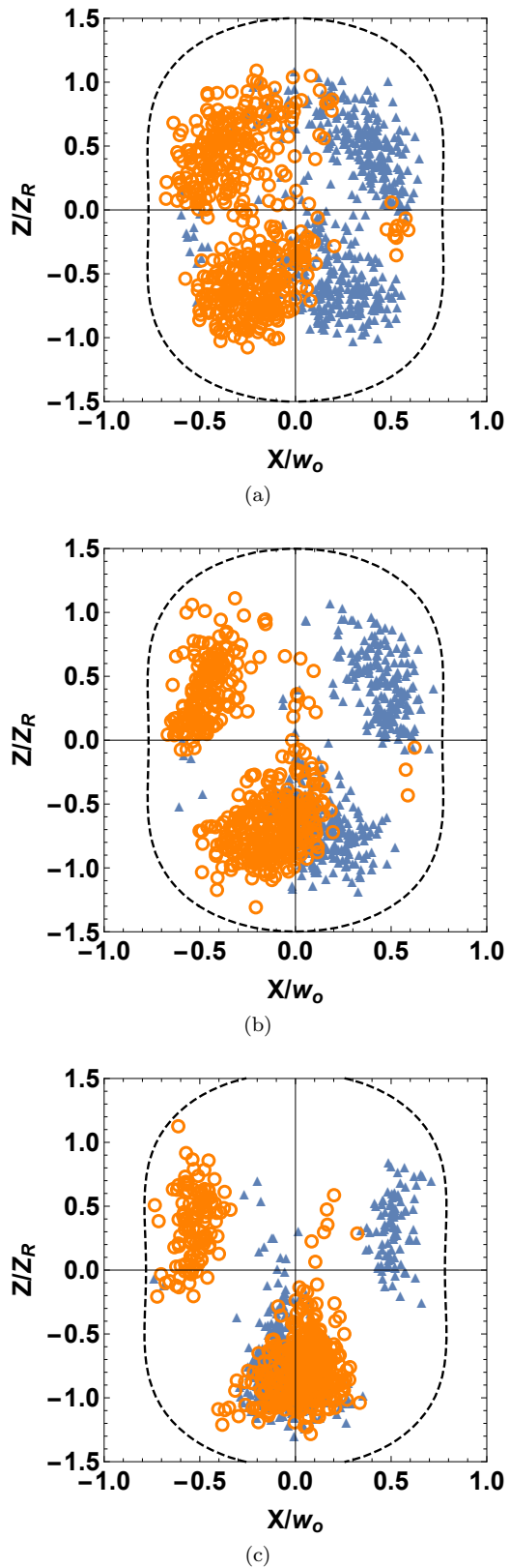
FIG. 6. Initial positions of the 10% highest-energy ATI electrons produced by a) \text{Ar}^{17+} at 4.7 \times 10^{21} \text{ W/cm}^2 , b) \text{Ti}^{21+} at 1.6 \times 10^{22} \text{ W/cm}^2 , and c) \text{Kr}^{35+} at 3 \times 10^{23} \text{ W/cm}^2 . Open orange circles (color online) denote negative E_x , solid blue triangles denote positive E_x . The focal spot 1/e^2 diameter is 3 \mu\text{m} . The black dashed curve represents the focal volume boundary containing all atoms (before arrival of the laser pulse) in the simulation.
