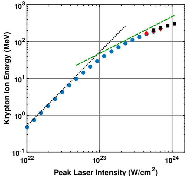
FIG. 3. Average energy of 500 krypton ions originating from (w_o/2, 0, 0) for different peak laser intensities. Peak laser intensity is defined at (0, 0, 0) . Blue circles indicate \text{Kr}^{34+} , red diamonds indicate \text{Kr}^{35+} , and black squares indicate \text{Kr}^{36+} . The black dotted line and the green dashed line are the short pulse maximum energies (Eq. 3) or ponderomotive energy for a \text{Kr}^{34+} ion, respectively. The focal spot 1/e^2 diameter is 3 \mu\text{m} .
