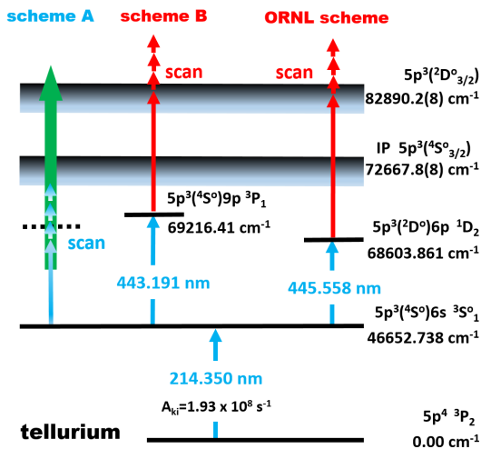
FIG. 2. Te excitation paths. Vacuum wavelengths are used. For the intermediate level of scheme B, the configuration 5p^3(^4S^o)9p\ ^3P_1 and level energy 69216.413\text{ cm}^{-1} are from this experiment; For the intermediate level of ORNL scheme, the configuration 5p^3(^2D^o)6p\ ^1D_2 and level energy 68603.861\text{ cm}^{-1} are from NIST ADS [28]; The IP value is from NIST ADS.
