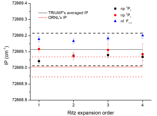
FIG. 6. Fitting model test with different Ritz expansion orders. TRIUMF’s and ORNL’s IP values are marked as solid straight lines in black and red, respectively. Their uncertainties, estimated as the sum of systematic and statistical uncertainties, are shown as the dashed line with the associated colors.
