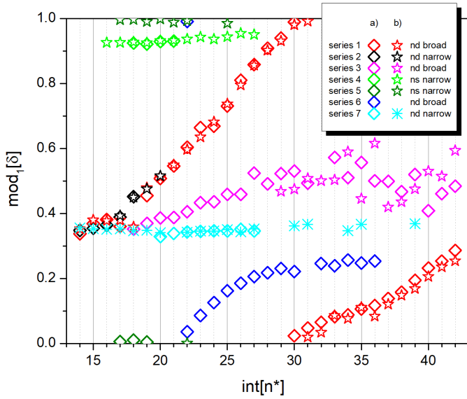
FIG. 8. Fano-Lu plot for the obtained AI states. Different series use different colors (online). All observed levels are symbolized as “◇” for spectrum a), “★” for spectrum b), and “*” for series 7 measured in our previous work at ORNL using the same excitation scheme [22].
