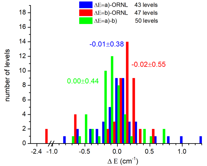
FIG. 9. Comparison of the level energies measured from spectrum a), b) and our previous work at ORNL. \Delta E was calculated as the differences between the measurements of each two spectra: spectrum a)-ORNL, spectrum b)-ORNL and spectrum a)- spectrum b). The statistic of each data set is labelled nearby the peak as “mean \pm standard deviation” of \Delta E .
