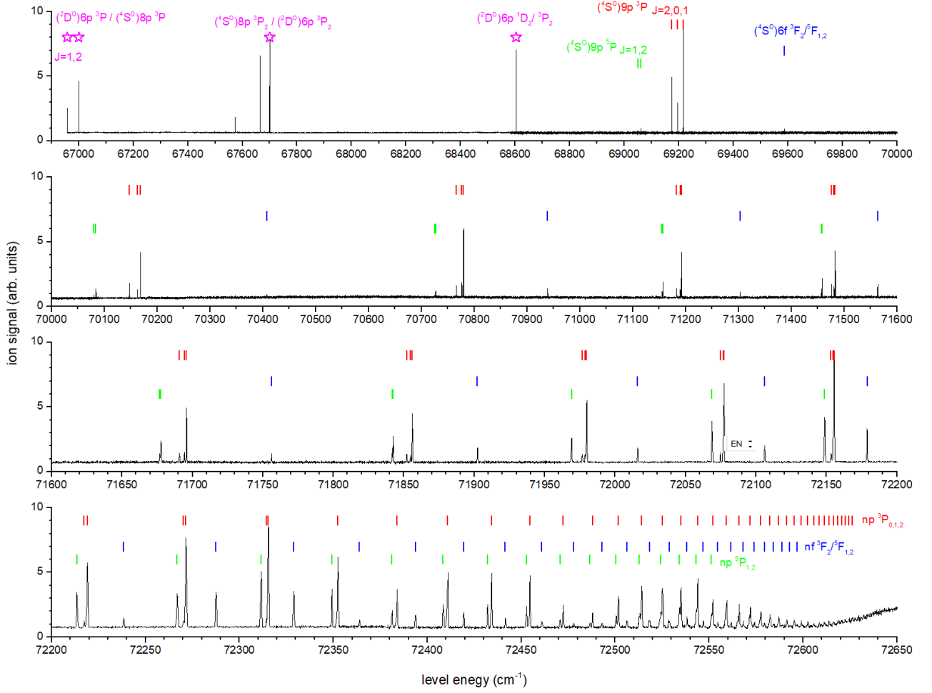
FIG. 3. Te even-parity Rydberg spectrum excited from the level of 5p^3(^4S_{3/2}^o)6s^3S_1 46652.738\text{ cm}^{-1} . The assigned levels are label with “|” and their principal quantum number n . Different series 5p^3(^4S_{3/2}^o)np^3P_{0,1,2} , 5p^3(^4S_{3/2}^o)np^5P_{1,2} and 5p^3(^4S_{3/2}^o)nf^3F_2/5F_{1,2} are colored as red, green and blue respectively, which matches with Fig. 4. The J values of fine structure sublevels are marked out in the top subplot. The observed levels that coincide with NIST data are labeled with “☆” and their assigned configurations as given in NIST database [28]. The spectrum is composed of three individual scans: 67000\text{--}68610\text{ cm}^{-1} , 68000\text{--}71350\text{ cm}^{-1} and 71300\text{--}72850\text{ cm}^{-1} . The scans were normalized via resonance peaks in the overlapping scan ranges. The laser power variation across the wide energy range (from \sim 30\text{mW} at the low energy to \sim 200\text{mW} at the high energy side) may affect the relative resonance peak heights.
