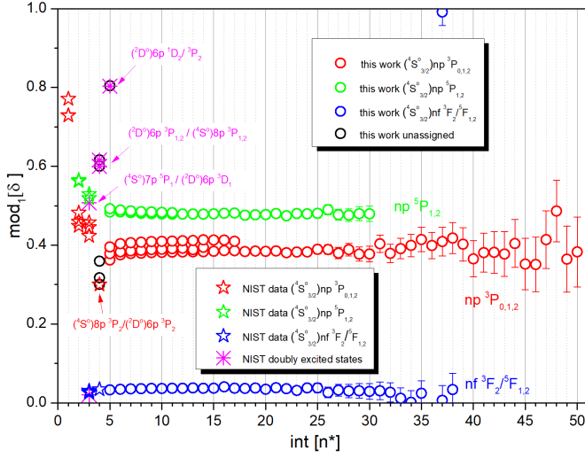
FIG. 4. Fano-Lu plot for the even-parity Rydberg series below the IP. The x-axis is the integer part of the effective quantum number n^* . The y-axis shows the decimal part of the quantum defect \delta which mathematically expresses as \text{mod}_1[\delta] . For np series, n = \text{int}[n^*] + 3 ; for nf series, n = \text{int}[n^*] . For clarity the fine structure sublevels of np^3P_{0,1,2} series are marked in a same color “red” (color online) although distinguishable at low n . Likewise the sublevels of np^5P_{1,2} are all in “green” (color online). The J values of the np^3P_{0,1,2} splittings are 2, 0 and 1 from high to low \delta respectively; for np^5P_{1,2} the J values are 1, 2 from high to low \delta respectively. Different symbols are used for our data and NIST data, but the same color for the same series.
