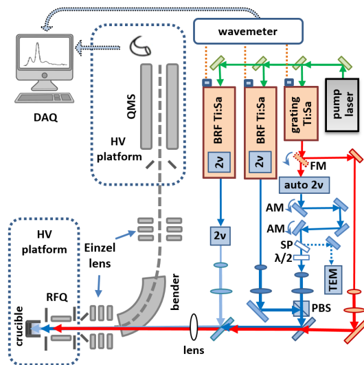
FIG. 1. Schematic setup for Te laser ionization spectroscopy. Details of intra-cavity and external doubling are omitted for clarity. DAQ: data acquisition system, QMS: quadrupole mass spectrometer, RFQ: radio frequency quadrupole, FM: foldable mirror, AM: automated mirror, SP: beam sampler, PBS: polarization beam splitter, TEM: TEM BeamLock detectors.
