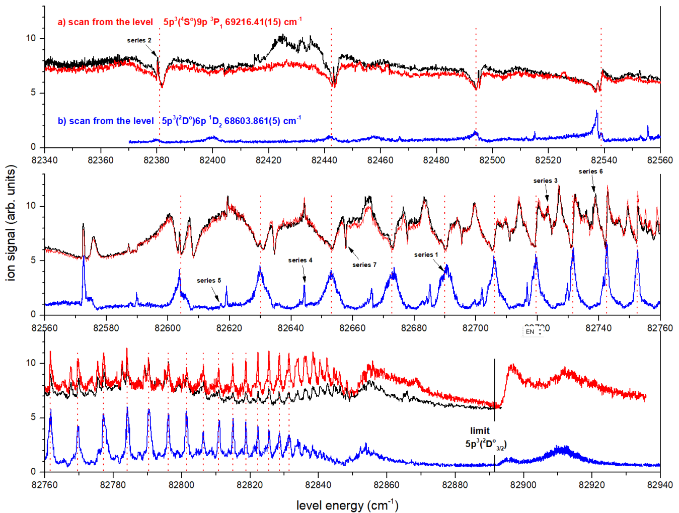
FIG. 7. AI Rydberg spectra excited from 5p^3(^4S_{3/2}^o)9p^3P_1 69216.41(15) \text{cm}^{-1} (spectrum a) and 5p^3(^2D_{3/2}^o)6p^1D_2 68603.861(5) \text{cm}^{-1} (spectrum b). An example of repeating the scan (black line) was presented for spectrum a). The ion signal is in arbitrary units (arb. units). For clearly displaying and comparing the spectra, spectrum a) were shifted up by 2 arb. units. The most prominent AI series (series 1) was marked by red dotted lines to guide the eye to the evolution of the resonance shapes.
