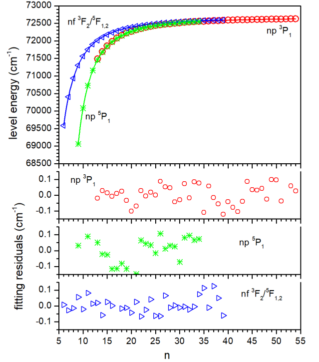
FIG. 5. Rydberg Ritz fits of the three series np^5P_1 , np^3P_1 and nf^3F_2/5F_{1,2} .
