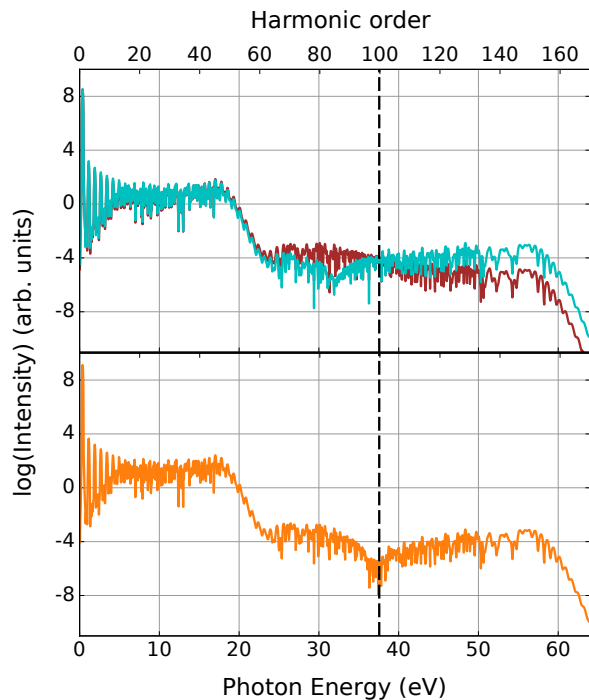
FIG. 5: Top panel: High-harmonic spectrum corresponding to the two-components of Eq. (4): -2\pi V_0/a[\langle\Phi(t)|\beta \sin(2\pi x/a)|\Phi(t)\rangle] (in brown or with higher greyscale value) and -2\pi V_0/a[\langle\Phi(t)|2\alpha \sin(4\pi x/a)|\Phi(t)\rangle] (in cyan or with lower greyscale value). Bottom Panel: The total High-harmonic spectrum corresponding to \langle\Phi(t)|\nabla V|\Phi(t)\rangle . The dotted line represents the region of the interference of the two-components and resultant minimum in the total spectrum. The harmonic spectrum is obtained for intensity of 8 \times 10^{11} W/cm 2 and wavelength of 3.2 \mu m.
