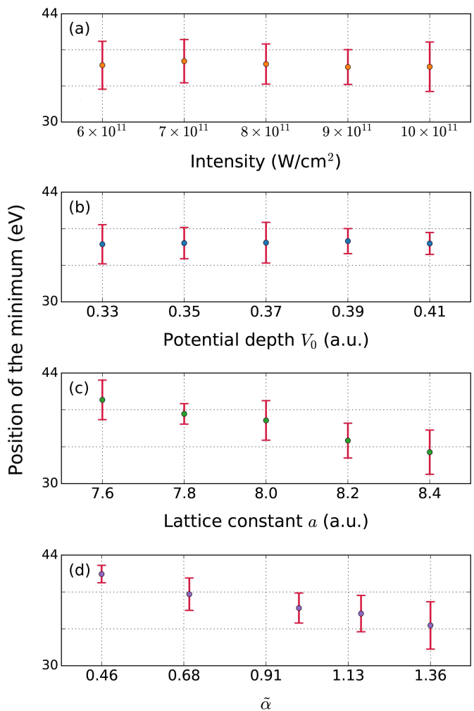
FIG. 3: The variation in the position of the minimum in the harmonic spectrum as a function of (a) intensity of the driving laser ( \lambda = 3.2\mu m , V_0 = 0.37 a.u. and a = 8 a.u.), (b) potential depth V_0 for the fixed lattice constant ( a = 8 a.u.), (c) as a function of the lattice constant ( a ) (for V_0 = 0.37 a.u.); and (d) as a function of the depth of the double-well potential \tilde{\alpha} = \alpha/\beta^2 (for V_0 = 0.37 a.u., a = 8 a.u.). In (b), (c) and (d), the laser intensity I = 8 \times 10^{11} were used. The error bar represents the width of the interference minimum.
