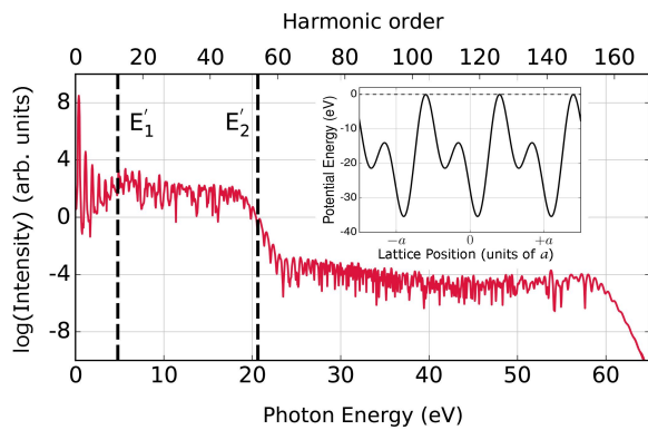
FIG. 4: High-harmonic spectrum for the asymmetric bichromatic periodic lattice (shown in inset). The harmonic spectrum is obtained for intensity of 8 \times 10^{11} W/cm 2 and wavelength of 3.2 \mu\text{m} . Here, E'_1 and E'_2 mark the minimum (4.79 eV) and the maximum (20.63 eV) band-gaps between the first conduction band and the valence band. The minimum energy band-gap is at the edge of the Brillouin zone ( k = \pm\pi/a ).
