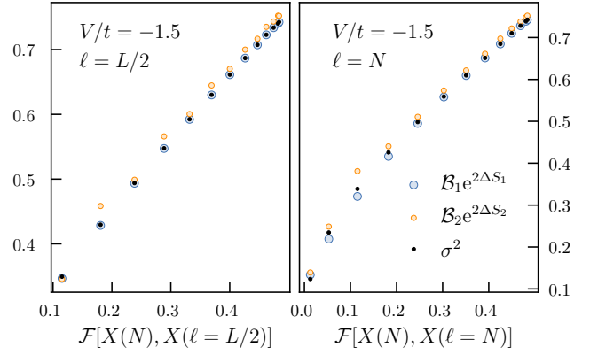
FIG. 8. The filling fraction dependence of the variance \sigma^2 (black dots) of the particle number distribution P_n compared to that computed from the difference between the (exponentiated) accessible and spatial entanglement entropies for \alpha = 1 (large circles) and \alpha = 2 (small circles) using Eq. (29). Exact diagonalization results in the ground state of the t - V model with V/t = -1.5 and L = 28 demonstrate consistency with the predicted asymptotic scaling function \mathcal{F}(N, \ell) given in Eq. (27) where we have fixed \ell = L/2 (left panel) or set \ell = N (right panel) and changed N from 2 \dots 14 . In order to reduce finite size effects, both of the partition size \ell and the total number of particles N are replaced by their corresponding chord length X(\ell) = (L/\pi) \sin(\pi \ell/L) and X(N) , respectively. The constants \mathcal{B}_1 = (\pi e)^{-1} and \mathcal{B}_2 = (2\pi)^{-1} are used to rescale the entanglement reduction to obtain a prediction for the variance \sigma^2 .
