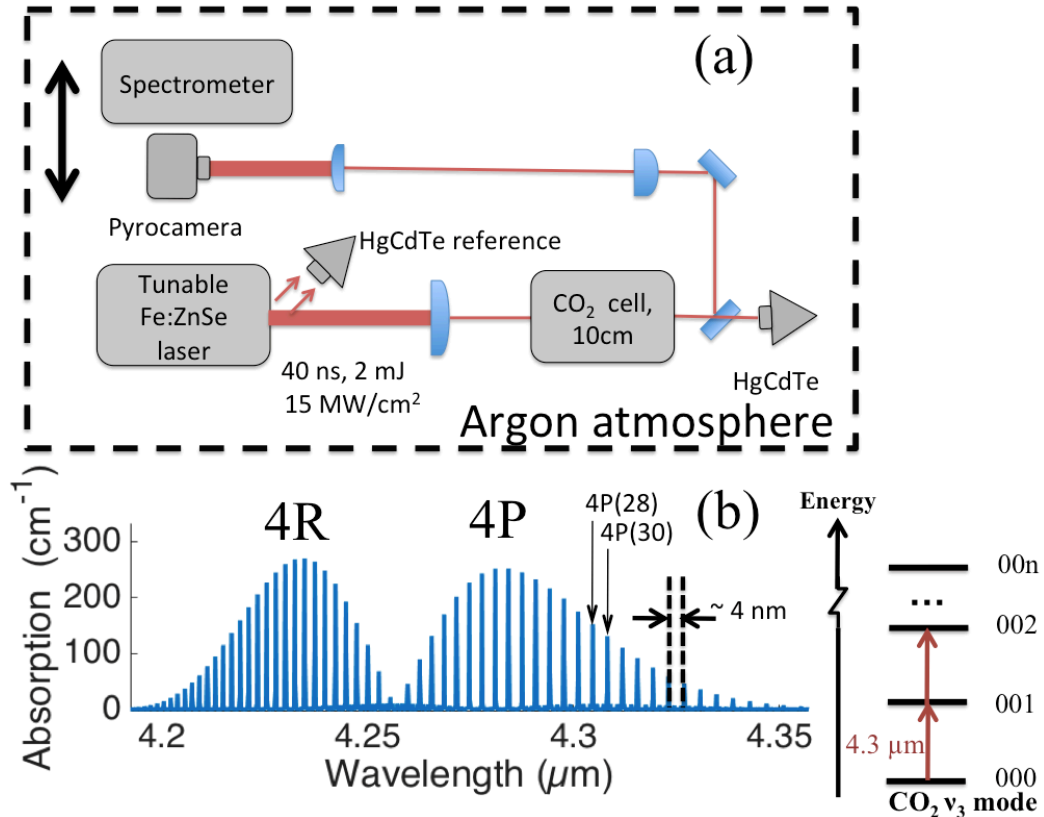
Figure 1: (a) Simplified experimental setup used for measurements of resonant self-focusing and self-defocusing of 4.3 \mu\text{m} light in \text{CO}_2 gas and (b) absorption spectrum of \text{CO}_2 (100 torr, 295 K) obtained from the HITRAN database showing the rovibrational structure of the so-called 4R and 4P branches [13]. The inset is a simplified energy level diagram of \text{CO}_2 showing only the 4.3 \mu\text{m} 000 - 00n ( v_3 ) vibrational asymmetric stretching mode.
