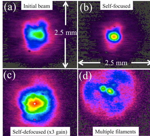
Figure 2: (a) Initial 4.3 \mu\text{m} beam profile and beam profiles for a case when the laser was tuned to the (b) self-focusing and (c) self-defocusing sides of a rovibrational line located on the wing of the 000 - 001 4P branch of \text{CO}_2 . (d) Beam profile showing transverse beam break-up indicative of multiple filamentation for a case when the laser was tuned to the self-focusing side of a rovibrational line near the peak of the 4P branch.
