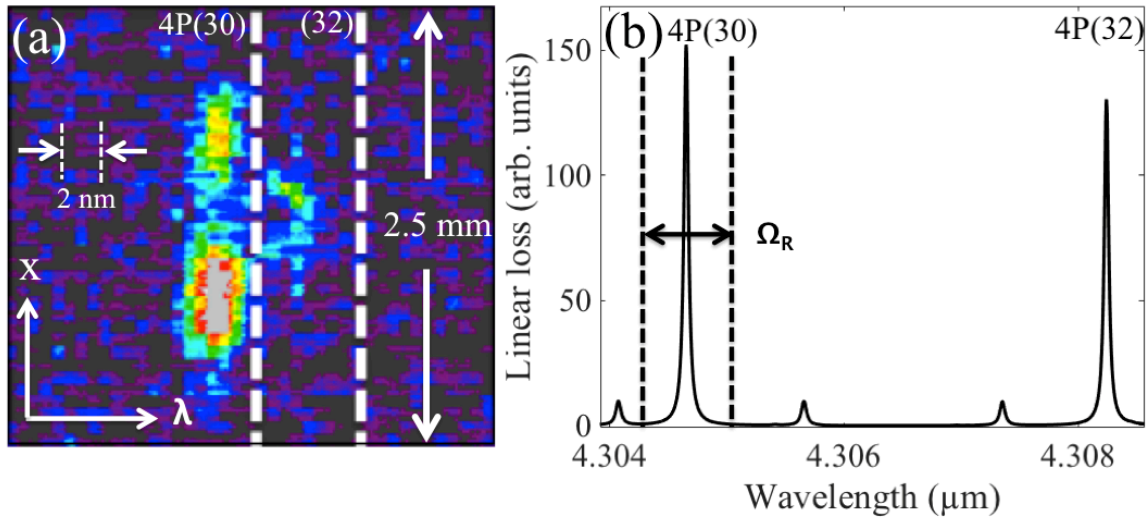
Figure 5: (a) Frequency-resolved self-focusing measurement showing apparent power broadening of the 4P(30) line of \text{CO}_2 . The field dependence of the Rabi frequency gives rise to a ring-shaped intensity distribution since the maximum shift is on-axis where the laser intensity is maximum. (b) The absorption spectrum of \text{CO}_2 in the vicinity of the 4P(30) and 4P(32) line from the HITRAN database with a depiction of the level splitting that may be achieved based on the calculated Rabi frequency.
