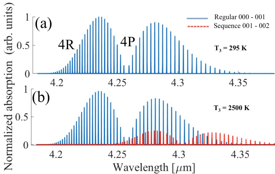
Figure 8: Calculated absorption spectra showing lines corresponding to the 000 – 001 and 001 – 002 transitions of the \text{CO}_2 molecule for a vibrational temperature of (a) 295 K and (b) 2500 K.
