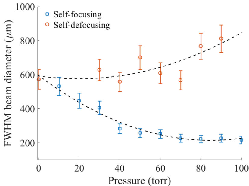
Figure 3: The evolution of the FWHM beam profile as a function of \text{CO}_2 pressure for a case when the laser was tuned to the self-focusing (blue squares) and self-defocusing (orange circles) sides of resonance. The dashed lines are quadratic fits to the data intended to guide the eye.
