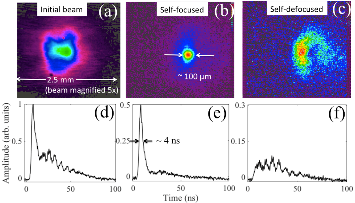
Figure 6: Beam profile measurements of (a) the initial beam, (b) the self-focused, and (c) self-defocused beam that correspond to temporal pulse profile measurements (d), (e), and (f), respectively. Note that pulse consisted of a 4 ns FWHM spike followed by a 30 ns tail and that only the initial spike was subjected to nonlinear focusing. Note that the vertical axes of (d), (e), and (f) are normalized to the peak amplitude of the initial laser pulse. These measurements were performed in the vicinity of the 4P(30) line where the absorption was \sim 50\% for (b), (e) and \sim 70\% for (c), (f).
