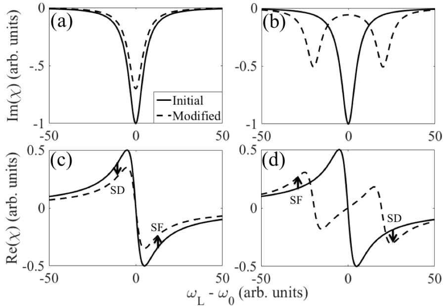
Figure 7: Imaginary and real parts of the susceptibility ( \chi ) when modified by (a), (c) saturation and (b), (d) power broadening, respectively. Note that \omega_L - \omega_0 is the detuning where \omega_L is the laser frequency and \omega_0 is the resonant frequency. SF and SD denote regions of self-focusing and self-defocusing, respectively.
