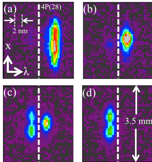
Figure 4: Frequency-resolved measurements of self-focusing and self-defocusing in the vicinity of a rovibrational line of the 000 – 001 transition of \text{CO}_2 . (a) Shows the unaffected beam where the location of the line is marked by the vertical dashed line. (b) Shows the beam self-focusing as the rovibrational line is approached from the red side of resonance. (c) Shows the laser spectrum both focusing and defocusing on either side of resonance. (d) Shows the laser defocusing on the blue side of resonance. It should be noted that the dumbbell shape is the one-dimensional cross-section of the donut-shaped beam that is produced from self-defocusing and that the elongated beam profiles result from imaging the slit of the spectrometer.
