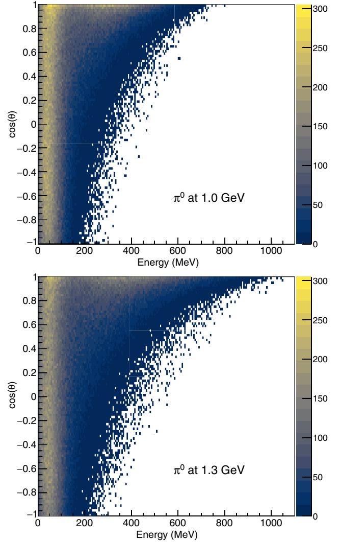
FIG. 15. Distribution of production angles and creation energies of \pi^0 at the SNS-FTS assuming an aluminum PBW. Top: using 1 GeV incident protons to mimic the current operating conditions of the SNS. Bottom: using 1.3 GeV incident protons to mimic the operating conditions following the upgrade.
