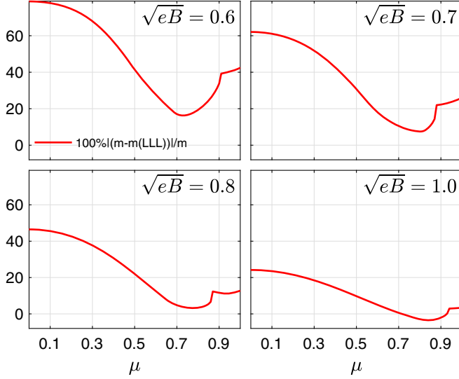
FIG. 2. Percentage deviation, [(m - m(\text{LLL}))/m] \times 100\% , versus chemical potential for four magnetic-field values and at a coupling constant G = 3 . The deviation is taking between the induced mass calculated summing in all LLs, m , and only considering the LLL, m(\text{LLL}) .
