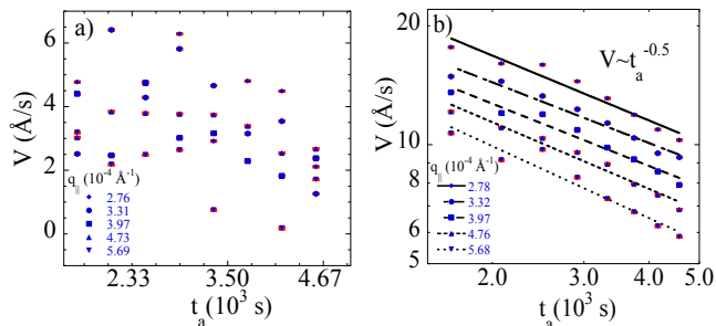
FIG. 4. Mean velocity V as a function of t_a for different wave vectors q_{\parallel} for (a) 1000 Å top surface at t_w = 6811 s and (b) buried interface of the bilayer at t_w = 21427 s.
