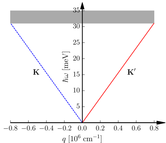
FIG. 1. The edge second sound dispersion for a half-gap \Delta/k_B = 180 K and a temperature T = 90 K [ k_B T/(2\Delta) = 1/4 ]. The shaded region correspond to the particle-hole continuum ( \hbar\omega > 2\Delta ). Note that the edge second-sound modes are completely valley polarized.
