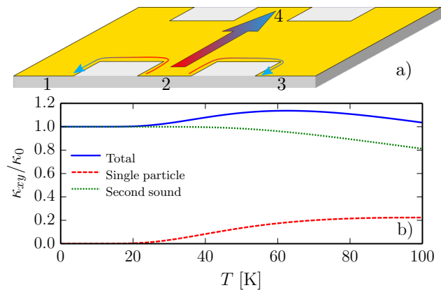
FIG. 3. Panel (a) the proposed experimental setup. A thermal gradient is applied between the middle contacts (2 and 4), and the temperature drop is measured on contacts 1 and 3. The non-local temperature drop can be related to the transverse thermal conductance as in [65, 66]. Panel (b) The thermal conductance \kappa_{xy} [in units of the thermal conductance of a perfect one-dimensional bosonic channel \kappa_0 = \pi^2 k_B^2 T / (3h) ] as a function of the temperature (in K). We also plot the two components \kappa_{xy}^{\text{sp}} and \kappa_{xy}^{\text{ss}} in the same units. Note that at low temperature the single-particle contribution is completely suppressed, and the transport is dominated by edge collective modes. At higher temperature the fast growth of \kappa_{xy}^{\text{sp}} leads to a change in the slope of the total thermal conductance.
