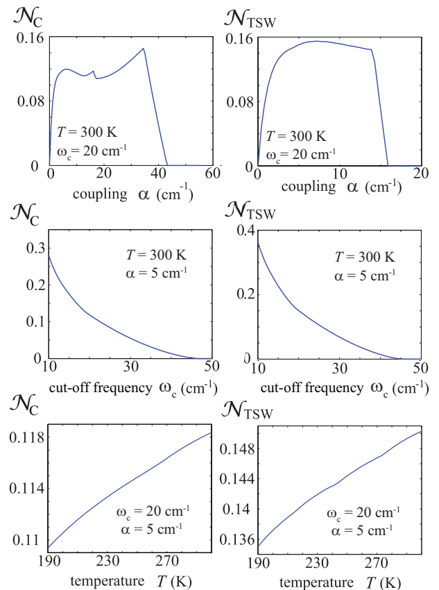
FIG. 2. (Color online) The non-Markovianity measures, \mathcal{N}_{\text{TSW}} (based on the temporal steerable weight) and \mathcal{N}_C (based on the entanglement with an ancilla), as a function of system-reservoir coupling \alpha , reservoir cut-off frequency \omega_c and temperature T , for a two-level system coupled to a bosonic reservoir with Drude-Lorentz spectral density. The system parameters are chosen to maximize the affect of the reservoir memory, with E = 0 and \Delta = 100\text{cm}^{-1} . The magnitude of these parameters are typical for excitation energy transfer in photosynthesis [41], where the memory effect and structure of the environment is thought to play an important role.
