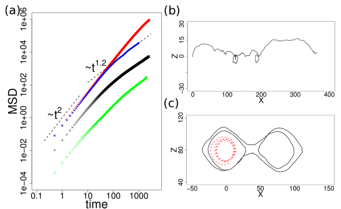
FIG. 2: (Color online) (a) MSDs for \phi = 0.2 ( \times ), 0.4 ( \diamond ), 0.5 ( \bullet ), 0.56 ( \blacktriangle ). Representative trajectories for (b) \phi = 0.40 , (c) 0.50 . The red and black lines refer to trajectories of different rotors.
