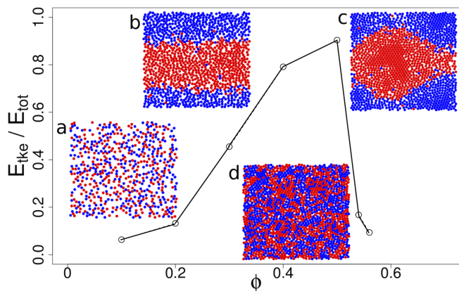
FIG. 1: (Color online) The ratio of the translational kinetic energy to the total kinetic energy \kappa = E_{tke}/E_{tot} as a function of rotor density \phi . The insets are snapshots of simulations (50-50 mixture of clockwise (blue)–counterclockwise (red) spinning rotors) with total density (a) \phi=0.20 , (b) 0.40, (c) 0.50, and (d) 0.54. Movies are available in the supplementary material [35].
