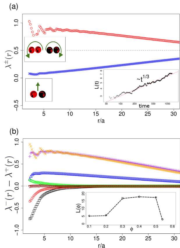
FIG. 3: (Color online) (a) Normalized partial number density of same-spin ( \lambda^- ; \circ ) and opposite-spin ( \lambda^+ ; \times ) rotors for \phi = 0.5 at steady state. Insets illustrate co- and counter-rotating particles and their joint rotation or translation. The inset shows a \sim t^{1/3} growth of the lengthscale from the initial random configuration. (b) Average density difference between coherently moving same-spin and opposite-spin rotors, \lambda^- - \lambda^+ , for \phi = 0.1 ( \square ), 0.2 ( \circ ), 0.3 ( \triangle ), 0.4 ( + ), 0.5 ( \times ), 0.54 ( \diamond ), and 0.56 ( \nabla ). The inset shows the final integrated lengthscale L as a function of \phi .
