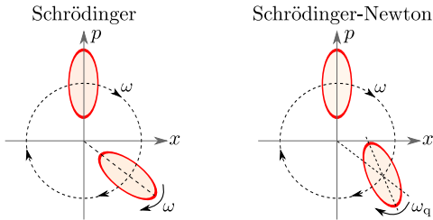
Figure 1: (Color online). Left Panel: according to standard quantum mechanics, both the vector (\langle x \rangle, \langle p \rangle) and the uncertainty ellipse of a Gaussian state for the CM of a macroscopic object rotate clockwise in phase space, at the same frequency \omega = \omega_{\text{CM}} . Right panel: according to the CM Schrödinger-Newton Equation (2), (\langle x \rangle, \langle p \rangle) still rotates at \omega_{\text{CM}} , but the uncertainty ellipse rotates at \omega_q \equiv (\omega_{\text{CM}}^2 + \omega_{\text{SN}}^2)^{1/2} > \omega_{\text{CM}} .
