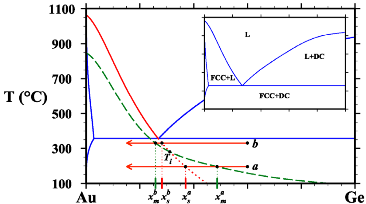
Figure 2: Calculated [26-28] phase diagram for the Au-Ge system with the metastable AuGe liquidus curve. The solidus curves, DC liquidus curve, and eutectic temperature are given in blue. The red solid curve indicates the FCC Au liquidus line above the eutectic temperature with the extended subeutectic FCC Au liquidus indicated by the dotted red curve. The green broken line indicates the metastable AuGe liquidus. The temperature where the two liquidus lines intersect is indicated by T_i . The inset is the unaltered equilibrium Au-Ge phase diagram.
