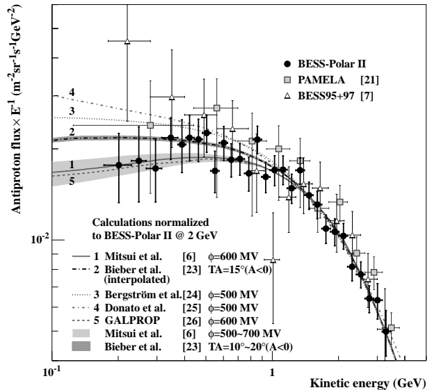
FIG. 3. Comparison of \bar{p} flux shapes with secondary calculations normalized to BESS-Polar II flux at 2 GeV. Sensitivity to uncertainty in the force-field modulation parameter is shown by the lower shaded band. The small sensitivity of secondary \bar{p} drift calculations at solar minimum to tilt angle is illustrated by the upper shaded band.
