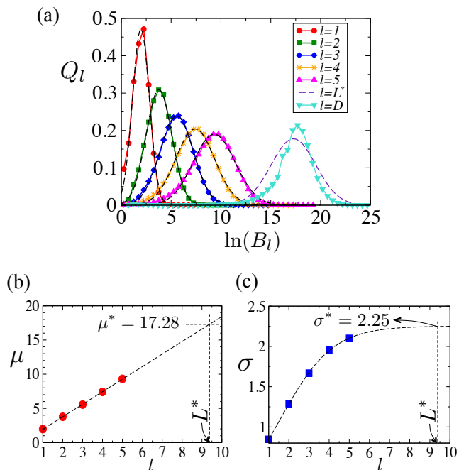
FIG. 5: (Color online) a) Distribution Q_l of the \ln(B_l) values in the SocNet for l = 1, 2, 3, 4, 5, D , where D = 26 is the diameter, and the predicted distribution for L^* . The distributions can be fitted with a Gaussian. b) The average \mu and c) standard deviation \sigma as function of l . Extrapolating to L^* = 9.35 we obtain \mu^* = 17.28 and \sigma^* = 2.25 .
