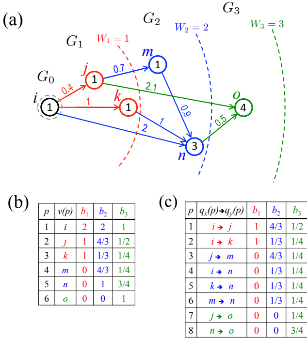
FIG. 6: (Color) a) Shells of the C_3 subgraph of node i (black) are colored red, blue, green. Distances defining the shells are: W_1 = 1, W_2 = 2, W_3 = 3 . The weight or length is shown next to each edge. Given a node j , the number inside its circle is the total number of shortest paths coming from the root i : \sigma_{ij} . b) The list of nodes v(p) and c) list of edges q_x(p) \rightarrow q_y(p) are shown together with their 1-, 2-, and 3-betweenness values.
