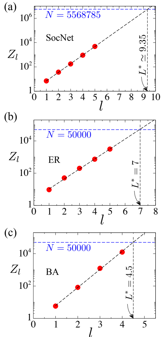
FIG. 2: (Color online) Volume Z_l growth with radius l . a) Extrapolating the growth for SocNet one can estimate that it reaches the N = 5\,568\,785 mark at L^* \simeq 9.35 . Similarly, there is exponential growth for both ER, b) and BA models, c).
