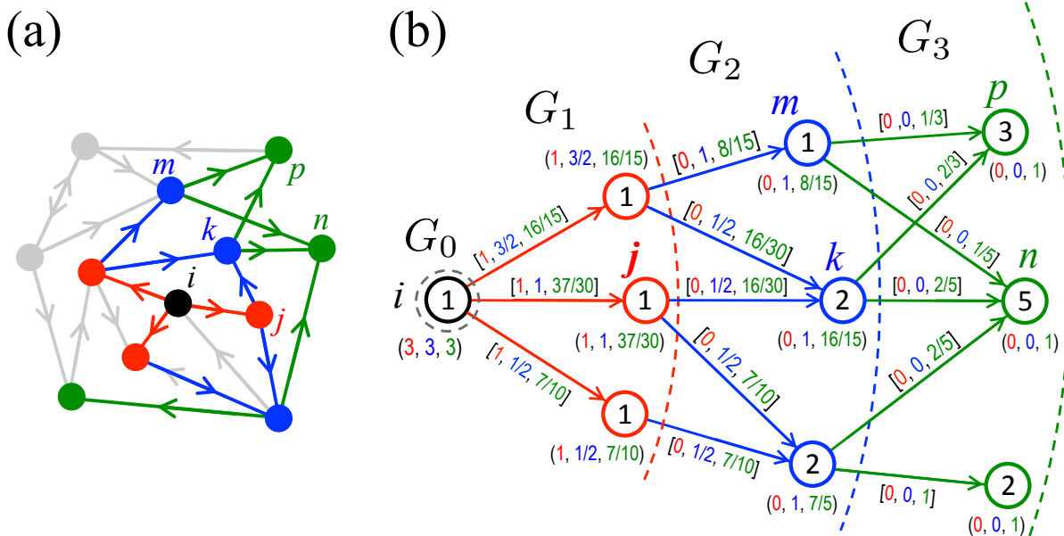
FIG. 1: (Color) a) Consecutive shells of the \mathcal{C}_3 subgraph of node i (black) are colored red, blue, green. Grey elements are not part of the subgraph. b) The (x, y, z) near a node j are the b_\ell(i|j) values for \ell = 1, \ell = 2 and \ell = 3 . The [x, y, z] on an edge (j, k) give the b_\ell(i|j, k) values for \ell = 1, \ell = 2 and \ell = 3 . Given a node j , the number inside its circle is the total number of shortest paths \sigma_{ij} to j from i . Colors indicate quantities based on \ell = 1 (red), \ell = 2 (blue), and \ell = 3 (green).
