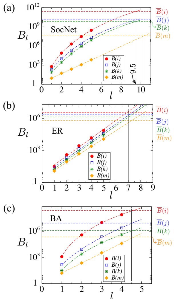
FIG. 4: (Color online) The [l] -BC values, B_l , of 4 individual nodes in the SocNet data a), in the ER b) and BA models as function of l . The exact/full BC value of each node is indicated by a horizontal dashed line, and denoted by \bar{B}(i) , \bar{B}(j) , etc. Extrapolating the range-limited values for larger l , the exact BC values are reached at around L^* in all cases.
