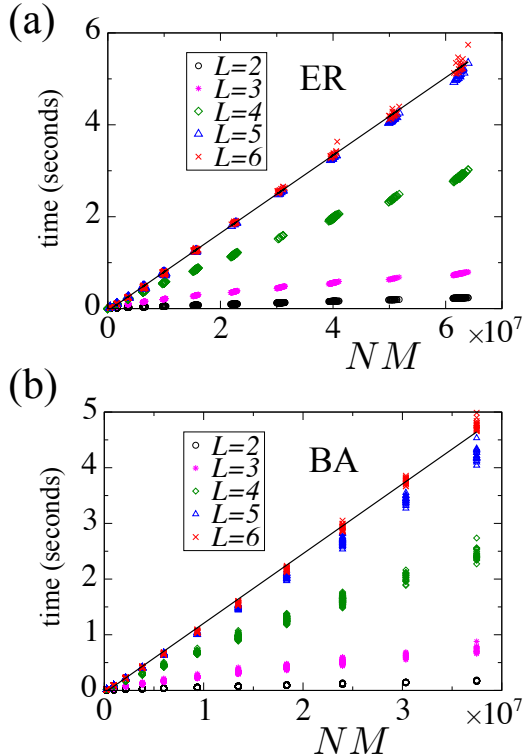
FIG. 3: (Color online) Scaling of range-limited betweenness computation times (in seconds) as function of NM for ER and BA models, where N is the number of nodes and M is the number of edges of the graphs. For ER the average degree was 5 and the BA model's parameter was m = 3 . The symbols are actual running times (not averages) for 100 networks, measured on an Apple quad core Mac Pro workstation.
