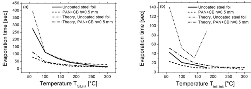
FIG. 10. Drop evaporation time on nanofiber-coated foils compared to the one on bare foils for (a) water and (b) ethanol.
