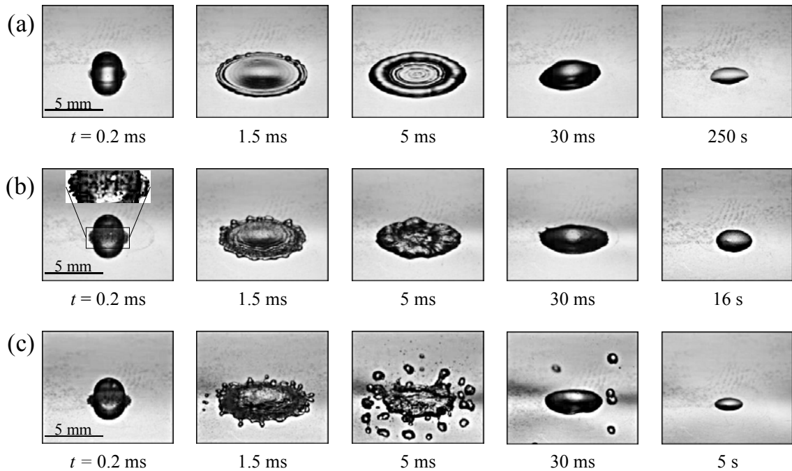
FIG. 3. Water drop impact on a bare steel foil at different initial foil temperatures.
