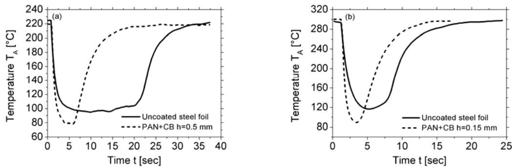
FIG. 7. Evolution of foil temperature under the drop impact point, T_A , for water drop impact. The initial foil temperature T_{\text{foil,init}} is equal to (a) 220^{\circ}\text{C} and (b) 300^{\circ}\text{C} .
