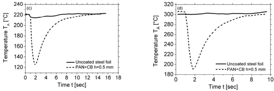
FIG. 8. Evolution of foil temperature under the drop impact point, T_A , for the ethanol drop impact. The initial foil temperature T_{\text{foil,init}} is equal to (a) 140^\circ\text{C} , (b) 180^\circ\text{C} , (c) 220^\circ\text{C} and (d) 300^\circ\text{C} .
