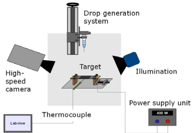
FIG. 2. Experimental setup for drop impact onto nanofiber mats.
