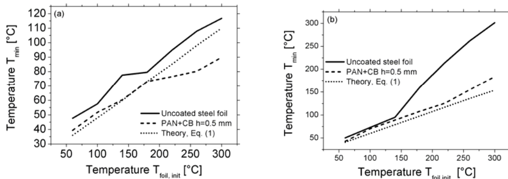
FIG. 9. Minimum foil temperature after drop impact as a function of the initial foil temperature for (a) water and (b) ethanol.
