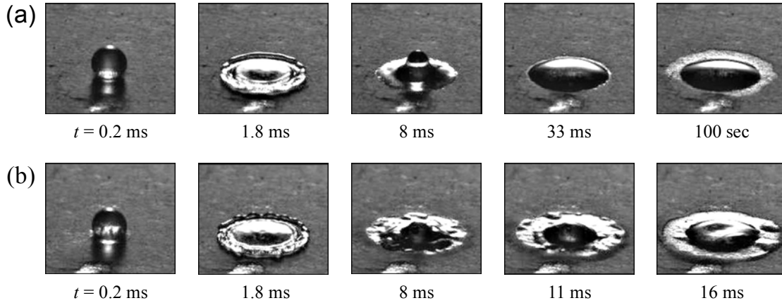
FIG. 11. Water drop impact on a PAN+CB nanofiber mat with thickness h=0.15 mm. The initial foil temperature is equal to (a) 80^{\circ}\text{C} and (b) 180^{\circ}\text{C} .
