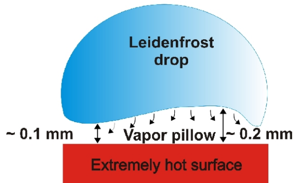
FIG 1. Leidenfrost effect: water droplet levitating on a vapor pillow above a very hot surface.
