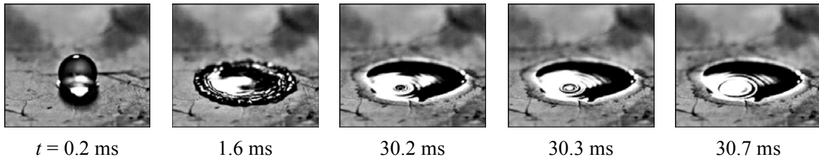
FIG. 12. Water drop impact onto a damaged PAN nanofiber mat with thickness h=1.5 mm. The initial foil temperature is equal to 220^{\circ} .
