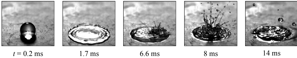
FIG. 13. Water drop impact onto a damaged PAN nanofiber mat with a thickness h=0.25 mm. The initial foil temperature is equal to 220^{\circ}\text{C} . This sequence of images illustrates the formation of a geyser.
