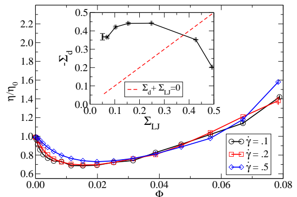
FIG. 1. (color online) Viscosity \eta vs. filling fraction \Phi for pushers for three strain rates \dot{\gamma} . \Phi = \frac{4}{3}\pi\sigma_{LJ}^3\rho , where \rho is the concentration, V_0 = 1 . Inset: Dipolar stress \Sigma_d vs LJ stress \Sigma_{LJ} ; \sigma_{LJ} = .35 , B_0 = 0.95 , and U_0 = -8\pi V_0 (pushers).
