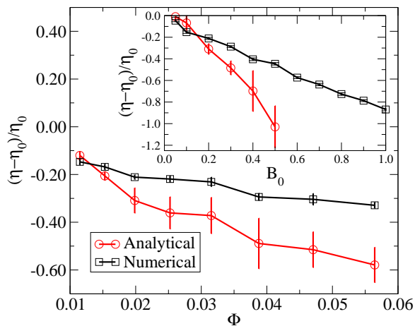
FIG. 4. (color online) \eta vs \Phi , B_0 = 0.2 , U_0 = -8\pi V_0 . Inset: Viscosity \eta vs. Bretherton constant B_0 for \Phi = .01986 . The error bars in the analytical results are due to uncertainty in the numerical calculation of the concentration variance.
