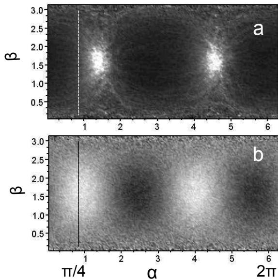
FIG. 3. P(\alpha, \beta) for \Phi = .0003 (a) and \Phi = .005 (b). Vertical lines indicate \alpha = \pi/4 ; V_0 = 1, \sigma_{LJ} = .35, U_0 = -8\pi V_0, B_0 = 0.95 . Maxima are shown in white, minima in black.
