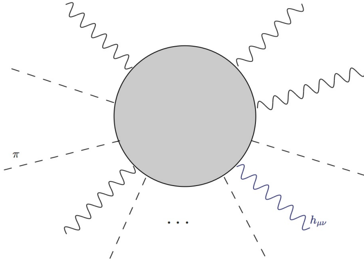
Figure 1: An arbitrary 1PI diagram with gravitational degrees of freedom in the loop.
