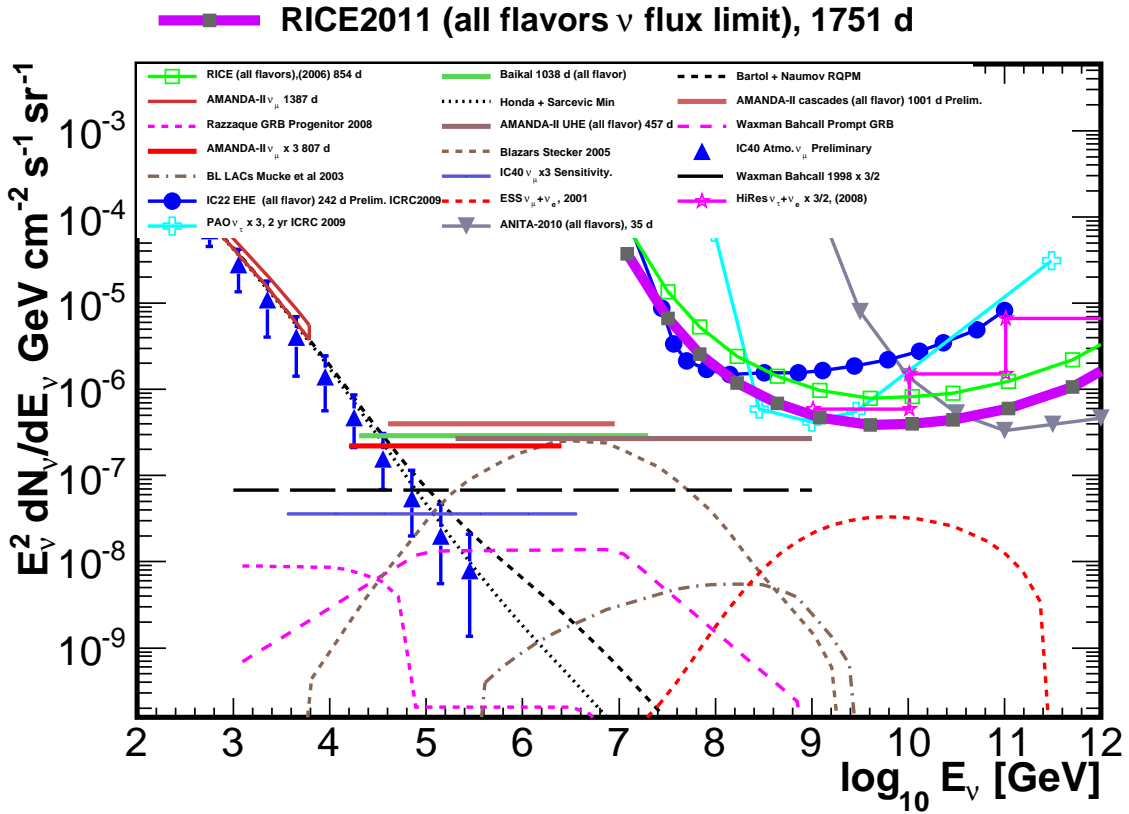
FIG. 15: Compilation of existing neutrino flux limits, including updates reported herein. Factors of 3 or 3/2 shown in the plot are needed to translate predictions and experiments sensitive to only one or two neutrino flavors to the three flavors of neutrinos to which the RICE experiment is sensitive. Model predictions shown are from calculations of the neutrino fluence from blazars by Stecker[37], BL LAc galaxies[38], GRB's[39], photonuclear production of neutrinos by cosmic-ray interactions with the Cosmic Microwave Background[40], models of neutrinos generated locally to Earth[41–44] and Active Galactic Nuclei fluence predictions[45]. Other presented experimental limits are those from AMANDA-II[46–49], the previous RICE result[2], the HiRes experiment[50], based on electron neutrinos only (and extrapolated to three flavors), ANITAI[51] and a result from the Auger experiment[52], based on tau neutrinos only (and extrapolated to three flavors). Models are shown as dashed or solid lines; experimental results as lines/points.
