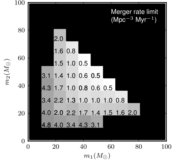
FIG. 2: The 90% confidence upper limit on the merger rate as a function of mass in units of M_\odot (symmetric over m_1 and m_2 ). This image represents the rate limit in units of \text{Mpc}^{-3} \text{Myr}^{-1} . These limits can be converted to traditional units of L_{10}^{-1} \text{Myr}^{-1} by dividing by 0.0198 L_{10} \text{Mpc}^{-3} [98]. Only bins with mass ratios < 4 : 1 have upper limits computed due to uncertainty in the waveform models for more asymmetric systems.
