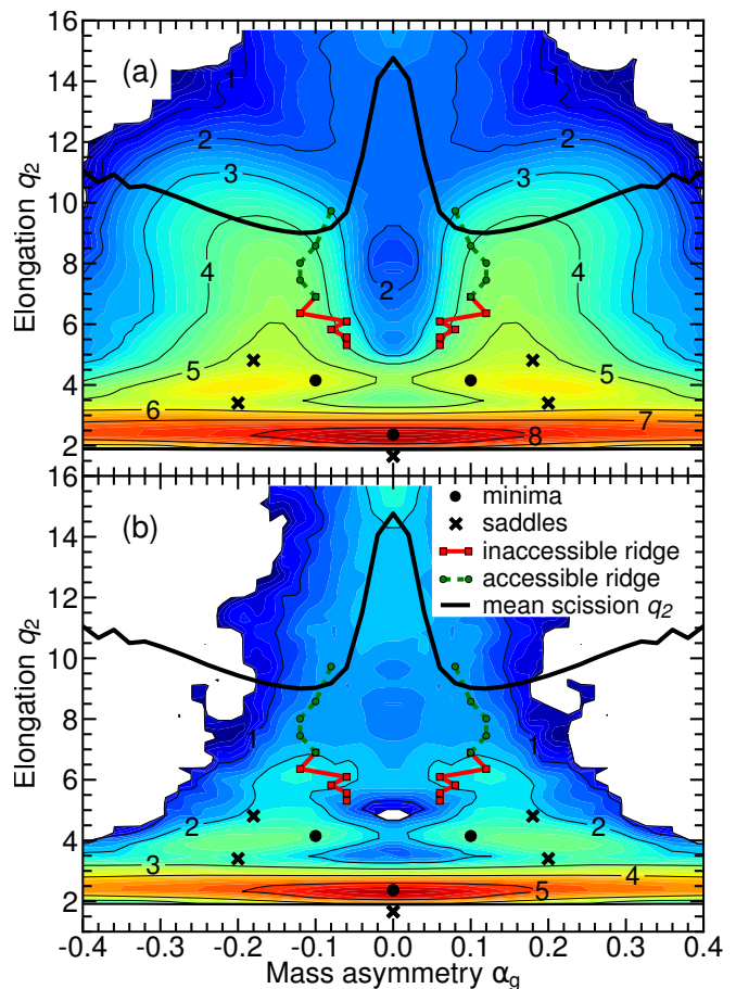
FIG. 3: (Color online) \log_{10} (number of visits) to grid points with a given combination of asymmetry \alpha_g and elongation q_2 for ^{236}\text{U} with E_{\text{exc}} = 6.55 MeV. (a) All tracks in the simulation. (b) The tracks ending in symmetric fission. Energy minima are shown as solid circles and saddle points as crosses. The solid black curve shows the mean “scission” elongation. The ridge separating symmetric from asymmetric fission paths is shown as a solid red (dark gray)/dashed green curve, where green/red indicates that the ridge is below/above the total energy, E_{\text{exc}} = 6.55 MeV, and thus accessible/inaccessible.
