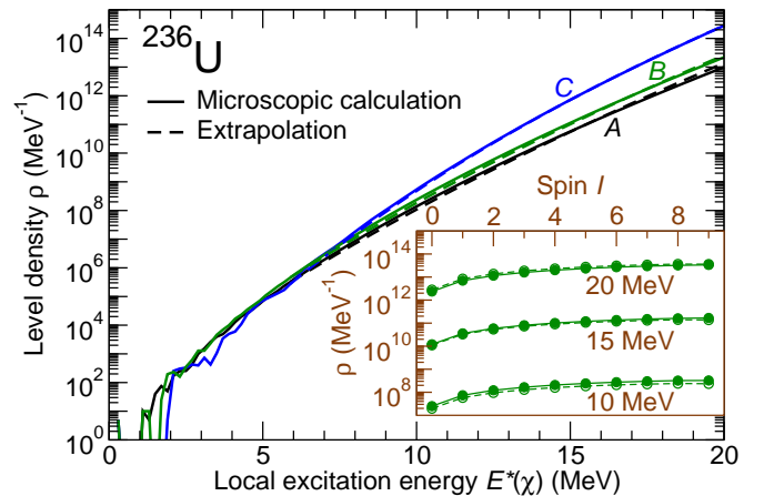
FIG. 2: (Color online) Microscopic level densities (solid lines) compared to extrapolated values (dashed lines). Three different deformations for ^{236}\text{U} are considered: A - the second minimum, B - the asymmetric second saddle, and C - an elongated symmetric shape close to the outer barrier. Extrapolated values are shown for local excitation energies E^*(\chi) \geq 6 MeV. The inset shows the angular momentum distribution of the level density at the asymmetric saddle ( B ) for different excitation energies.
