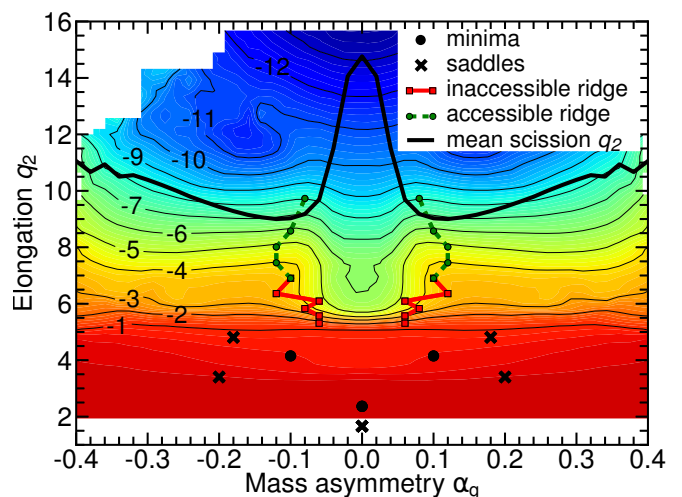
FIG. 6: (Color online) Logarithm of the ergodicity ratio, \log_{10}(r) , where r is given by Eq. (13), for ^{236}\text{U} with E_{\text{exc}} = 6.55 MeV.
