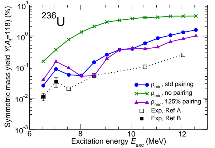
FIG. 12: (Color online) Mass yields (logarithmic scale) at symmetry for ^{236}\text{U} shown versus excitation energy. The calculated results (blue circles) are compared with experimental data from Ref. A (open squares) [25], and B (filled squares) [22]. Results of two additional calculations are also shown, one where the level densities are obtained without pairing (green crosses) and one where the pairing strength is increased by 25% (triangles). The potential-energy surface used in the three calculations is the same, consistent with standard pairing.
