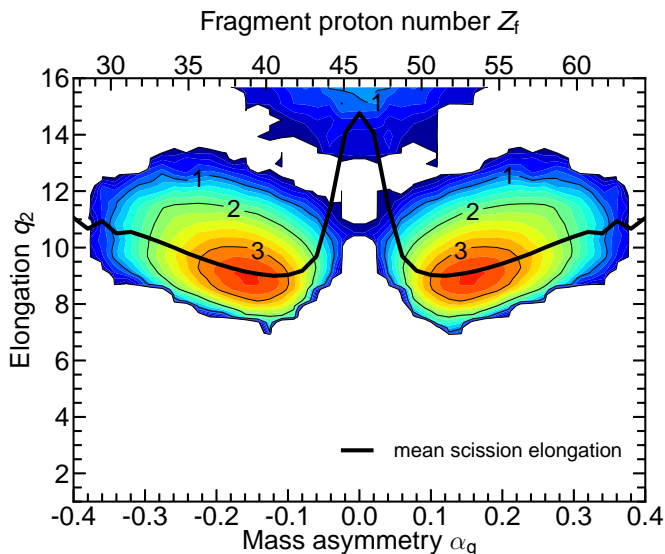
FIG. 5: (Color online) Contour plot (on a logarithmic scale) of the location of the end points projected onto the (\alpha_g, q_2) plane for fission of ^{236}\text{U} at E_{\text{exc}} = 6.55 MeV. Fragment proton numbers (shown on the upper axis) are obtained as Z_f = 46(1 + \alpha_g) .
