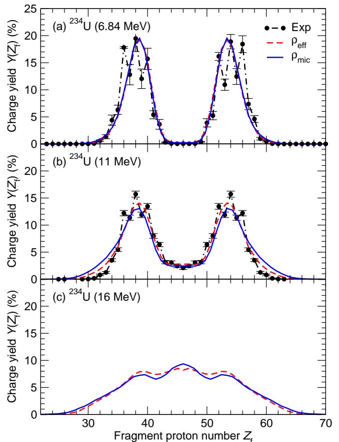
FIG. 8: (Color online) Fission-fragment charge yields for ^{234}\text{U} at three different excitation energies, (a) E_{\text{exc}} = 6.84 MeV, (b) 11 MeV and (c) 16 MeV. The blue solid curves have been obtained with the microscopic level densities, while the dashed red curves were calculated with the effective level density \rho_{\text{eff}} introduced in Ref. [2]. The results for E_{\text{exc}} = 6.84 MeV are compared to (n_{\text{th}}, f) data [22], while those for E_{\text{exc}} = 11 MeV are compared to (\gamma, f) data [23].
