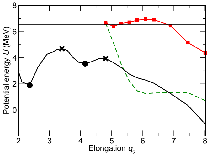
FIG. 4: (Color online) Potential-energy curves for ^{236}\text{U} versus elongation, q_2 . The energy path leading to asymmetric fission, starting close to the (symmetric) second minimum, is shown by a solid line. The valley leading to symmetric fission (dashed line) is separated from the asymmetric path by the ridge shown by the red (dark gray) line. The thin horizontal line indicates the excitation energy E_{\text{exc}}=6.55 MeV.
