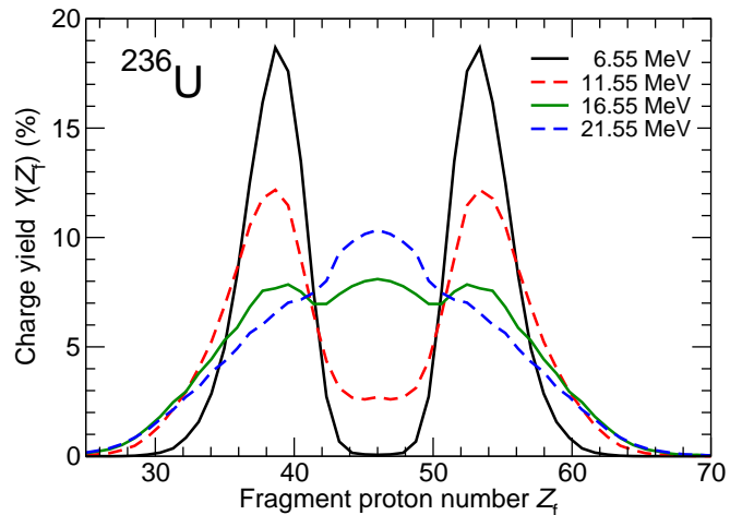
FIG. 10: (Color online) Calculated charge yields for fission of the nucleus ^{236}\text{U} at four values of the excitation energy: from E_{\text{exc}} = 6.55 \text{ MeV} ( = S_n , the neutron separation energy) up to 21.55 MeV in steps of 5 MeV.
