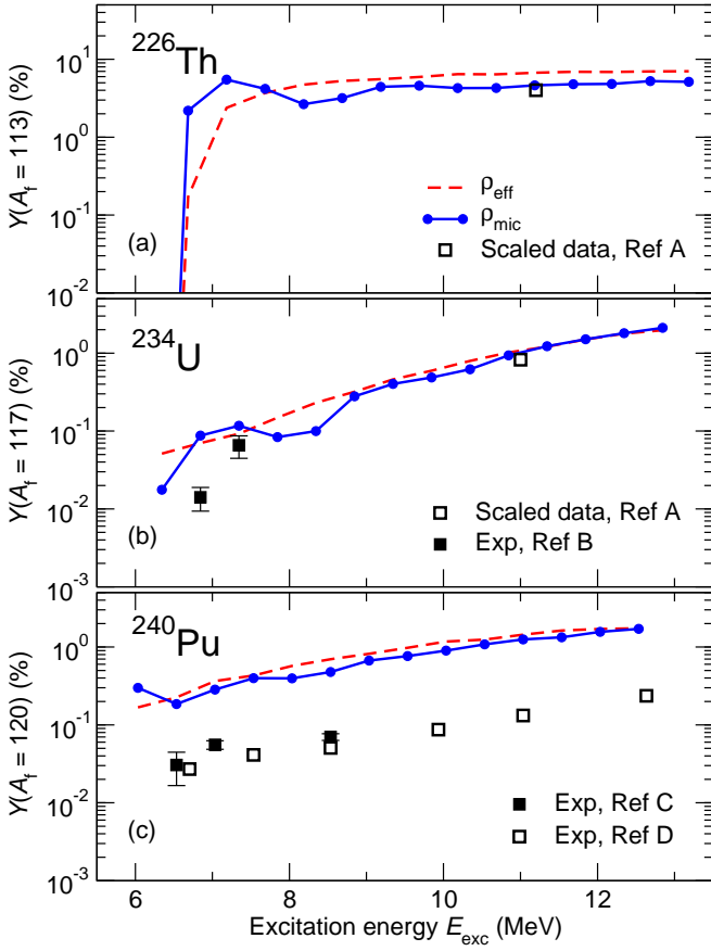
FIG. 11: (Color online) Symmetric mass yields versus excitation energy for (a) ^{226}\text{Th} , (b) ^{234}\text{U} and (c) ^{240}\text{Pu} . The calculated yields are obtained with \rho_{\text{mic}} (blue circles) or \rho_{\text{eff}} as in Ref. [2] (dashed red curve). The squares show various experimental data from Refs. [23] (A), [22] (B), [22] (C), and [24] (D); the charge yield from Ref. [23] have been multiplied by Z/A .
