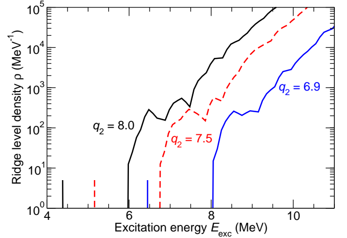
FIG. 13: (Color online) Level densities at the first three accessible points along the ridge separating the asymmetric and symmetric valleys.
