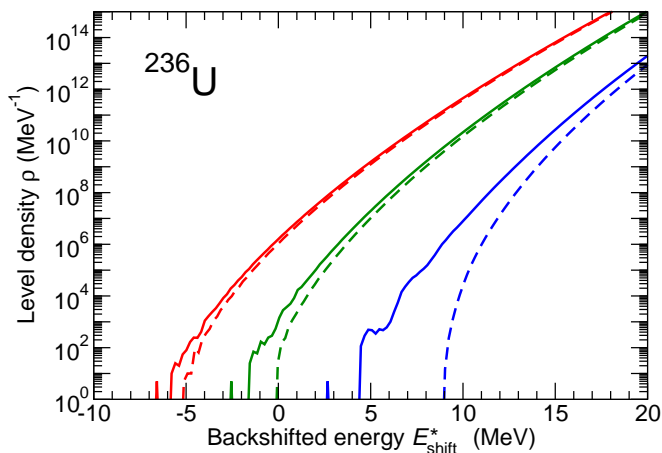
FIG. 1: (Color online) The microscopic level density, \rho(E^*) , calculated for ^{236}\text{U} at angular momentum I = 4\hbar and plotted versus the backshifted energy, E_{\text{shift}}^* = E^* + E_{\text{sh}} + E_{\text{pc}} , shown for three selected shapes: (i) the second minimum (red/left) ( E_{\text{sh}} = -5.4 MeV, E_{\text{pc}} = -1.5 MeV), (ii) the outer symmetric fission barrier (blue/right) ( E_{\text{sh}} = +8.7 MeV, E_{\text{pc}} = -6.1 MeV), and (iii) a shape in between (green/middle) ( E_{\text{sh}} = -0.3 MeV, E_{\text{pc}} = -2.5 MeV), either with (solid) or without (dashed) pairing.
