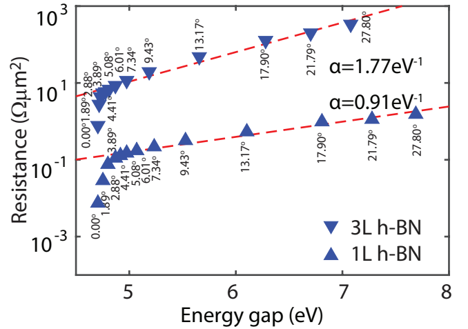
FIG. 3. Zero temperature coherent resistance of graphene/1L h-BN/graphene (upward-pointing triangles) and graphene/3L h-BN/graphene (downward-pointing triangles) as a function of the effective energy gap of the monolayer h-BN and 3 layer h-BN at the K -point of the graphene. The angles are given next to each data point. The red lines show exponential fits to the data, R = R_0 e^{\alpha E_G} . The values of \alpha are shown next to the fitted line. E_F = 0.26 eV.
