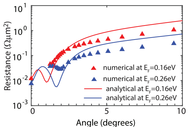
FIG. 4. Zero temperature coherent resistance of Gr/1L h-BN/Gr as a function of rotation angle for Fermi energies equal to 0.26eV (blue) and 0.16eV (red). The solid lines show the result calculated from the continuum model, and the triangles show the results from the tight-binding, NEGF calculation. The smallest commensurate rotation angle calculated numerically is 1.25^\circ .
