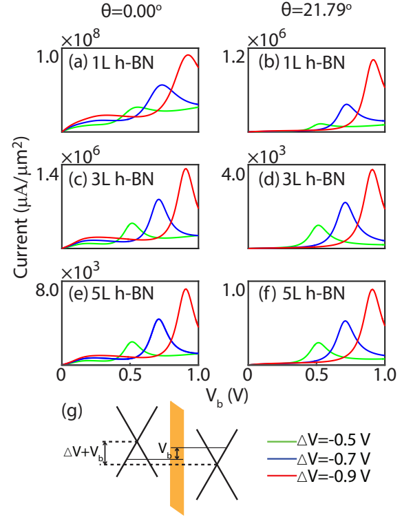
FIG. 7. Current as a function of bias voltage for different potential differences \Delta V between the two graphene layers. (a) Graphene/1L h-BN/graphene with no rotation; (b) graphene/1L h-BN/graphene with a 21.79^\circ rotation angle; (c) graphene/3L h-BN/graphene with no rotation; (d) graphene/3layer h-BN/graphene with a 21.79^\circ rotation angle; (e) graphene/5L h-BN/graphene with no rotation; (f) graphene/5layer h-BN/graphene with a 21.79^\circ rotation angle. (g) Schematic diagram of the structure with bias voltage V_b and built-in potential \Delta V .
