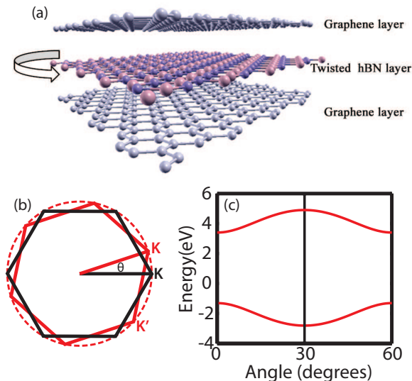
FIG. 1. (a) Atomistic geometry of the graphene/boron-nitride/graphene heterostructure. The top and bottom layers are aligned graphene. The middle boron-nitride layer is rotated with respect to the graphene layers. (b) In k space. The relative rotation between the Brillouin zone of h-BN (red) with respect to that of graphene (black). (c) The energy gap of monolayer h-BN at the K point of graphene as a function of rotation angle.
