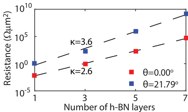
FIG. 10. Resistance versus number of h-BN layers for rotation angles of 0.00^\circ and 21.79^\circ at a Fermi energy of E_F = 0.26\text{eV} . The dash lines show the exponential fits R = R_0 e^{\kappa \cdot n} where n is the number of BN layers. The decay constants \kappa are shown next to the fits for the two structures.
