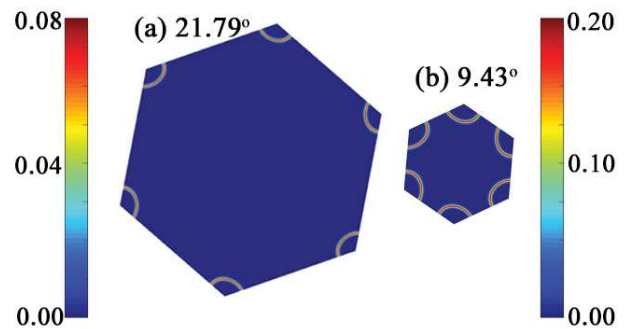
FIG. 9. Transmission coefficient T(E, \mathbf{k}) in the first Brillouin zone at energy of 0.5 eV for Graphene/1L h-BN/Graphene heterostructure with rotation angle: (a) 21.79^\circ (b) 9.43^\circ
