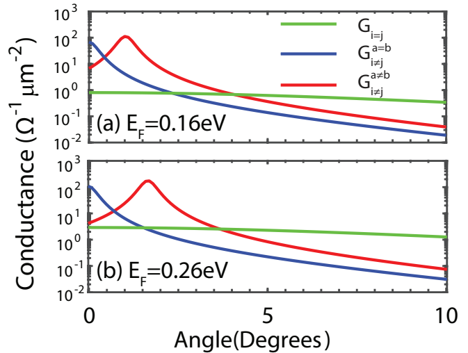
FIG. 5. Conductance components as a function of rotation angle for (a) E_F = 0.16\text{eV} , (b) E_F = 0.26\text{eV} .
