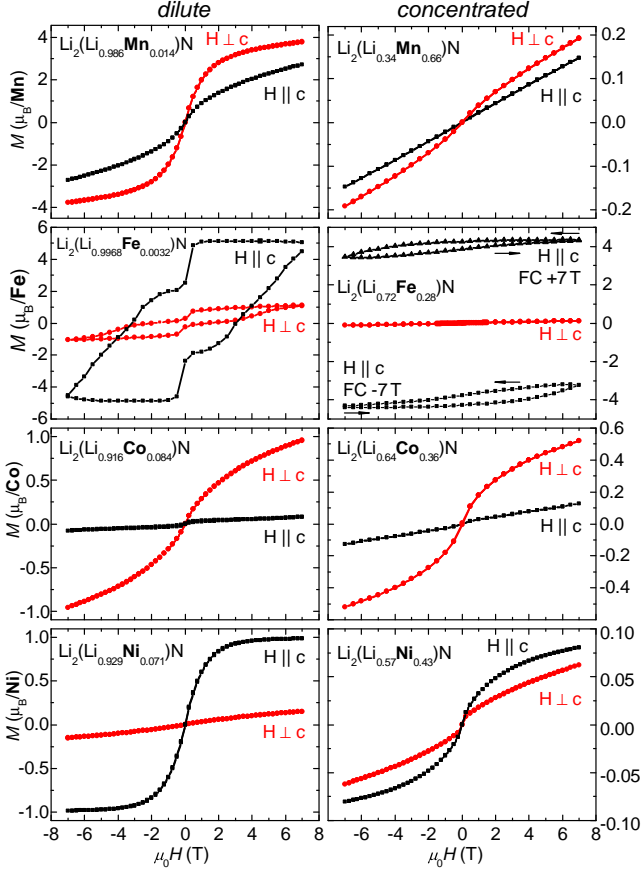
FIG. 1. (color online) Isothermal magnetization loops at T = 2\text{K} in Bohr magnetons per transition metal ion (FC \pm 7\text{T} refers to a field cooled measurement in +7\text{T} and -7\text{T} , respectively). The sign of the magnetic anisotropy changes in an alternating fashion from easy plane to easy axis independent from the concentration of the transition metal.
