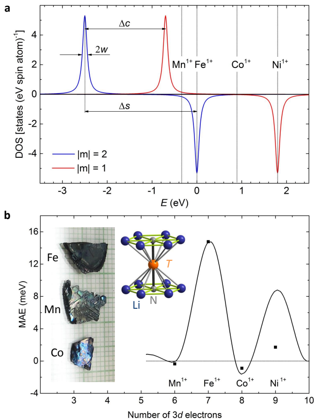
FIG. 3. (color online) a) Schematic density of states projected on the 3d states of isolated Fe atoms. The MAE in the analytical model is determined by crystal field splitting ( \Delta c ), spin splitting ( \Delta s ), and peak width ( w ). For T = \text{Mn}, \text{Co}, and \text{Ni} the position of the Fermi level is shifted according to the number of 3d electrons (rigid band approximation). b) The magnetic anisotropy energy (MAE) per isolated T atom as a function of the number of 3d electrons calculated in the analytical single-ion model is shown by the solid line. The MAE calculated by LSDA is shown for comparison (black squares). Inset are three single crystals on a millimeter grid and the local crystal structure of the transition metal with nearest and next-nearest neighbors.
