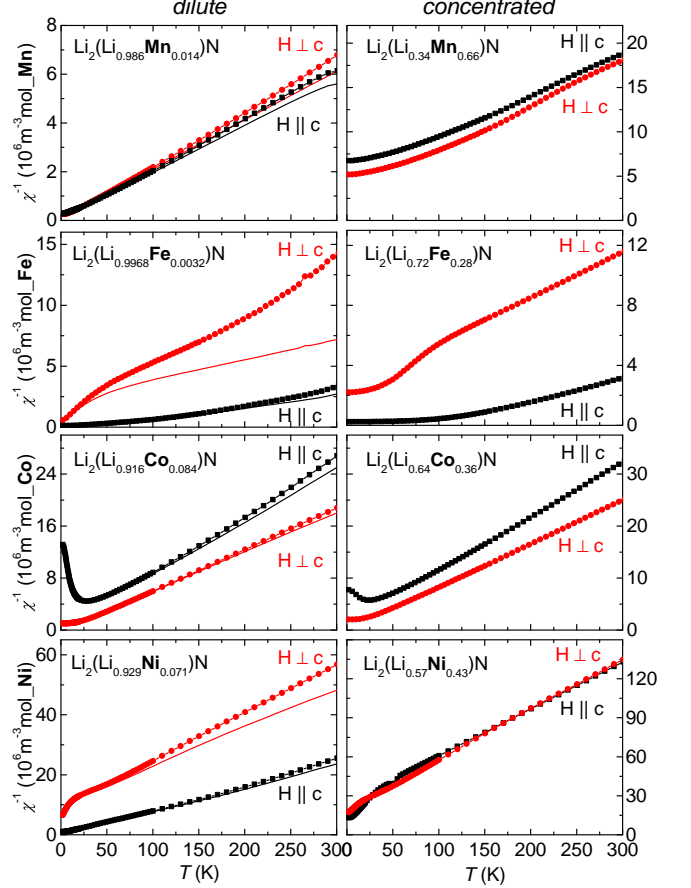
FIG. 2. (color online) Inverse magnetic susceptibility per mol transition metal as a function of temperature ( \chi^{-1} = H/M , \mu_0 H = 7\text{T} ). A pronounced magnetic anisotropy is observed over the whole temperature range except for T = \text{Mn} and concentrated, T = \text{Ni} \text{Li}_2(\text{Li}_{1-x}\text{T}_x)\text{N} . The solid lines given for the dilute case (left panel) show the inverse susceptibility after subtracting the core diamagnetism of \text{Li}_3\text{N} .
