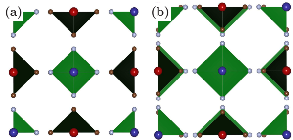
FIG. 1. (Color online) Similar to the Prussian blue family of mixed-metal poly-cyanides, the CoFe-PBA exhibits a face-centered cubic (fcc) structure comprising a three-dimensional network of \text{CoN}_6 (green) and \text{FeC}_6 (black) octahedra. The major structural difference between the (a) low-spin and (b) high-spin states lies in the Co-N bond length, which is \sim 0.21 Å longer in the high-spin state (Table I). Atomic elements are shaded as follows: Co (blue), Fe (red); N (gray); and C (brown). Alkali metal cations ( \text{K}^+ ) occupy the tetrahedral sites of the fcc structure, and are not shown for clarity.
