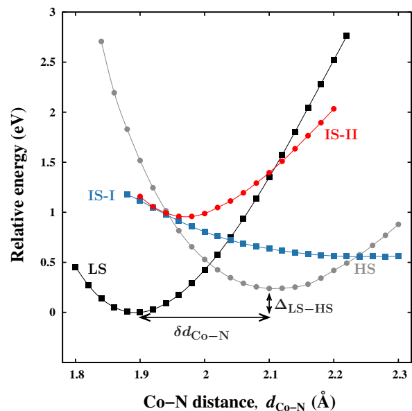
FIG. 3. (Color online) Electronic transitions are strongly coupled with the structural relaxations of the CoN 6 -octahedra. The CoN 6 octahedra of the PBA crystal are elongated along the Co-N ligands by a distance \delta d_{Co-N} in the high-spin state. Thus, we calculate the relative free energy ( E - E_{LS} ) at varying d_{Co-N} for different spin states. The forward and reverse spin transitions are both mediated via intermediate states.
