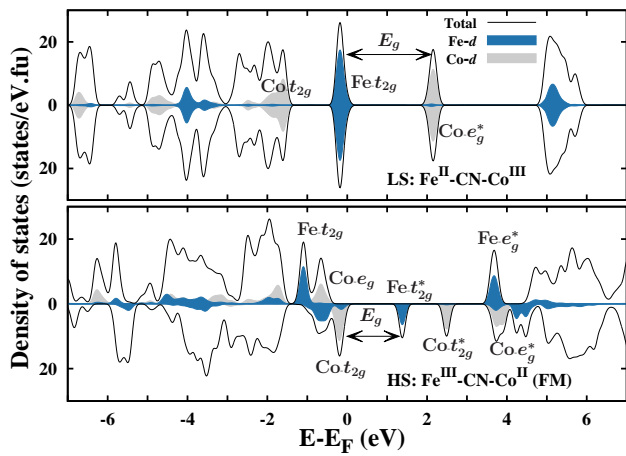
FIG. 2. (Color online) Density of states in forward and reverse spin transitions indicates metal-to-metal charge transfer. The valence band of the low-spin (high-spin) state is composed with the Fe- t_{2g} (Co- t_{2g} ) states, whereas the conduction band is composed with the Co- e_g (Fe- t_{2g} ) states. Calculated charge transfer excitations agree with the experimental absorption spectra. 1,2,30
