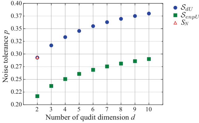
FIG. 5. Noise tolerance of steering conditions (7) and (9). If the probability of white noise p_{\text{noise}} < p , then the single-system steering, that underlies the qudits sent by Alice with the states \rho_i(a_i, p_{\text{noise}}) , can be certified by the steering conditions (7) or (9). Here the threshold of noise intensity p is an indicator showing the noise tolerance of these steering criteria. Note that the noise tolerance of the certification based on violating the EPR steering inequality, i.e., S_N > 1 , implemented with two measurement settings ( N = 2 ) is the same as that of the steering condition (7) for two-dimensional systems (the EPR steering inequality introduced by Smith et al. [7] is applicable to d = 2 only). For large d , both the conditions (7) and (9) are robust against noise up to p = 50\% .
