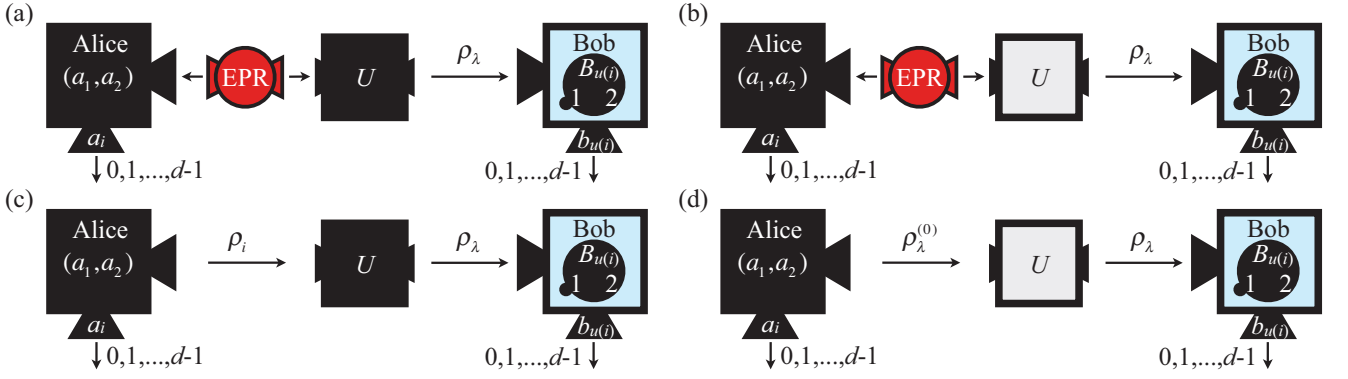
FIG. 4. Mimicries of EPR steering where the EPR source is qualified but the measurement device of Alice is not. (a) the unqualified operation is used, and (b) the operation used is qualified in the mimicry. These two possible situations can be described by the two realism conditions and represented in practical descriptions (c) and (d), respectively. The demonstration (c) has the analogue of single-system steering described by Fig. 2(e). The concrete mimicry (d) is equivalent to that of single-system steering depicted in Fig. 3(c).
