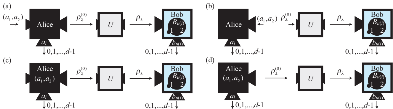
FIG. 3. Steering mimics where the operation U is qualified but the measurement device of Alice is not. The classical mimics of single-system steering (a) and EPR steering (b) are based on the realistic assumptions that (1) the state of the particle sent by Alice can be described by a fixed set (a_1, a_2) , and (2) the state can change from (a_1, a_2) to another state \lambda which corresponds to a quantum state of the qudit \rho_\lambda finally held by Bob. One can concretely represent these scenarios in the practical descriptions of unqualified Alice's apparatus (c) and (d), respectively. These concrete simulations are then shown to be equivalent.
