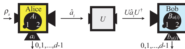
FIG. 1. Single-system steering for quantum information tasks. The state \hat{a}_i is sent from Alice to Bob. Here \hat{a}_i is a post-measurement state of a qudit \rho_s under the measurement A_i for i = 1, 2 . By sharing certain information distributed via a classical communication channel (not shown), Alice can steer the state of Bob's particle by asking him to perform the quantum operation U . For example, by simply choosing U as an identity operator, Alice's steering enables them to realize QKD. When U is an arbitrary quantum logic gate, steering single systems is equivalent to performing quantum computation. To identify whether Alice can implement such steering, Bob can use the steering condition (7) or (9) to rule out the results mimicked by generic classical strategies. As illustrated, Bob performs measurements B_{u(i)} to implement these certifications. These steering conditions ensure secure quantum communication and faithful quantum computation (see table I). Here, it is allowed that Alice and Bob have no spatial separation but access the single system at different times.
