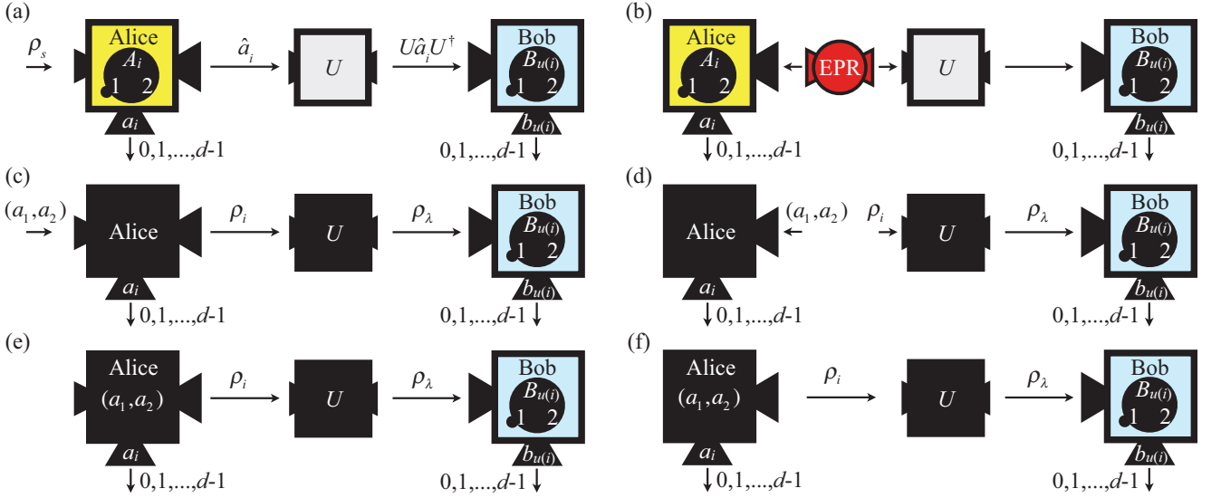
FIG. 2. Comparison between single-system steering and EPR steering. We compare these two scenarios by, first, their basic concepts of ideal single-system steering (a) and ideal EPR steering (b), and, second, classical mimics of single-system steering (c), (e) and EPR steering (d), (f). For the ideal case, Alice can use the effect of EPR steering, by sharing the entangled states (EPR source), to implement the operation U on the state of Bob’s qudit, U\hat{a}_iU^\dagger , for both quantum steering scenarios. To distinguish classical mimicry from genuine quantum steering, the respective classical models based on realistic theories (c) and (d) are introduced. These “classical simulations” can be concretely represented in the practical descriptions of, for example, unqualified measurements of Alice and the unqualified operation U performed by Alice or Bob [(e) and (f)]. As shown in (e) and (f), these effective simulations are equivalent.
