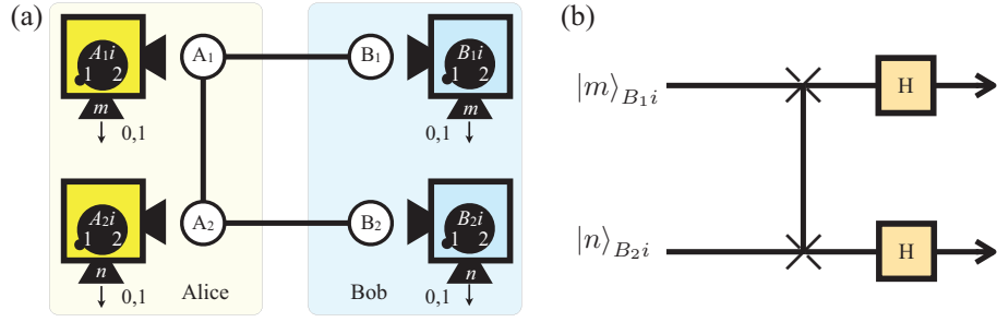
FIG. 6. EPR steering for one-way quantum computing. (a) A genuine four-qubit chain-type cluster state shared by Alice and Bob is represented by a fully-connected horseshoe graph. Alice, who performs the measurements A_{1i} and A_{2i} for i = 1, 2 on her qubits A_1 and A_2 , respectively, can reveal the EPR steering effect to realize the gate operation U on the qubits of Bob B_1 and B_2 . (b) The state |m\rangle_{B_{1i}} \otimes |n\rangle_{B_{2i}} is an input of the quantum gate U composed of one two-qubit CPHASE gate and two single-qubit Hadamard operations. For one-way quantum computing, the outcomes of Alice's measurements, m and n , corresponding to the post measurement state |m\rangle_{A_{1i}} \otimes |n\rangle_{A_{2i}} , determines the output state of the gate operation, U(|m\rangle_{B_{1i}} \otimes |n\rangle_{B_{2i}}) .
